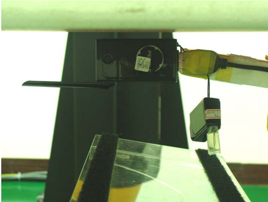
USB Configuration 3 with 5 mm separation (Ant. set 180 degree)
