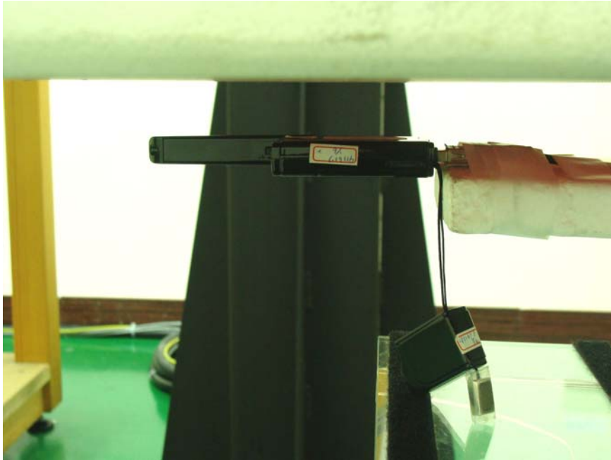
USB Configuration 2 with 20 mm separation for Back-Off SAR (Ant. set 180 degree)
