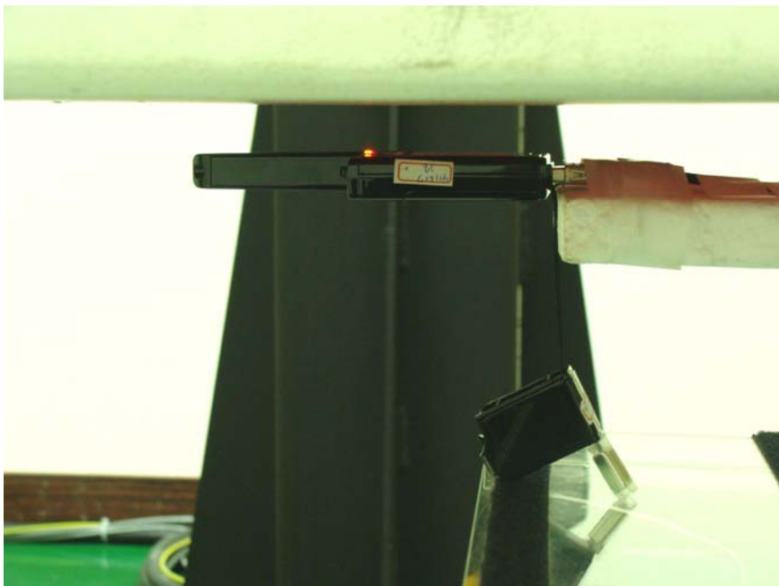
USB Configuration 2 with 15 mm separation for Back-Off SAR (Ant. set 180 degree)
