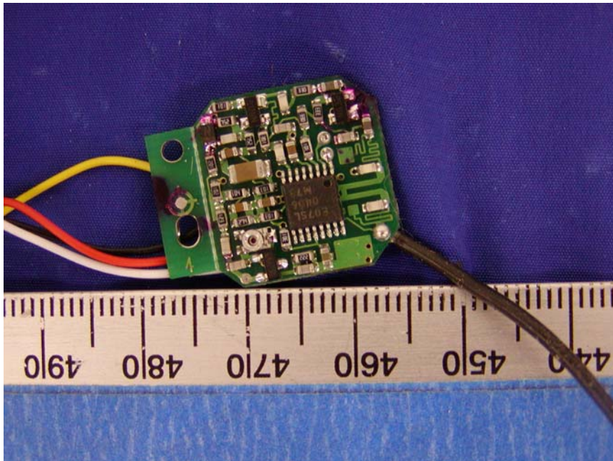
EUT – Antenna Top View
