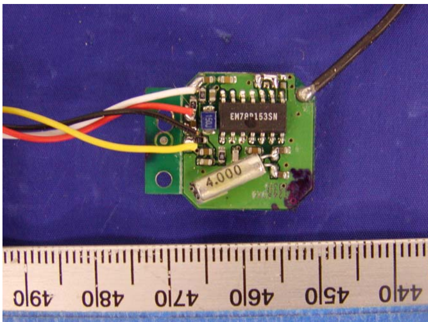
EUT – Antenna Bottom View
