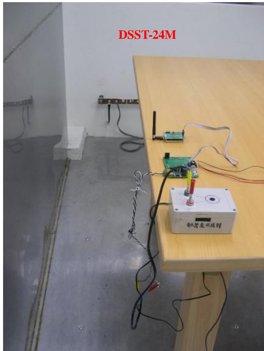
Photo 2: Conducted Emission Test Set-up
