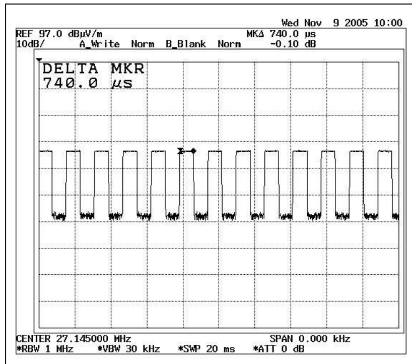
Duty Cycle 3
