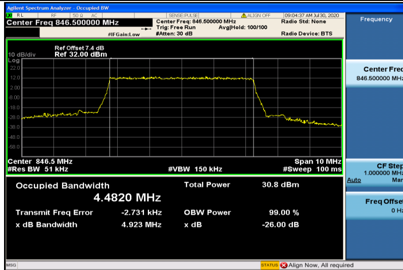
Band5-5MHz-QPSK-20625-25RB#0-4.4820
