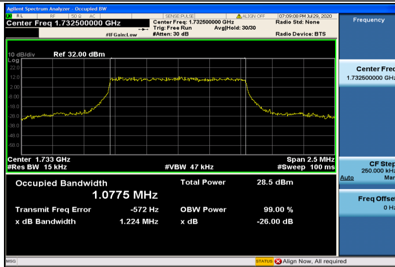
Band4-1.4MHz-16QAM-20175-6RB#0-1.0775
