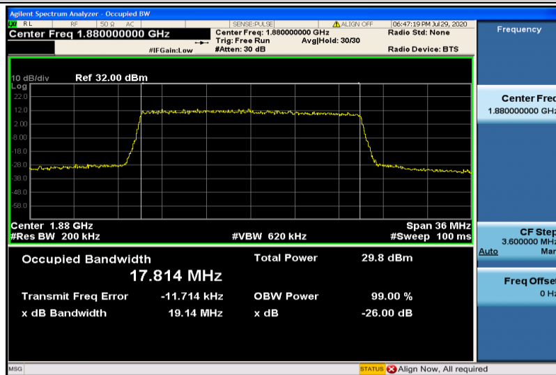
Band2-20MHz-16QAM-18900-100RB#0-17.814
