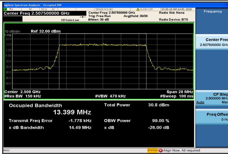
Band7-15MHz-QPSK-20825-75RB#0-13.399
