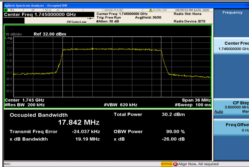
Band4-20MHz-16QAM-20300-100RB#0-17.842
