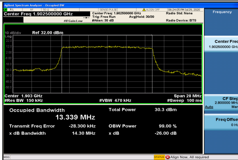
Band2-15MHz-QPSK-19125-75RB#0-13.339
