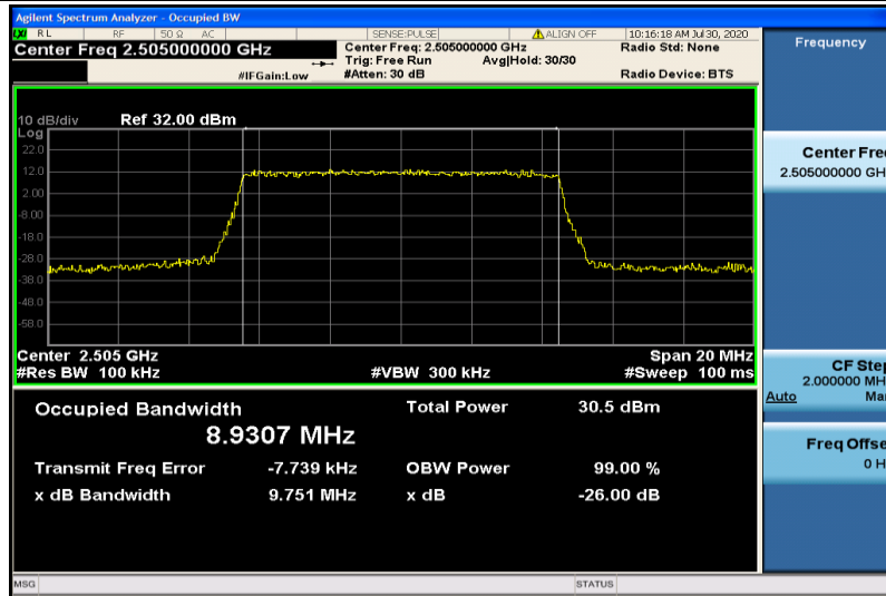
Band7-10MHz-QPSK-20800-50RB#0-8.9307
