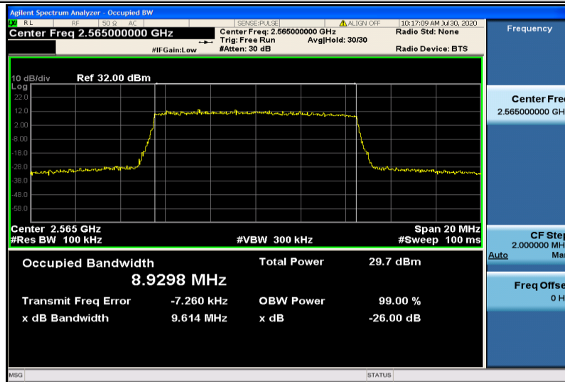
Band7-10MHz-16QAM-21400-50RB#0-8.9298
