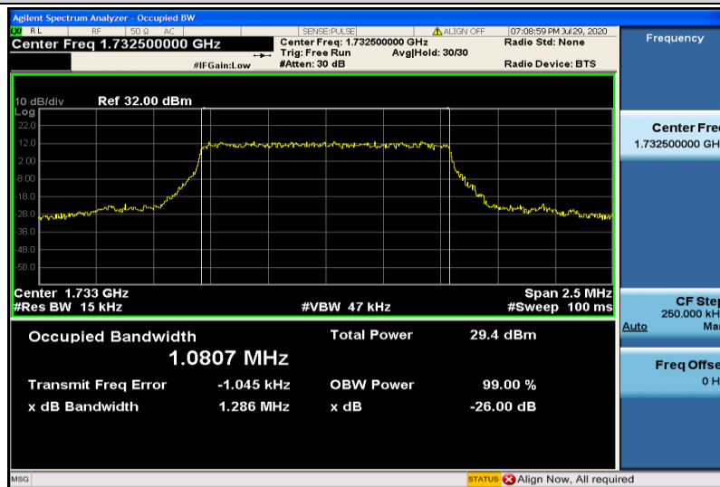
Band4-1.4MHz-QPSK-20175-6RB#0-1.0807
