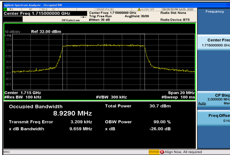
Band4-10MHz-QPSK-20000-50RB#0-8.9290
