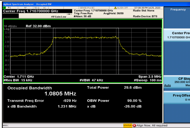
Band4-1.4MHz-QPSK-19957-6RB#0-1.0805
