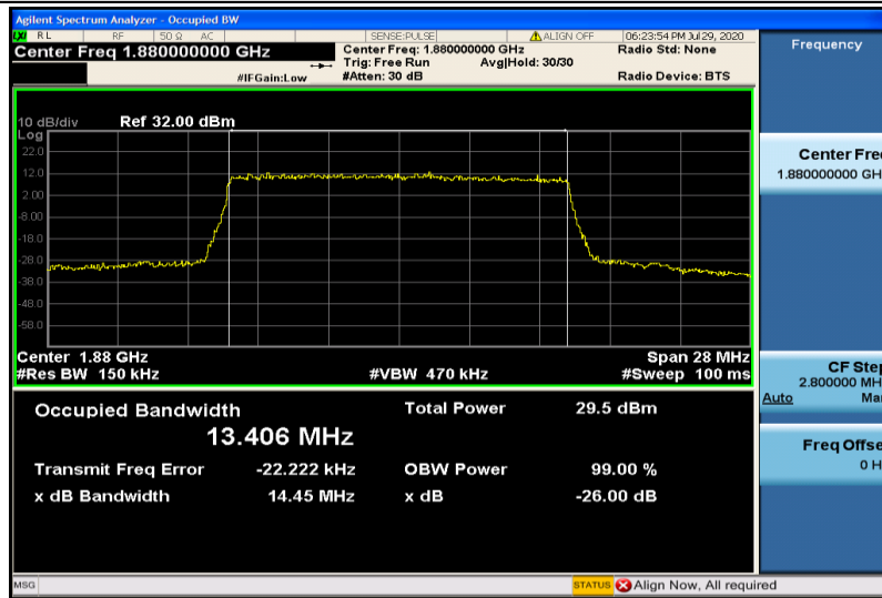
Band2-15MHz-16QAM-18900-75RB#0-13.406
