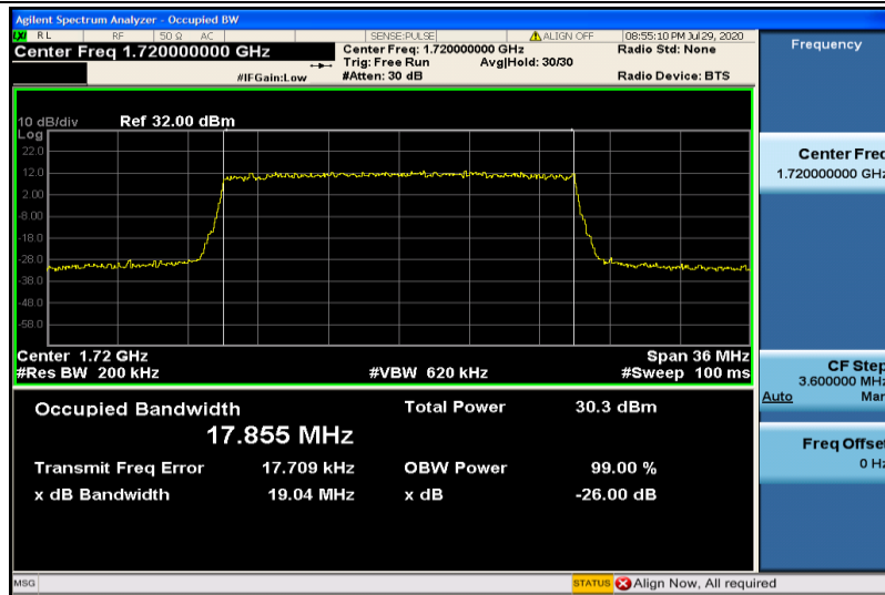
Band4-20MHz-16QAM-20050-100RB#0-17.855
