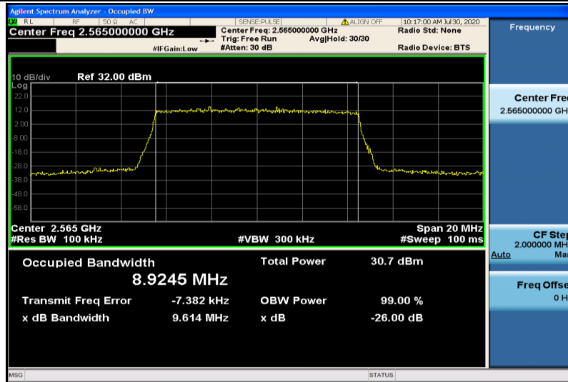
Band7-10MHz-QPSK-21400-50RB#0-8.9245
