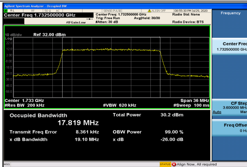
Band4-20MHz-16QAM-20175-100RB#0-17.819
