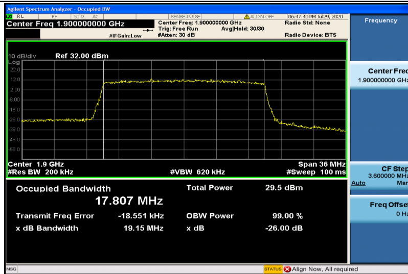
Band2-20MHz-16QAM-19100-100RB#0-17.807
