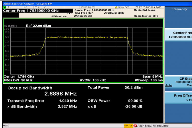
Band4-3MHz-QPSK-1753500000 GHz
