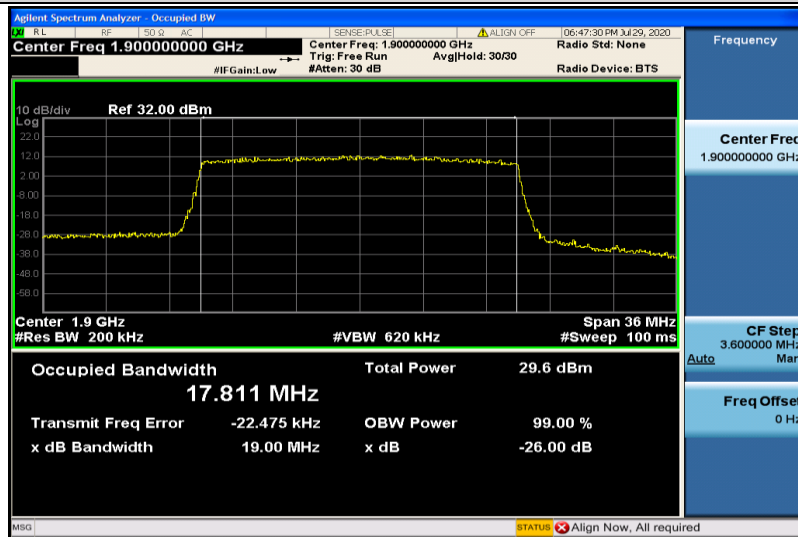
Band2-20MHz-QPSK-19100-100RB#0-17.811
