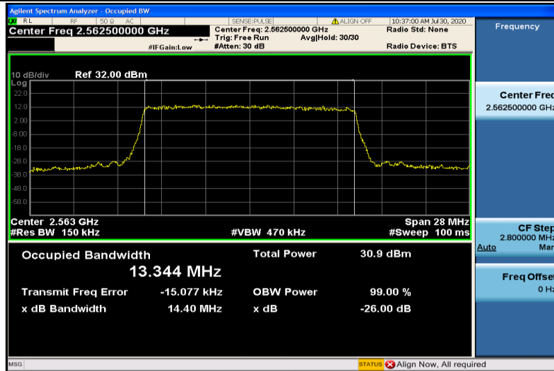
Band7-15MHz-QPSK-21375-75RB#0-13.344
