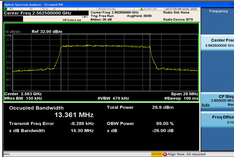
Band7-15MHz-16QAM-21375-75RB#0-13.361
