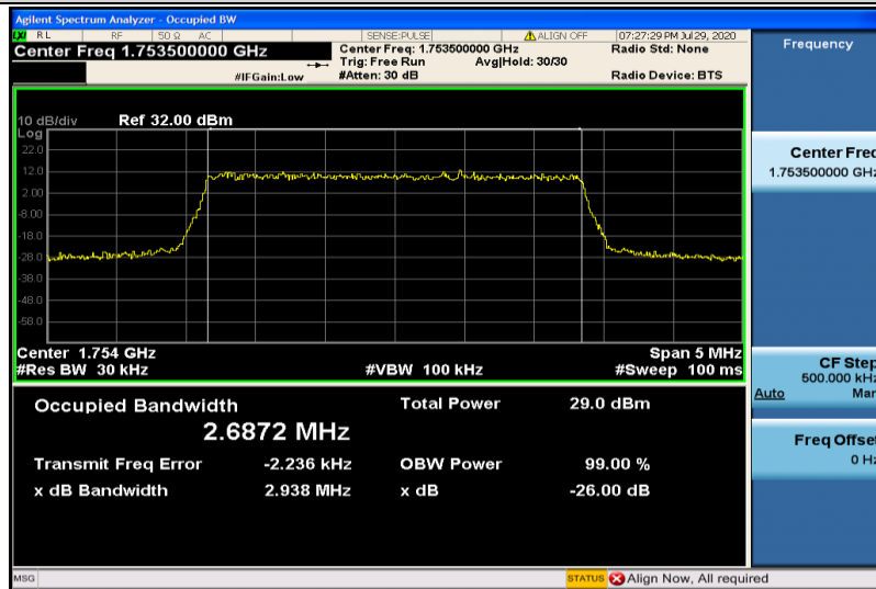
Band4-3MHz-16QAM-20385-15RB#0-2.6872
