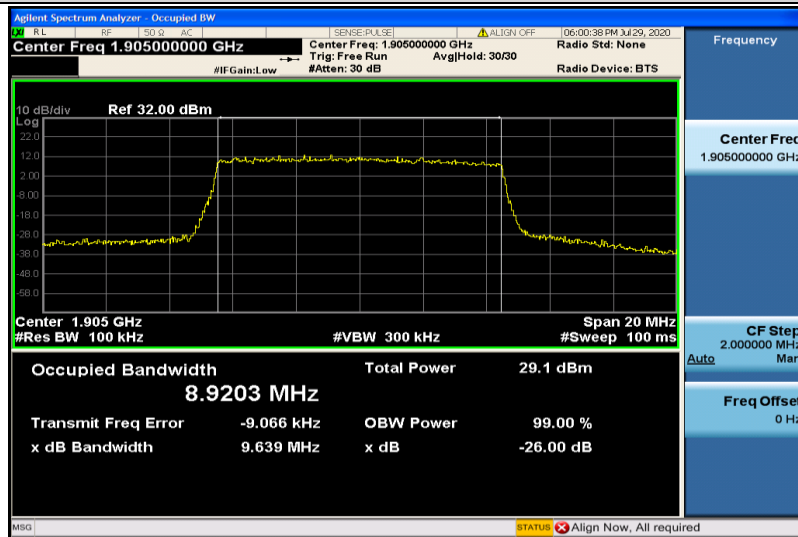
Band2-10MHz-16QAM-19150-50RB#0-8.9203
