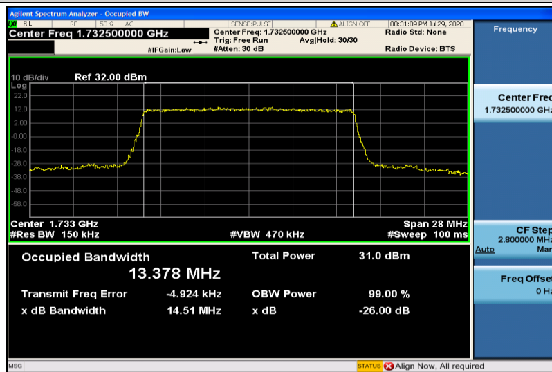
Band4-15MHz-QPSK-20175-75RB#0-13.378
