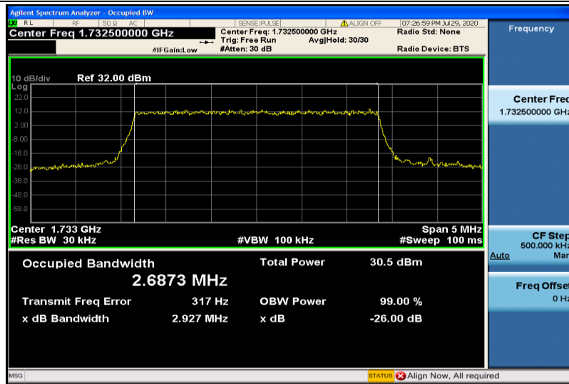
Band4-3MHz-QPSK-1732500000 GHz
