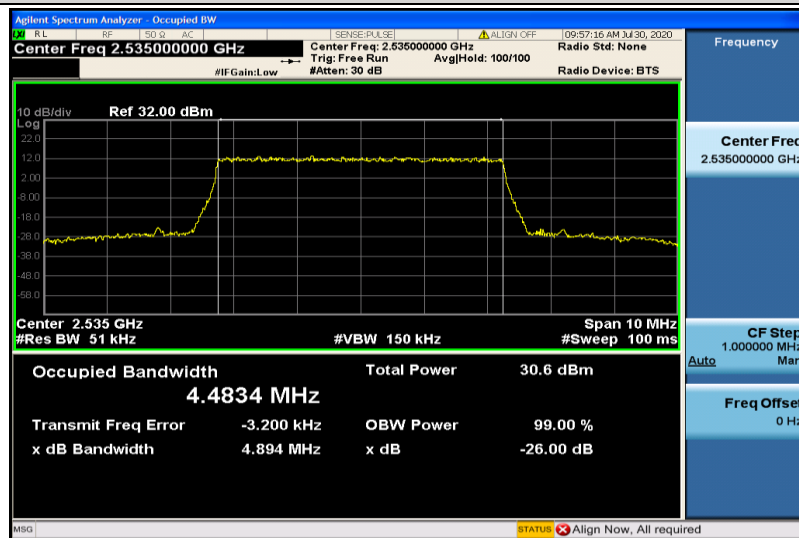
Band7-5MHz-QPSK-21100-25RB#0-4.4834
