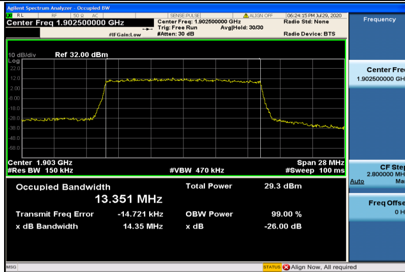
Band2-15MHz-16QAM-19125-75RB#0-13.351
