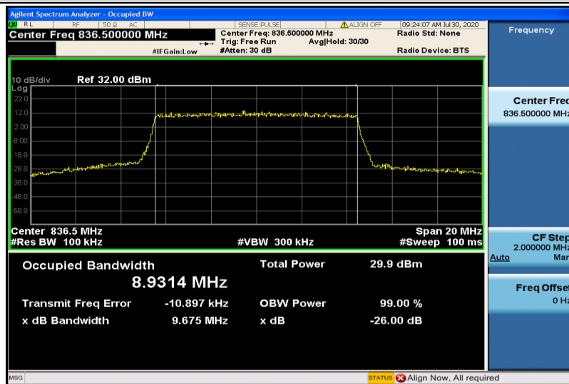
Band5-10MHz-16QAM-20525-50RB#0-8.9314
