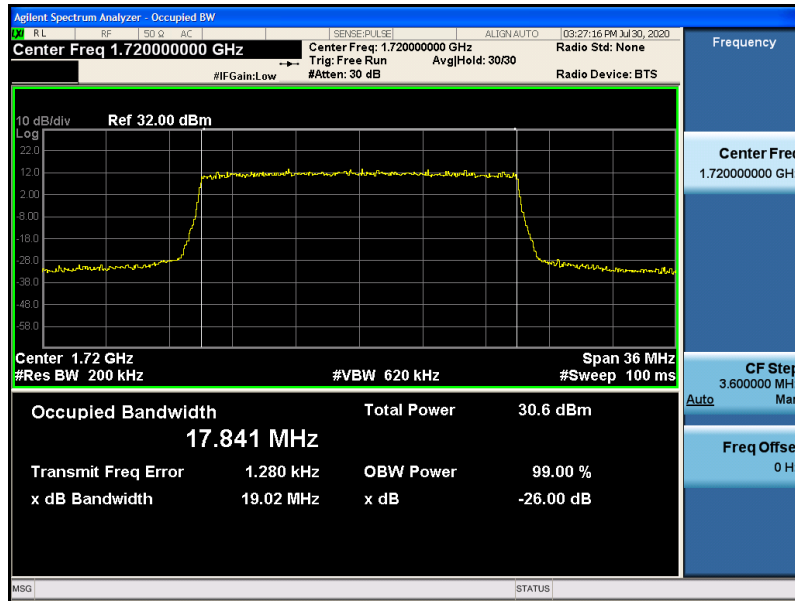
Band4-20MHz-QPSK-20050-100RB#0-17.841
