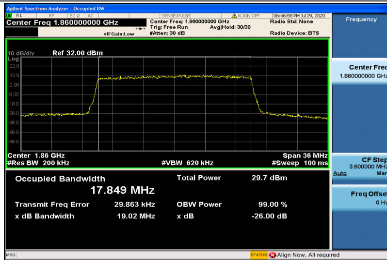
Band2-20MHz-16QAM-18700-100RB#0-17.849
