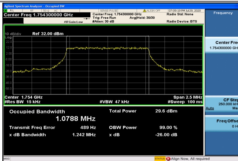
Band4-1.4MHz-QPSK-20393-6RB#0-1.0788
