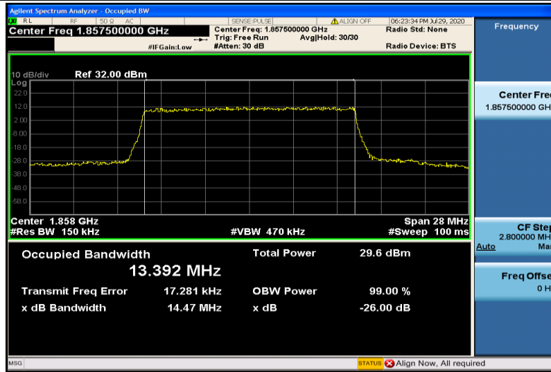
Band2-15MHz-16QAM-18675-75RB#0-13.392
