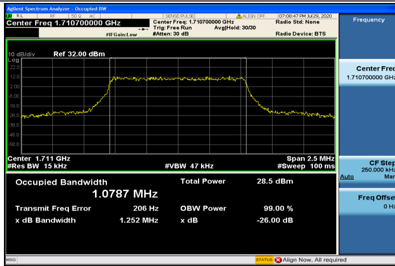
Band4-1.4MHz-16QAM-19957-6RB#0-1.0787
