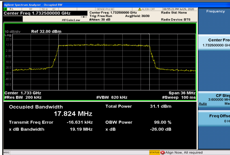
Band4-20MHz-QPSK-20175-100RB#0-17.824
