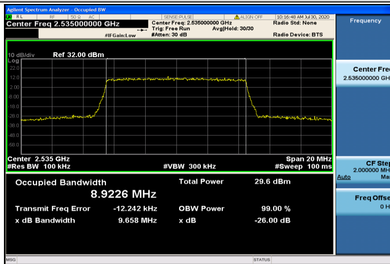
Band7-10MHz-16QAM-21100-50RB#0-8.9226
