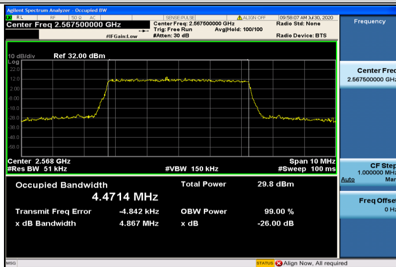
Band7-5MHz-16QAM-21425-25RB#0-4.4714
