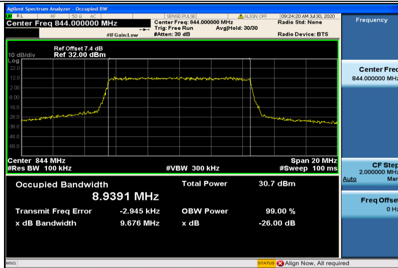
Band5-10MHz-QPSK-20600-50RB#0-8.9391
