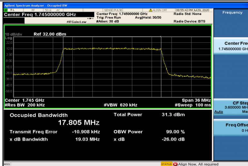
Band4-20MHz-QPSK-20300-100RB#0-17.805
