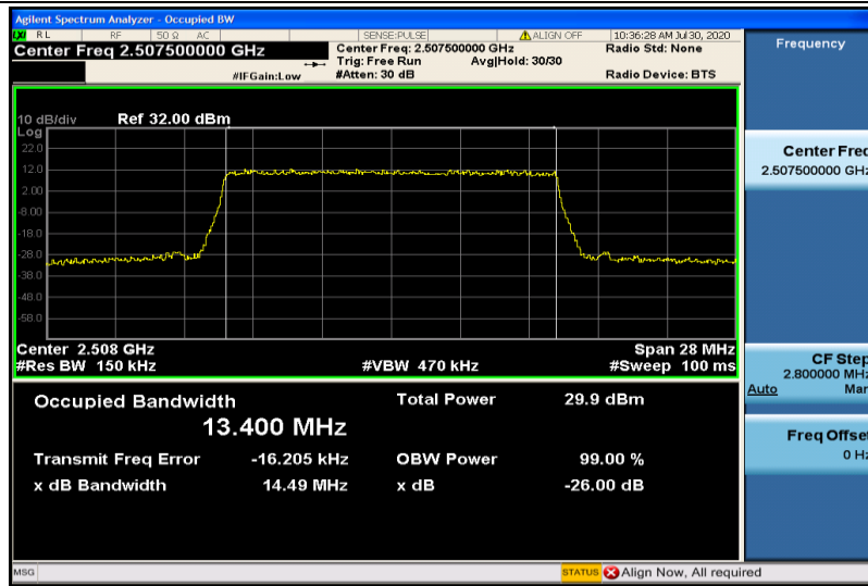
Band7-15MHz-16QAM-20825-75RB#0-13.400
