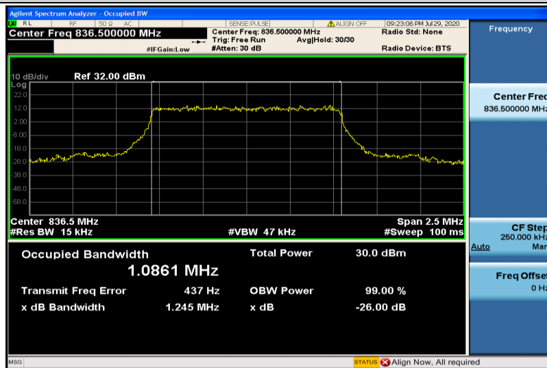
Band5-1.4MHz-QPSK-20525-6RB#0-1.0861
