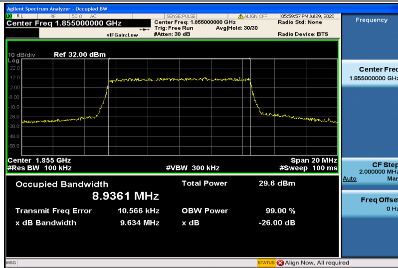
Band2-10MHz-16QAM-18650-50RB#0-8.9361
