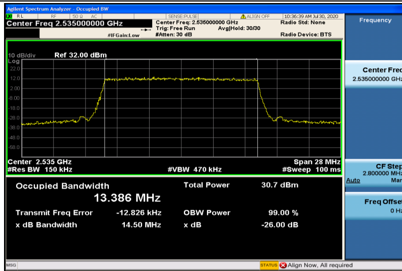
Band7-15MHz-QPSK-21100-75RB#0-13.386
