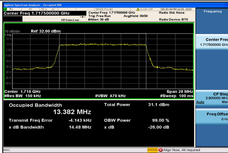
Band4-15MHz-QPSK-20025-75RB#0-13.382
