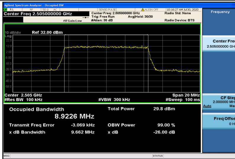
Band7-10MHz-16QAM-20800-50RB#0-8.9226
