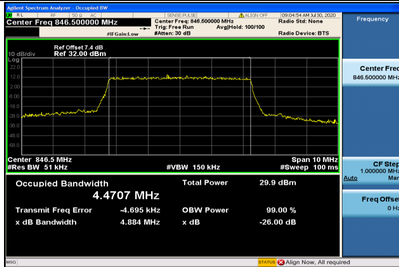
Band5-5MHz-16QAM-20625-25RB#0-4.4707
