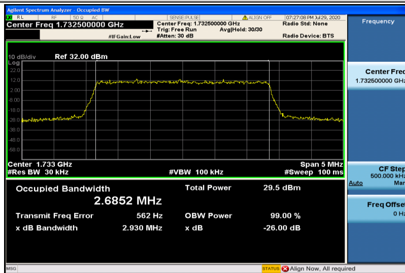
Band4-3MHz-16QAM-20175-15RB#0-2.6852
