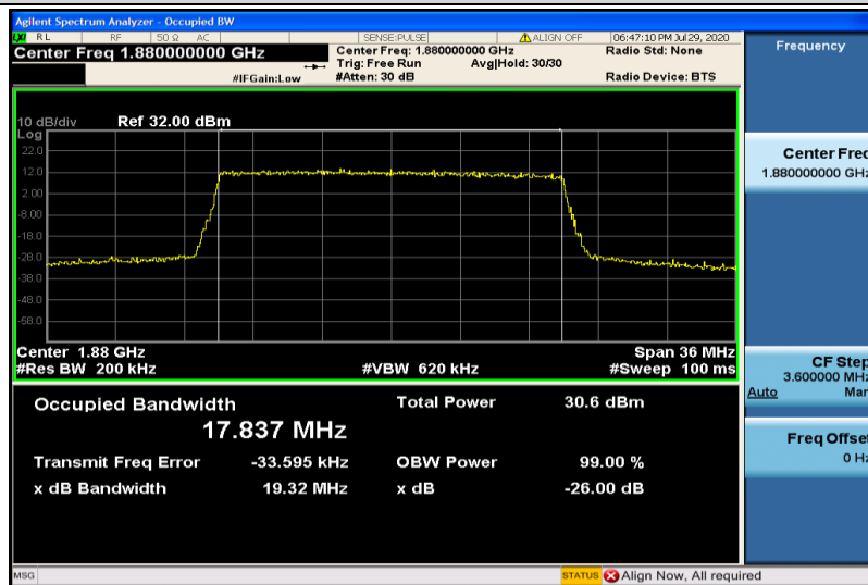
Band2-20MHz-QPSK-18900-100RB#0-17.837
