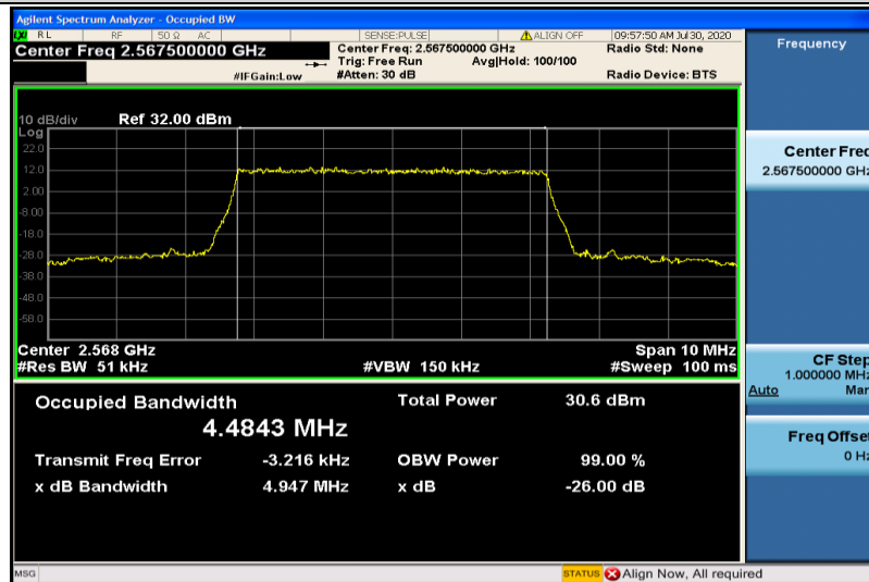
Band7-5MHz-QPSK-21425-25RB#0-4.4843
