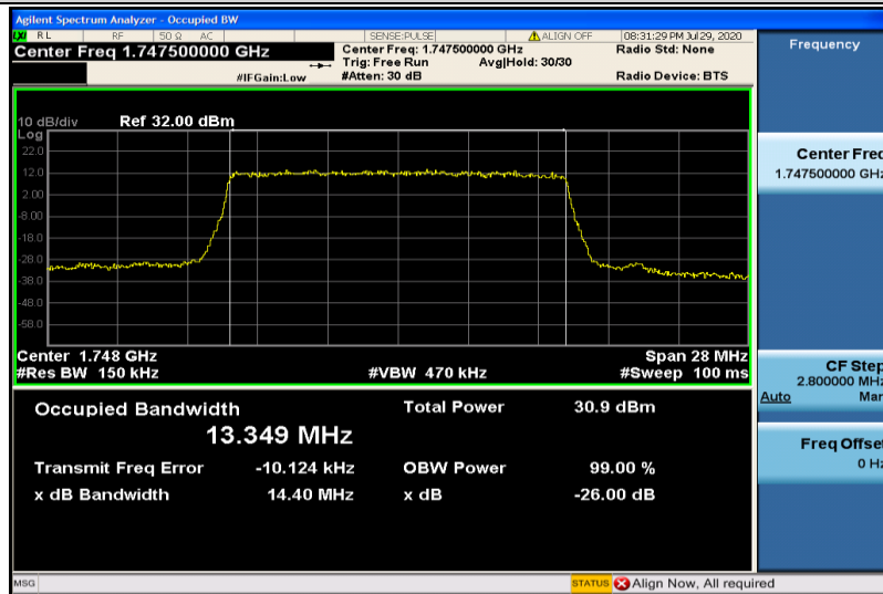
Band4-15MHz-QPSK-20325-75RB#0-13.349
