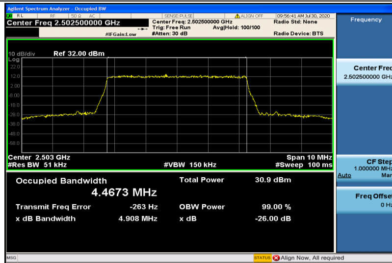
Band7-5MHz-QPSK-20775-25RB#0-4.4673
