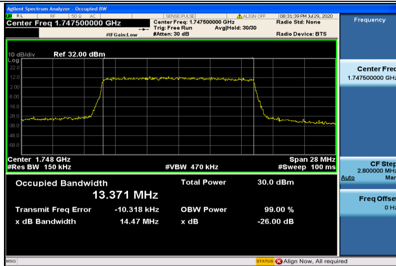
Band4-15MHz-16QAM-20325-75RB#0-13.371
