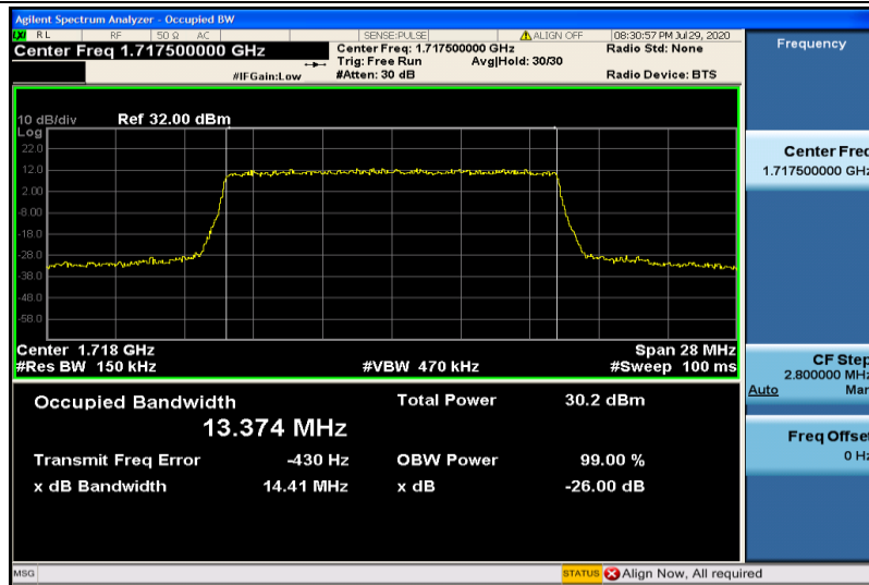
Band4-15MHz-16QAM-20025-75RB#0-13.374
