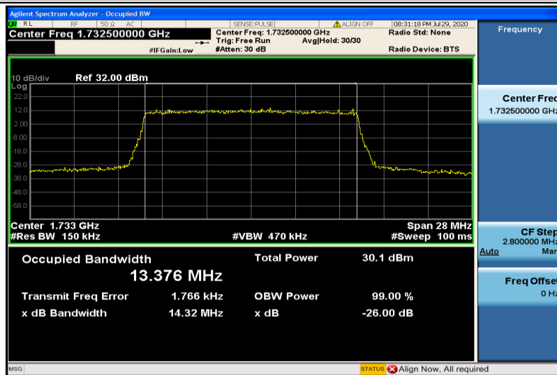
Band4-15MHz-16QAM-20175-75RB#0-13.376
