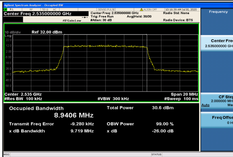
Band7-10MHz-QPSK-21100-50RB#0-8.9406
