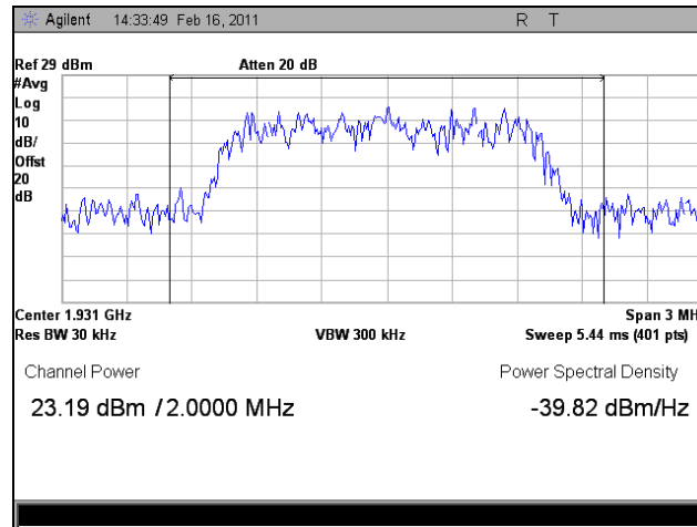
Plot 11. 1930.7 MHz, RF Power Output, Downlink, LTE, Average
