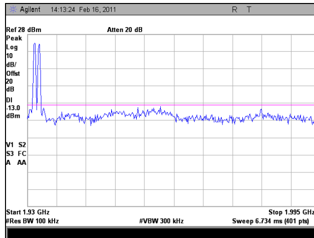
Plot 123. Intermodulation, Downlink, GSM, Low Channel
