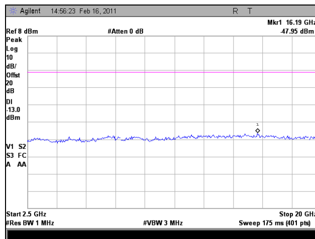
Plot 94. 1930.7 MHz, Conducted Spurious Emissions, Downlink, LTE, 2.5 GHz – 20 GHz
