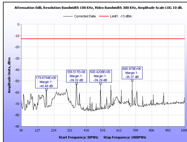
Plot 81. 1994.33 MHz, Radiated Spurious Emissions, Downlink, 30 MHz – 1 GHz
