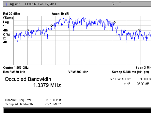
Plot 44. 1962 MHz, Occupied Bandwidth, Downlink, EVDO, Out
