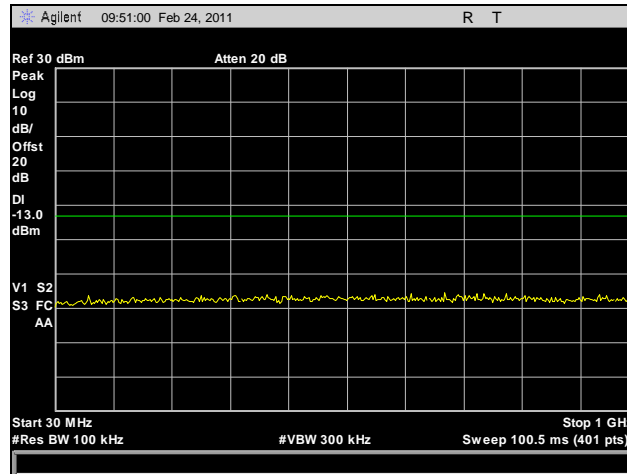
Plot 107. 1994.875 MHz, Conducted Spurious Emissions, Downlink, GSM, 30 MHz – 1 GHz
