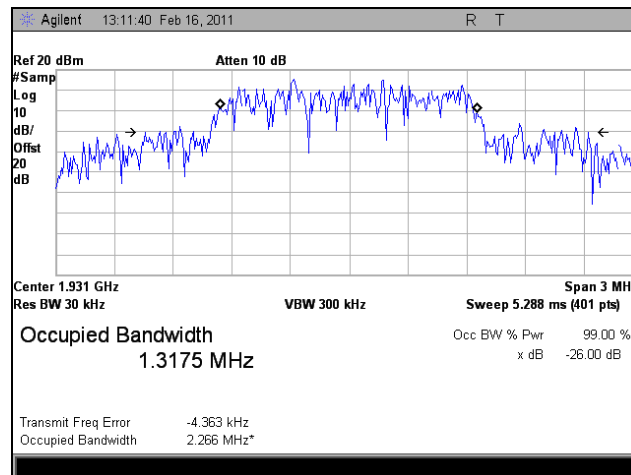
Plot 42. 1930.67 MHz, Occupied Bandwidth, Downlink, EVDO, Out
