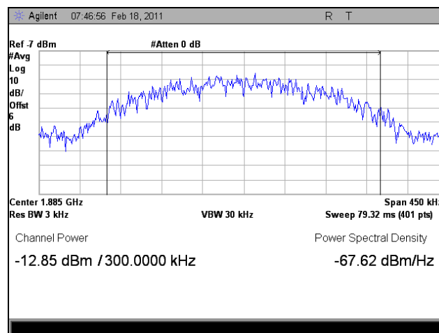
Plot 37. 1885 MHz, RF Power Output, Uplink, GSM, Average
