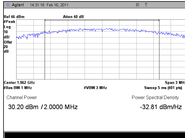
Plot 14. 1962 MHz, RF Power Output, Downlink, LTE, Peak
