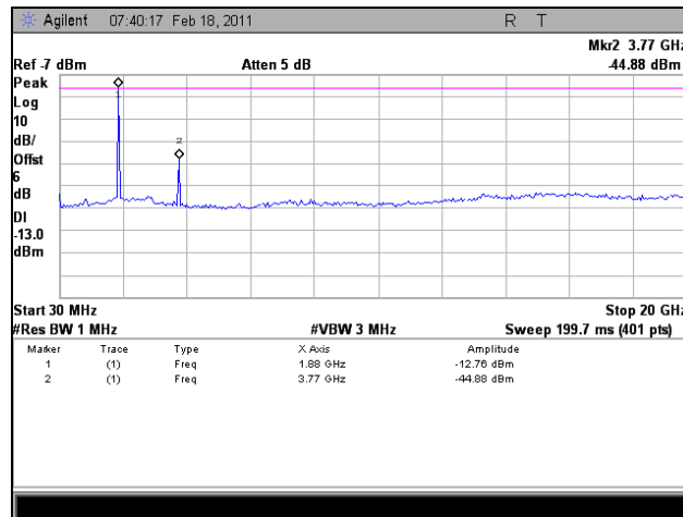
Plot 117. 1885 MHz, Conducted Spurious Emissions, Uplink, GSM, 30 MHz – 20 GHz
