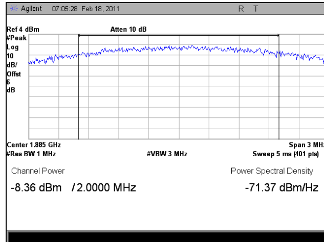
Plot 32. 1885 MHz, RF Power Output, Uplink, LTE, Peak
