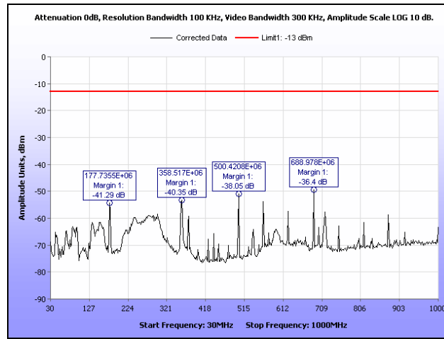
Plot 77. 1930.67 MHz, Radiated Spurious Emissions, Downlink, 30 MHz – 1 GHz
