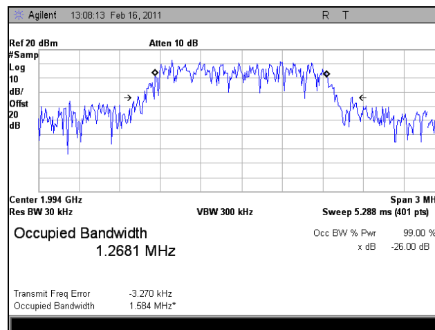
Plot 46. 1994.33 MHz, Occupied Bandwidth, Downlink, EVDO, Out
