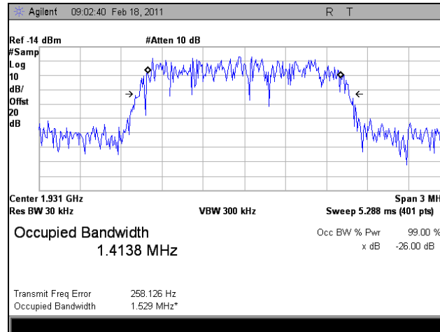
Plot 47. 1930.7 MHz, Occupied Bandwidth, Downlink, LTE, In
