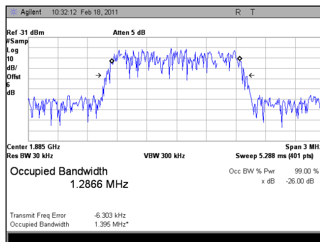
Plot 61. 1885 MHz, Occupied Bandwidth, Uplink, EVDO, In
