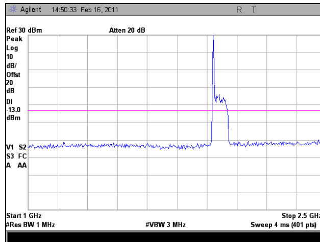
Plot 93. 1930.7 MHz, Conducted Spurious Emissions, Downlink, LTE, 1 GHz – 2.5 GHz
