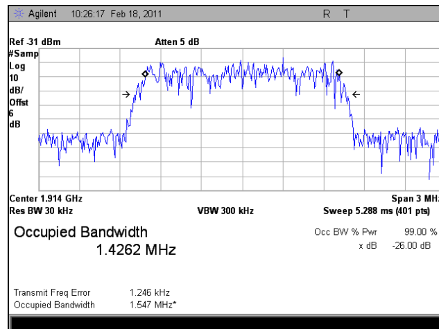
Plot 69. 1914.3 MHz, Occupied Bandwidth, Uplink, LTE, In
