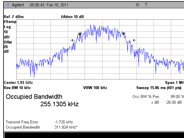
Plot 53. 1930.125 MHz, Occupied Bandwidth, Downlink, GSM, In
