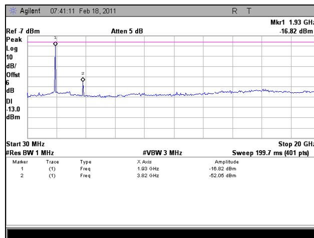
Plot 118. 1914.875 MHz, Conducted Spurious Emissions, Uplink, GSM, 30 MHz – 20 GHz
