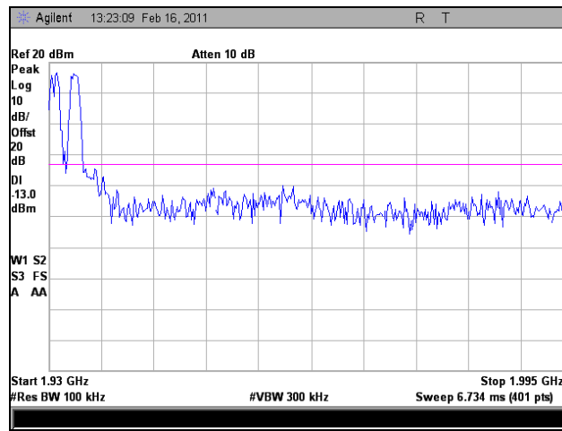
Plot 119. Intermodulation, Downlink, EVDO, Low Channel
