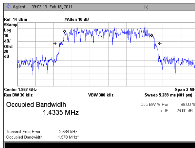
Plot 49. 1962 MHz, Occupied Bandwidth, Downlink, LTE, In
