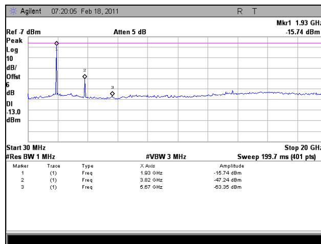
Plot 112. 1914.33 MHz, Conducted Spurious Emissions, Uplink, EVDO, 30 MHz – 20 GHz
