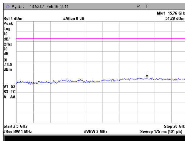
Plot 106. 1962 MHz, Conducted Spurious Emissions, Downlink, GSM, 2.5 GHz – 20 GHz
