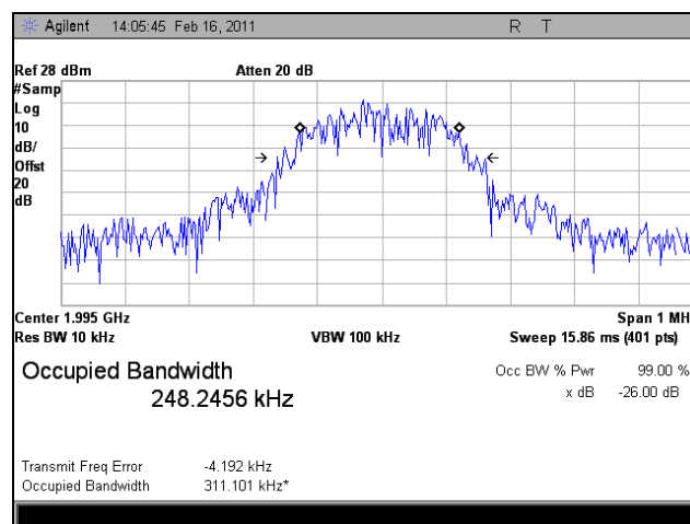
Plot 58. 1994.875 MHz, Occupied Bandwidth, Downlink, GSM, Out
