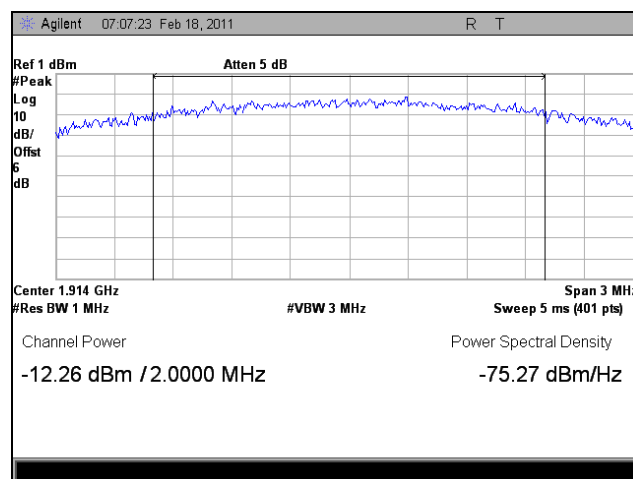
Plot 34. 1914.3 MHz, RF Power Output, Uplink, LTE, Peak
