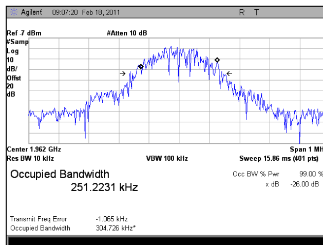
Plot 55. 1962 MHz, Occupied Bandwidth, Downlink, GSM, In
