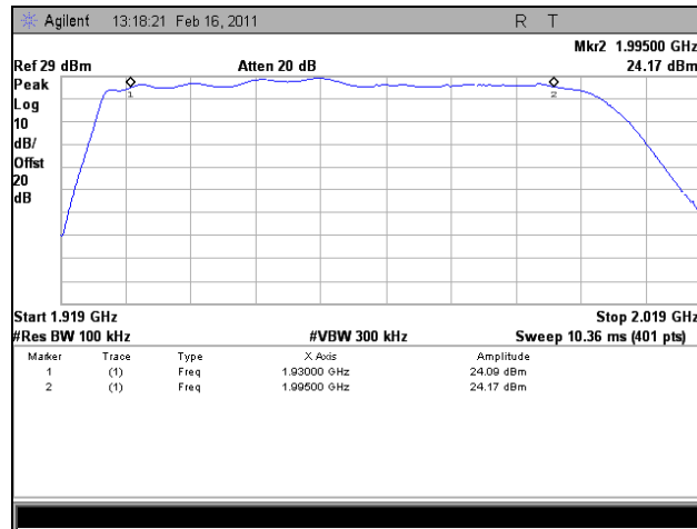
Plot 131. Filter Response, Downlink
