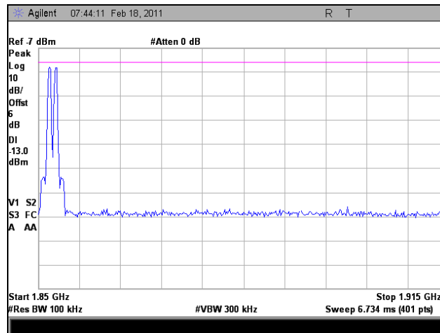
Plot 129. Intermodulation, Uplink, GSM, Low Channel
