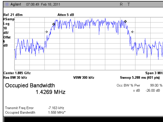
Plot 68. 1885 MHz, Occupied Bandwidth, Uplink, LTE, Out
