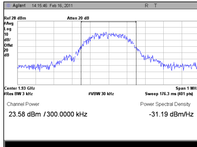
Plot 17. 1930.125 MHz, RF Power Output, Downlink, GSM, Average
