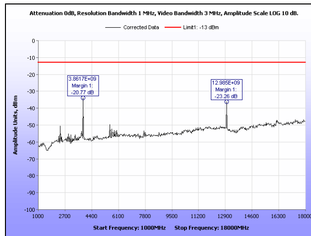
Plot 78. 1930.67 MHz, Radiated Spurious Emissions, Downlink, 1 GHz – 18 GHz
