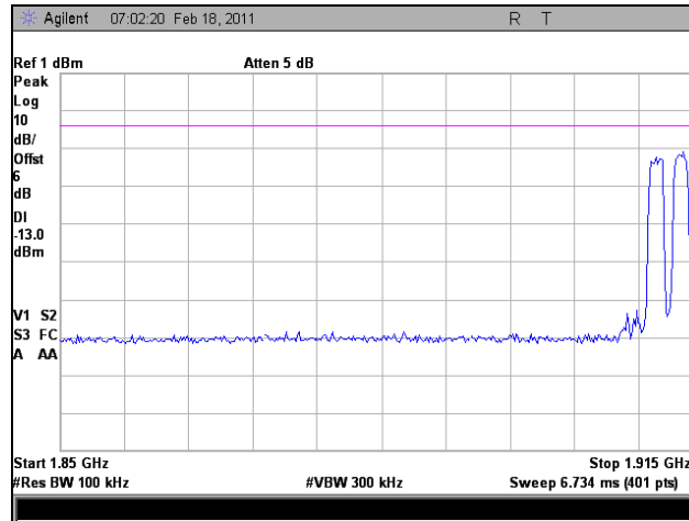
Plot 128. Intermodulation, Uplink, LTE, High Channel
