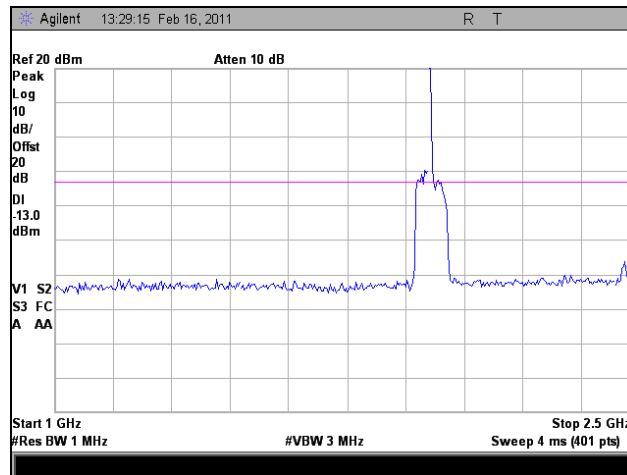
Plot 87. 1962 MHz, Conducted Spurious Emissions, Downlink, EVDO, 1 GHz – 2.5 GHz
