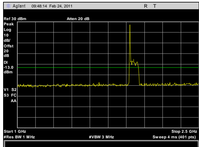
Plot 102. 1930.125 MHz, Conducted Spurious Emissions, Downlink, GSM, 1 GHz – 2.5 GHz
