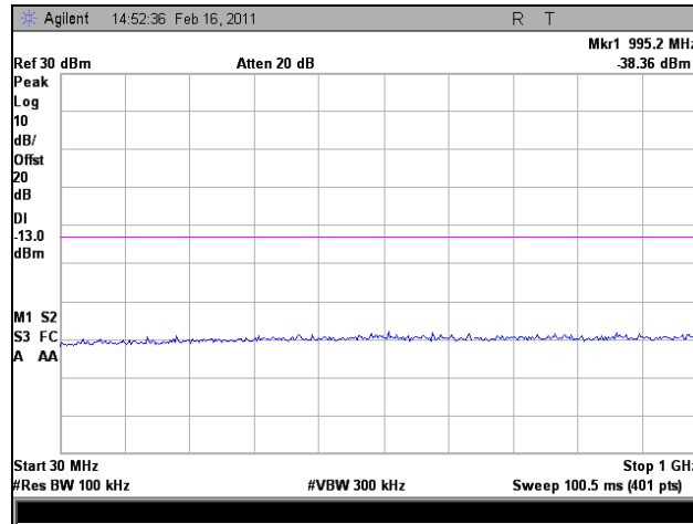
Plot 98. 1994.3 MHz, Conducted Spurious Emissions, Downlink, LTE, 30 MHz – 1 GHz
