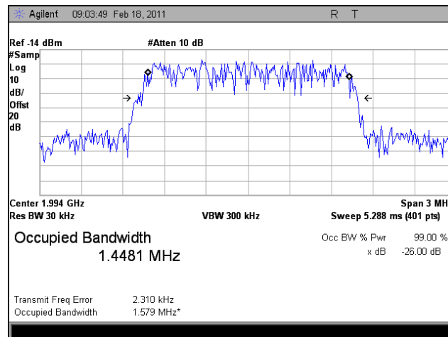
Plot 51. 1994.3 MHz, Occupied Bandwidth, Downlink, LTE, In
