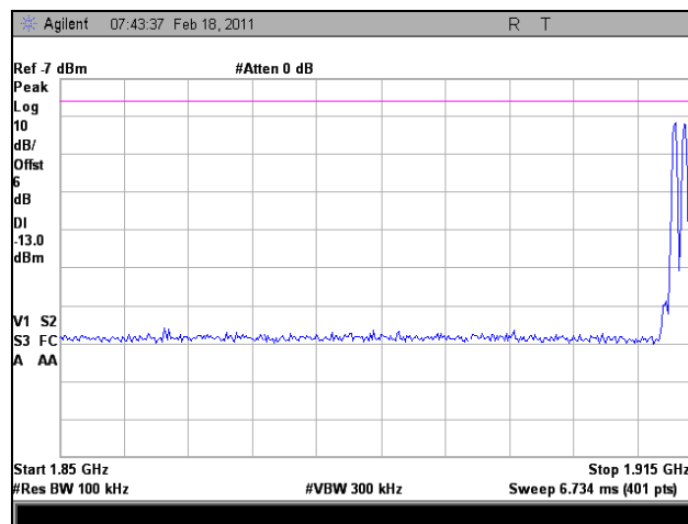
Plot 130. Intermodulation, Uplink, GSM, High Channel
