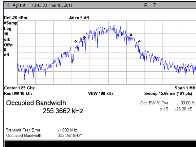
Plot 71. 1850.125 MHz, Occupied Bandwidth, Uplink, GSM, In
