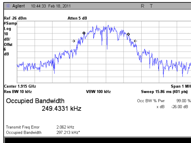
Plot 75. 1914.875 MHz, Occupied Bandwidth, Uplink, GSM, In
