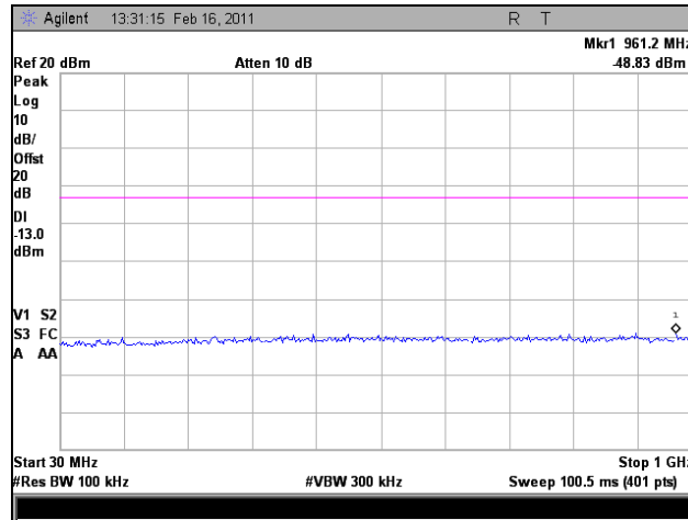
Plot 86. 1962 MHz, Conducted Spurious Emissions, Downlink, EVDO, 30 MHz – 1 GHz
