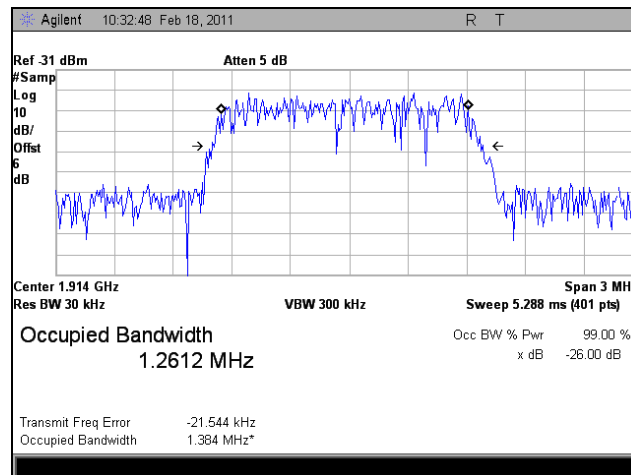
Plot 63. 1914.33 MHz, Occupied Bandwidth, Uplink, EVDO, In
