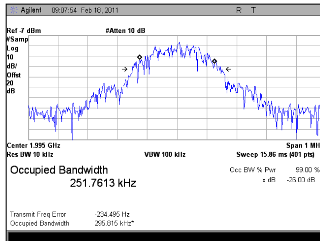
Plot 57. 1994.875 MHz, Occupied Bandwidth, Downlink, GSM, In
