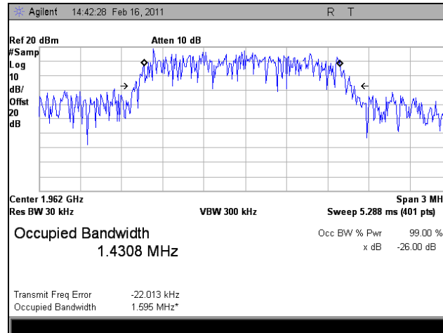
Plot 50. 1962 MHz, Occupied Bandwidth, Downlink, LTE, Out
