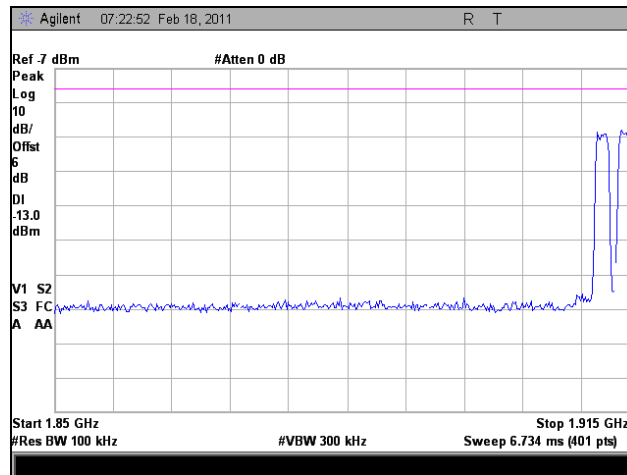
Plot 126. Intermodulation, Uplink, EVDO, High Channel
