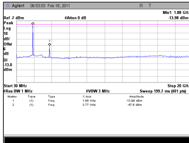
Plot 114. 1885 MHz, Conducted Spurious Emissions, Uplink, LTE, 30 MHz – 20 GHz
