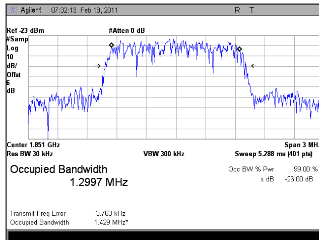
Plot 60. 1850.67 MHz, Occupied Bandwidth, Uplink, EVDO, Out
