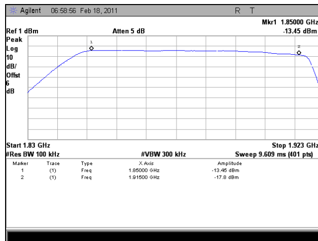
Plot 132. Filter Response, Uplink
