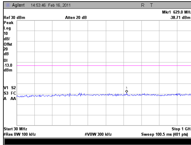
Plot 92. 1930.7 MHz, Conducted Spurious Emissions, Downlink, LTE, 30 MHz – 1 GHz
