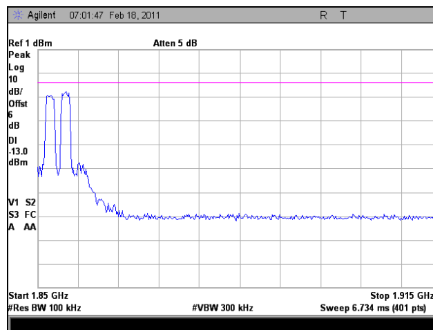
Plot 127. Intermodulation, Uplink, LTE, Low Channel
