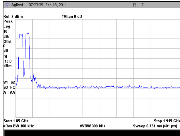
Plot 125. Intermodulation, Uplink, EVDO, Low Channel
