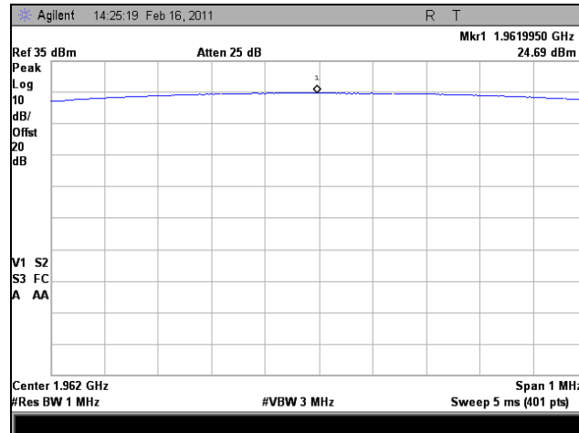
Plot 20. 1962 MHz, RF Power Output, Downlink, GSM, Peak
