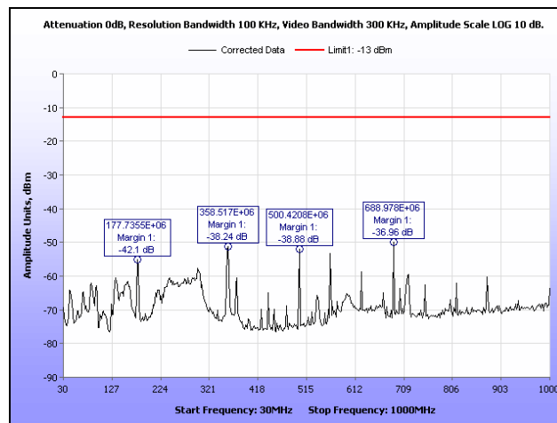
Plot 79. 1962 MHz, Radiated Spurious Emissions, Downlink, 30 MHz – 1 GHz
