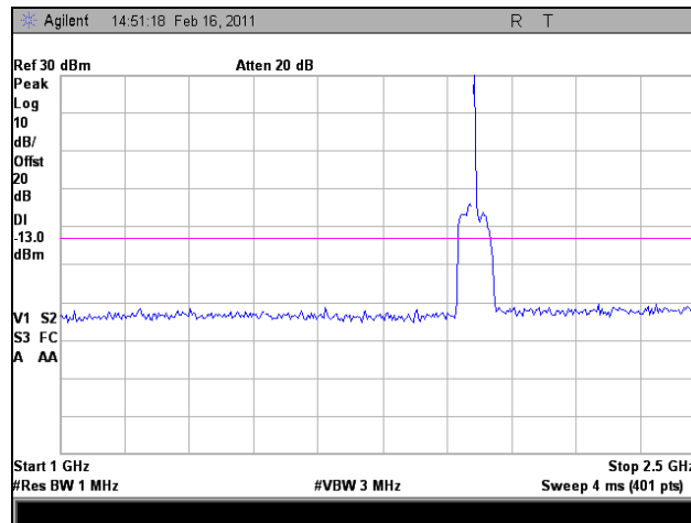
Plot 96. 1962 MHz, Conducted Spurious Emissions, Downlink, LTE, 1 GHz – 2.5 GHz
