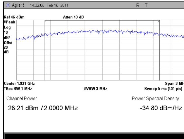
Plot 12. 1930.7 MHz, RF Power Output, Downlink, LTE, Peak
