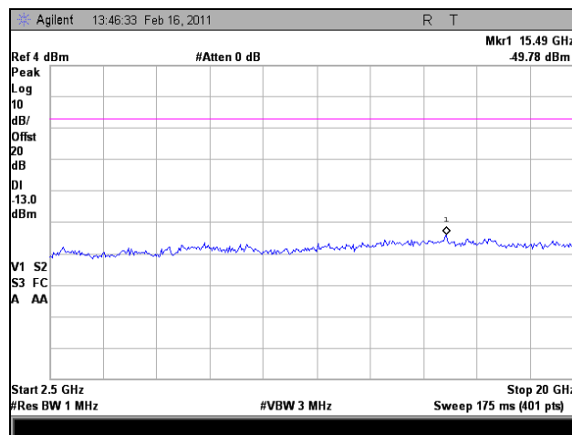
Plot 91. 1994.33 MHz, Conducted Spurious Emissions, Downlink, EVDO, 2.5 GHz – 20 GHz
