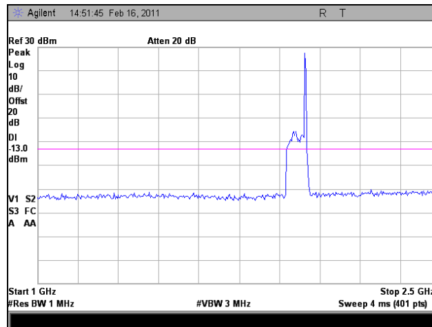
Plot 99. 1994.3 MHz, Conducted Spurious Emissions, Downlink, LTE, 1 GHz – 2.5 GHz
