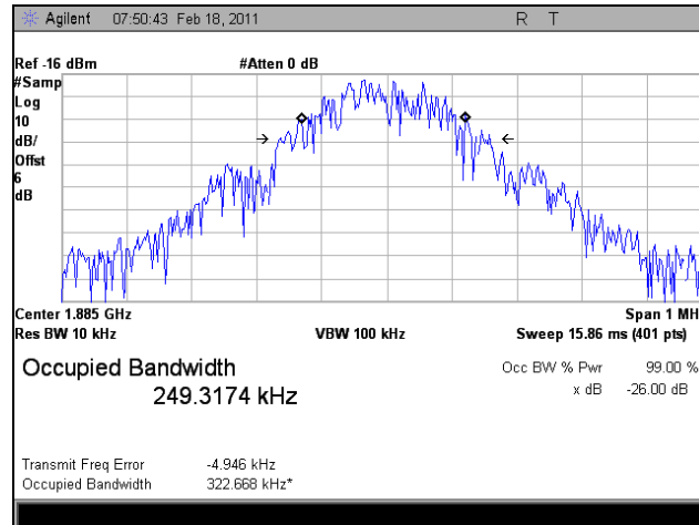
Plot 74. 1885 MHz, Occupied Bandwidth, Uplink, GSM, Out
