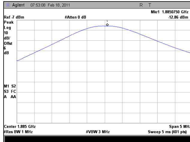
Plot 38. 1885 MHz, RF Power Output, Uplink, GSM, Peak
