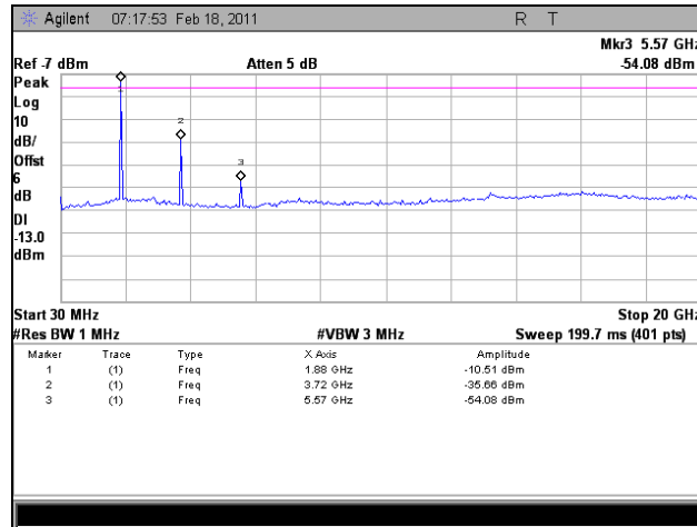
Plot 110. 1950.67 MHz, Conducted Spurious Emissions, Uplink, EVDO, 30 MHz – 20 GHz
