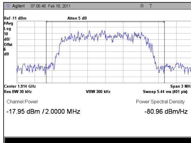
Plot 33. 1914.3 MHz, RF Power Output, Uplink, LTE, Average
