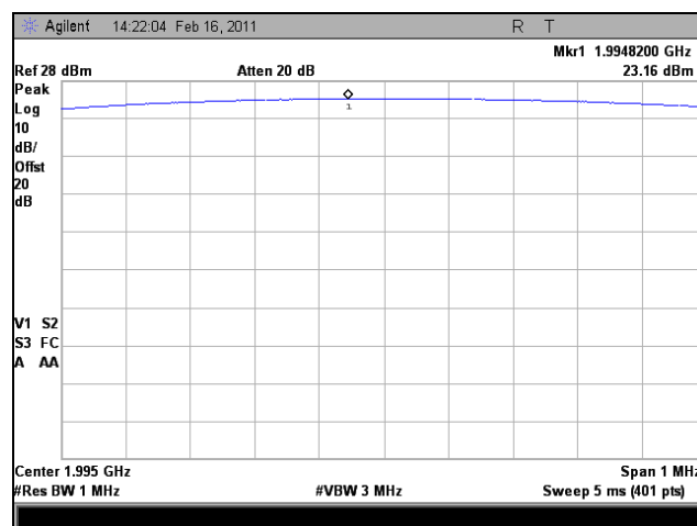
Plot 22. 1994.875 MHz, RF Power Output, Downlink, GSM, Peak
