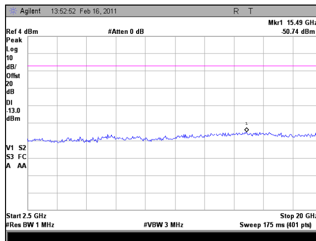
Plot 109. 1994.875 MHz, Conducted Spurious Emissions, Downlink, GSM, 2.5 GHz – 20 GHz
