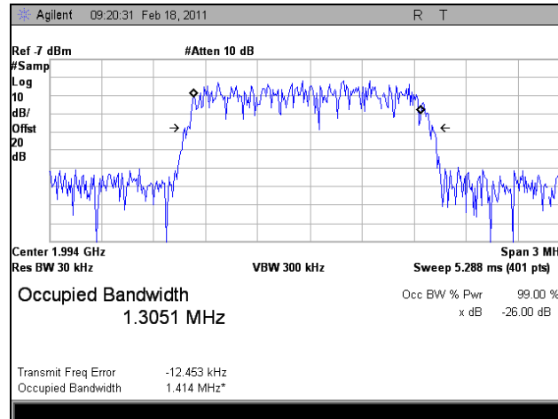
Plot 45. 1994.33 MHz, Occupied Bandwidth, Downlink, EVDO, In
