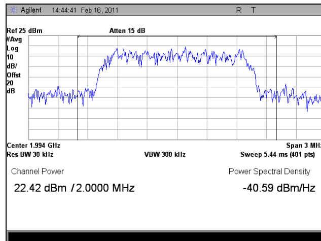
Plot 15. 1994.3 MHz, RF Power Output, Downlink, LTE, Average
