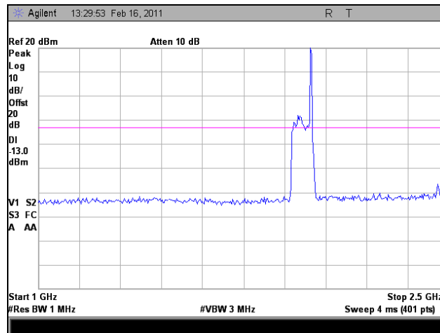
Plot 90. 1994.33 MHz, Conducted Spurious Emissions, Downlink, EVDO, 1 GHz – 2.5 GHz
