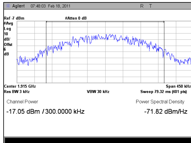
Plot 39. 1914.875 MHz, RF Power Output, Uplink, GSM, Average
