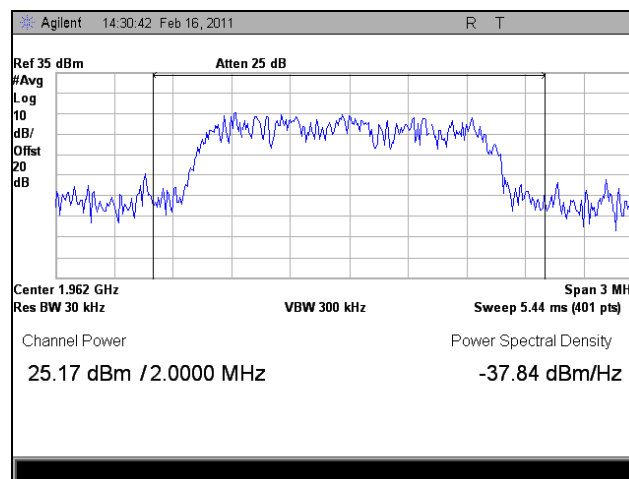
Plot 13. 1962 MHz, RF Power Output, Downlink, LTE, Average
