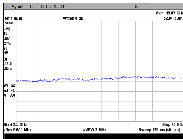
Plot 88. 1962 MHz, Conducted Spurious Emissions, Downlink, EVDO, 2.5 GHz – 20 GHz
