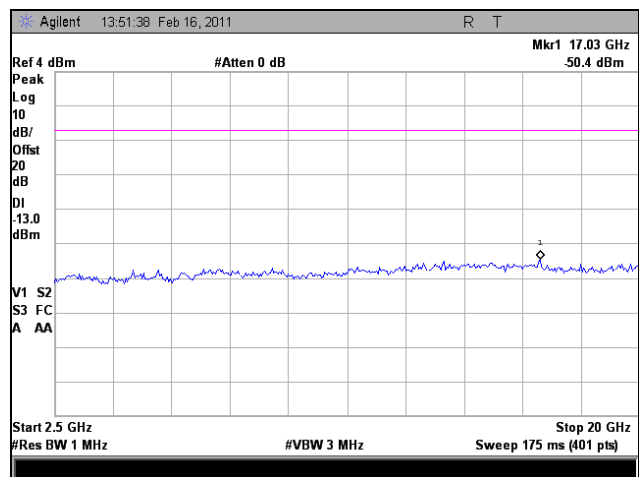
Plot 103. 1930.125 MHz, Conducted Spurious Emissions, Downlink, GSM, 2.5 GHz – 20 GHz
