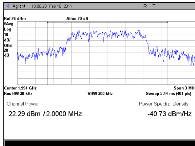
Plot 9. 1994.33 MHz, RF Power Output, Downlink, EVDO, Average
