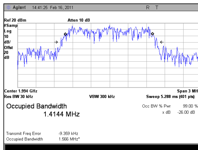
Plot 52. 1994.3 MHz, Occupied Bandwidth, Downlink, LTE, Out
