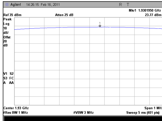
Plot 18. 1930.125 MHz, RF Power Output, Downlink, GSM, Peak
