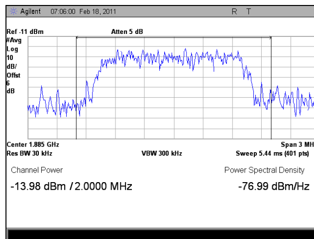
Plot 31. 1885 MHz, RF Power Output, Uplink, LTE, Average
