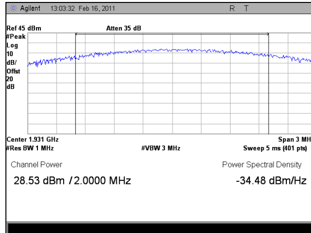
Plot 6. 1930.67 MHz, RF Power Output, Downlink, EVDO, Peak
