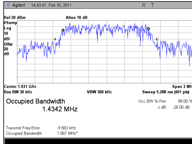
Plot 48. 1930.7 MHz, Occupied Bandwidth, Downlink, LTE, Out
