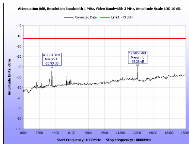
Plot 82. 1994.33 MHz, Radiated Spurious Emissions, Downlink, 1 GHz – 18 GHz
