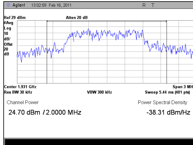
Plot 5. 1930.67 MHz, RF Power Output, Downlink, EVDO, Average
