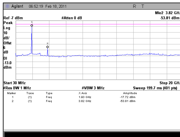
Plot 115. 1914.3 MHz, Conducted Spurious Emissions, Uplink, LTE, 30 MHz – 20 GHz
