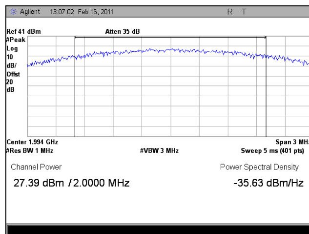
Plot 10. 1994.33 MHz, RF Power Output, Downlink, EVDO, Peak
