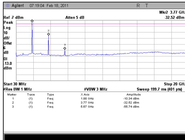
Plot 111. 1885 MHz, Conducted Spurious Emissions, Uplink, EVDO, 30 MHz – 20 GHz
