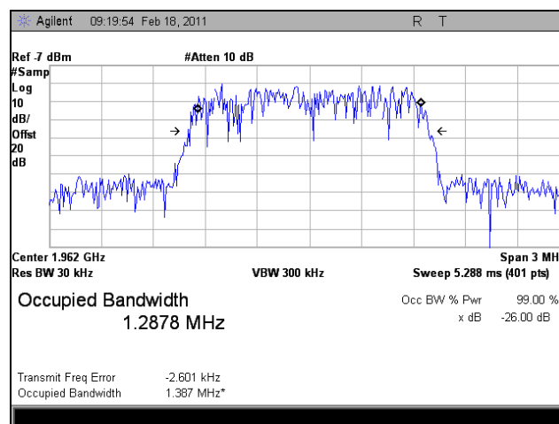
Plot 43. 1962 MHz, Occupied Bandwidth, Downlink, EVDO, In
