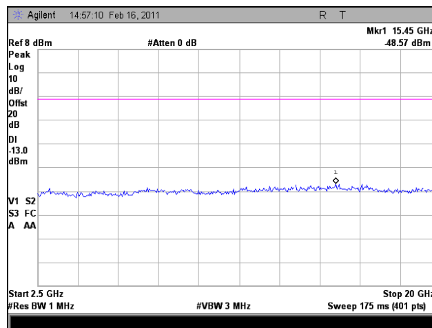
Plot 100. 1994.3 MHz, Conducted Spurious Emissions, Downlink, LTE, 2.5 GHz – 20 GHz
