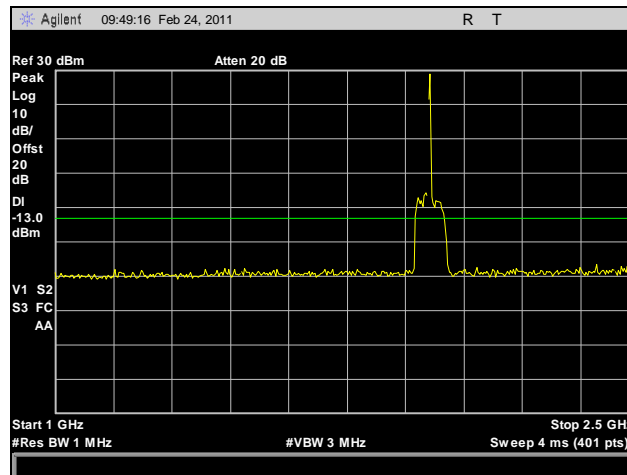
Plot 105. 1962 MHz, Conducted Spurious Emissions, Downlink, GSM, 1 GHz – 2.5 GHz
