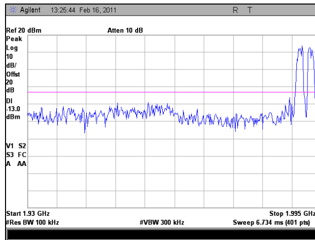
Plot 120. Intermodulation, Downlink, EVDO, High Channel
