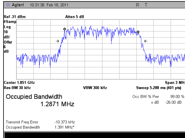
Plot 59. 1850.67 MHz, Occupied Bandwidth, Uplink, EVDO, In
