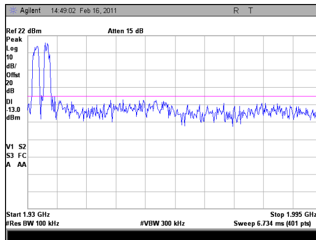
Plot 121. Intermodulation, Downlink, LTE, Low Channel
