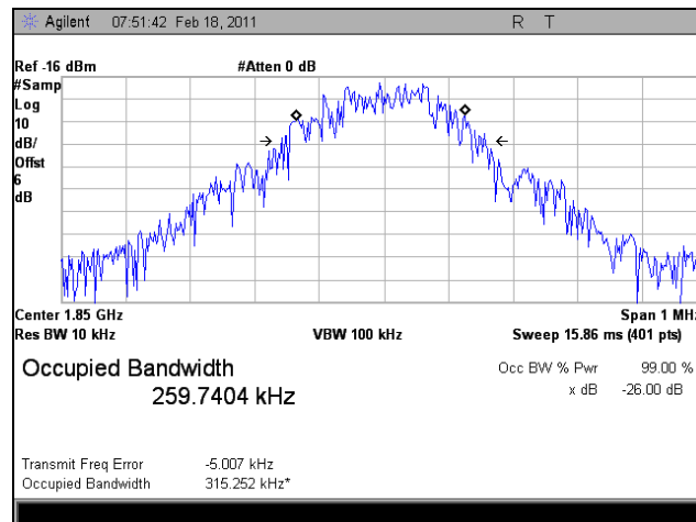
Plot 72. 1850.125 MHz, Occupied Bandwidth, Uplink, GSM, Out
