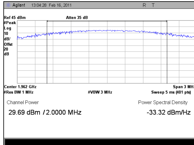
Plot 8. 1962 MHz, RF Power Output, Downlink, EVDO, Peak
