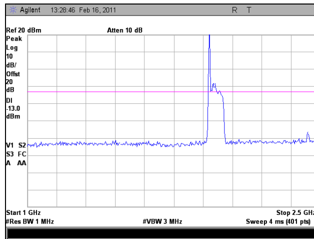
Plot 84. 1930.67 MHz, Conducted Spurious Emissions, Downlink, EVDO, 1 GHz – 2.5 GHz
