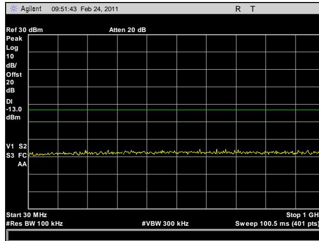
Plot 104. 1962 MHz, Conducted Spurious Emissions, Downlink, GSM, 30 MHz – 1 GHz
