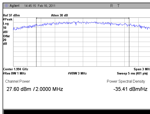
Plot 16. 1994.3 MHz, RF Power Output, Downlink, LTE, Peak
