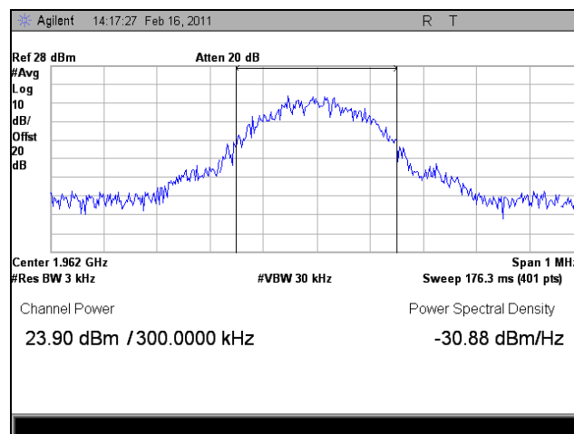
Plot 19. 1962 MHz, RF Power Output, Downlink, GSM, Average
