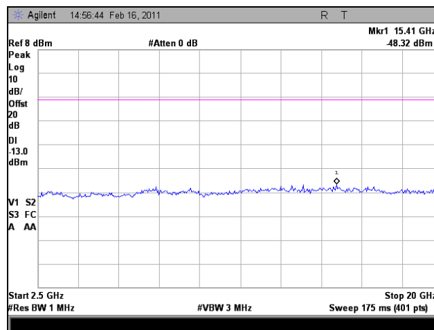
Plot 97. 1962 MHz, Conducted Spurious Emissions, Downlink, LTE, 2.5 GHz – 20 GHz
