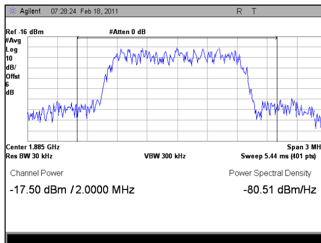
Plot 25. 1885 MHz, RF Power Output, Uplink, EVDO, Average
