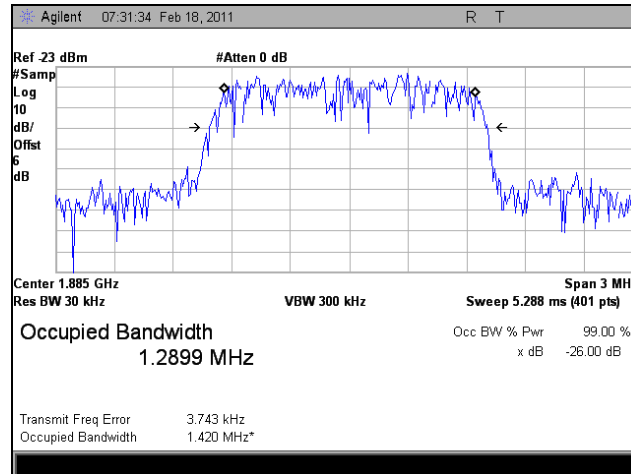
Plot 62. 1885 MHz, Occupied Bandwidth, Uplink, EVDO, Out
