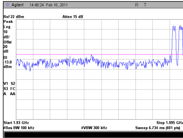
Plot 122. Intermodulation, Downlink, LTE, High Channel
