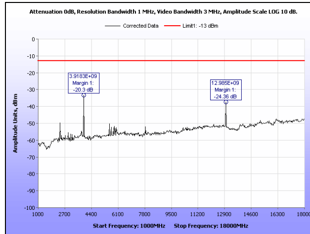
Plot 80. 1962 MHz, Radiated Spurious Emissions, Downlink, 1 GHz – 18 GHz
