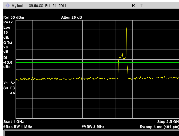
Plot 108. 1994.875 MHz, Conducted Spurious Emissions, Downlink, GSM, 1 GHz – 2.5 GHz
