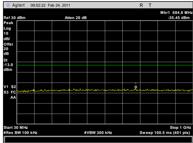
Plot 101. 1930.125 MHz, Conducted Spurious Emissions, Downlink, GSM, 30 MHz – 1 GHz
