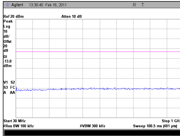
Plot 89. 1994.33 MHz, Conducted Spurious Emissions, Downlink, EVDO, 30 MHz – 1 GHz
