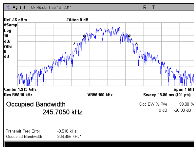
Plot 76. 1914.875 MHz, Occupied Bandwidth, Uplink, GSM, Out
