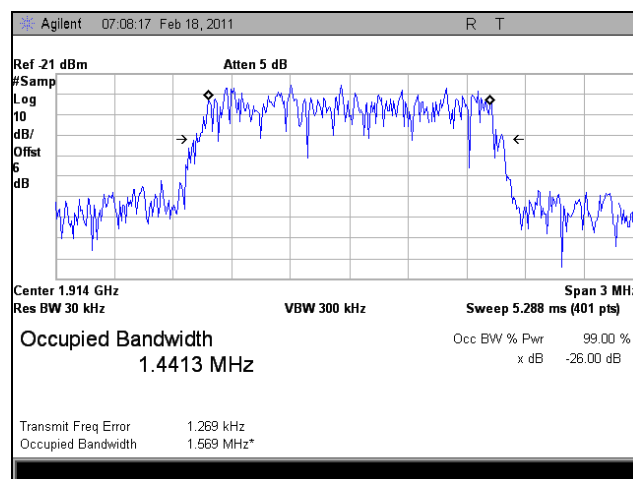
Plot 70. 1914.3 MHz, Occupied Bandwidth, Uplink, LTE, Out
