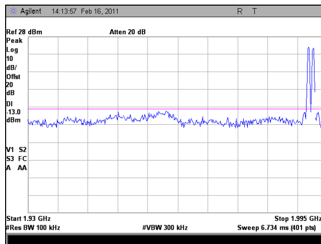
Plot 124. Intermodulation, Downlink, GSM, High Channel
