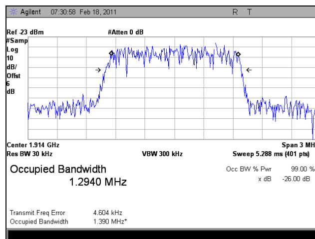
Plot 64. 1914.33 MHz, Occupied Bandwidth, Uplink, EVDO, Out
