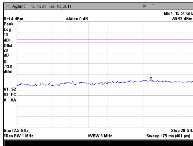
Plot 85. 1930.67 MHz, Conducted Spurious Emissions, Downlink, EVDO, 2.5 GHz – 20 GHz
