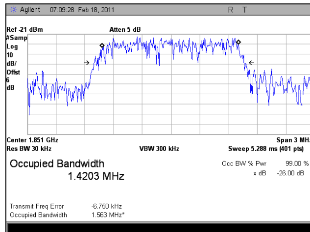
Plot 66. 1850.7 MHz, Occupied Bandwidth, Uplink, LTE, Out
