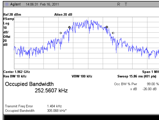
Plot 56. 1962 MHz, Occupied Bandwidth, Downlink, GSM, Out
