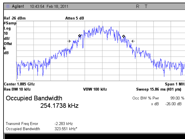
Plot 73. 1885 MHz, Occupied Bandwidth, Uplink, GSM, In
