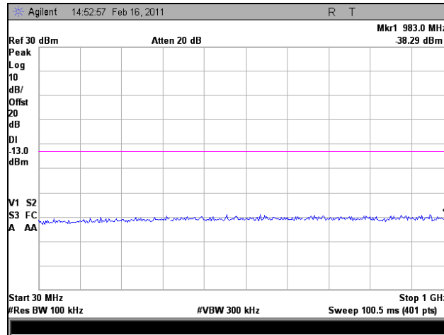
Plot 95. 1962 MHz, Conducted Spurious Emissions, Downlink, LTE, 30 MHz – 1 GHz
