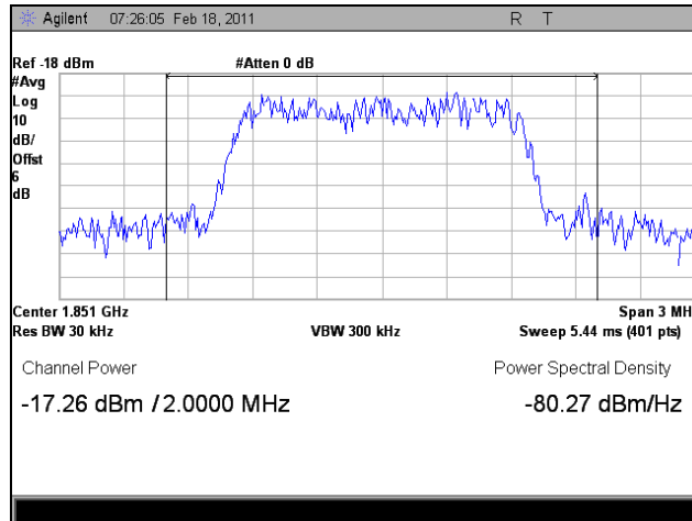
Plot 23. 1850.67 MHz, RF Power Output, Uplink, EVDO, Average
