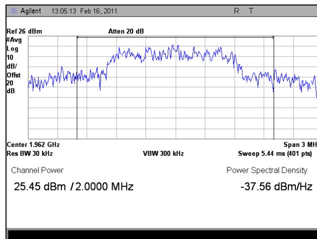
Plot 7. 1962 MHz, RF Power Output, Downlink, EVDO, Average
