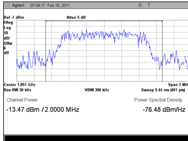
Plot 29. 1850.7 MHz, RF Power Output, Uplink, LTE, Average
