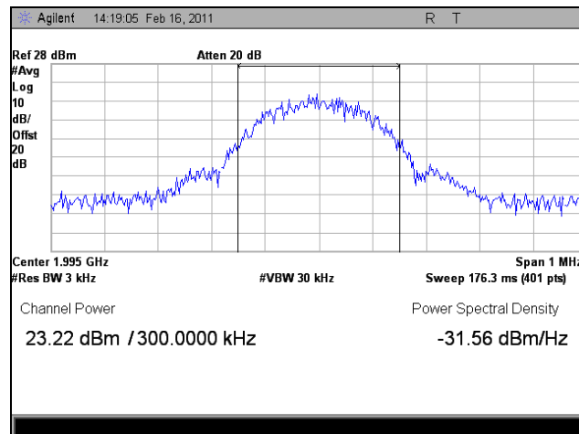
Plot 21. 1994.875 MHz, RF Power Output, Downlink, GSM, Average
