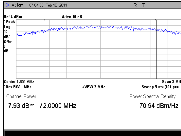
Plot 30. 1850.7 MHz, RF Power Output, Uplink, LTE, Peak
