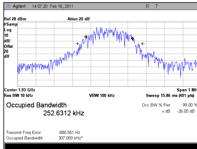
Plot 54. 1930.125 MHz, Occupied Bandwidth, Downlink, GSM, Out
