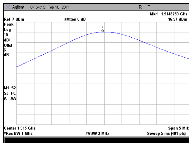
Plot 40. 1914.875 MHz, RF Power Output, Uplink, GSM, Peak
