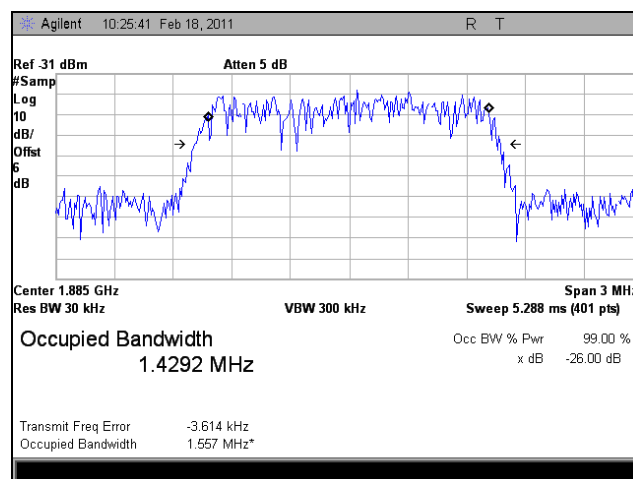
Plot 67. 1885 MHz, Occupied Bandwidth, Uplink, LTE, In
