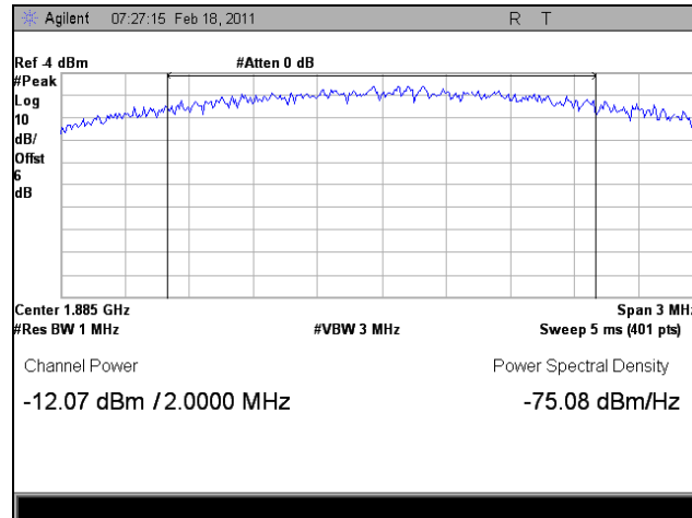
Plot 26. 1885 MHz, RF Power Output, Uplink, EVDO, Peak
