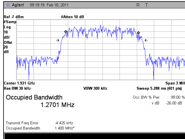
Plot 41. 1930.67 MHz, Occupied Bandwidth, Downlink, EVDO, In
