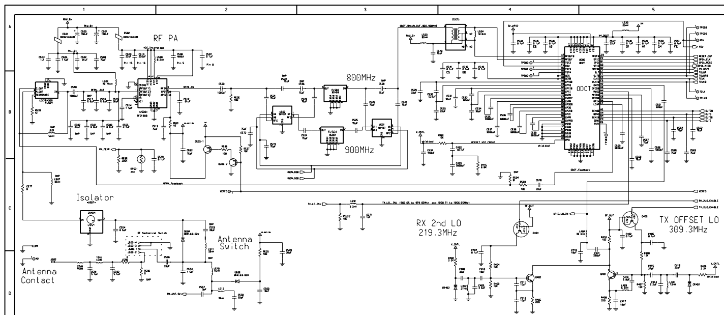
i30sx Transmitter Schematic
