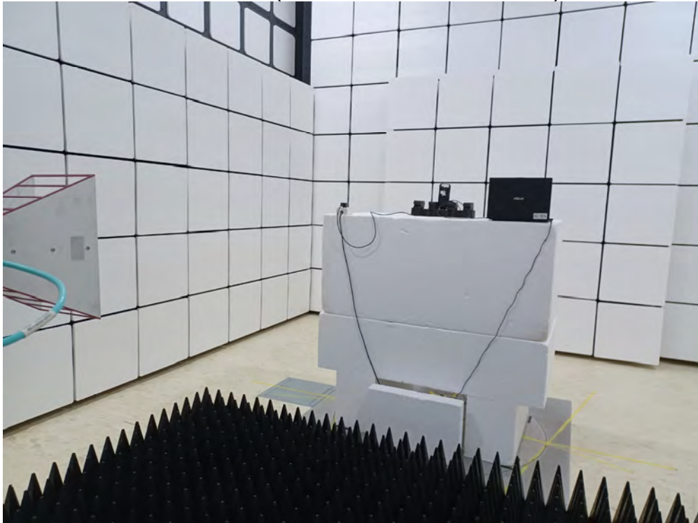
Radiated Test (1GHz to 18GHz, For WCDMA)
