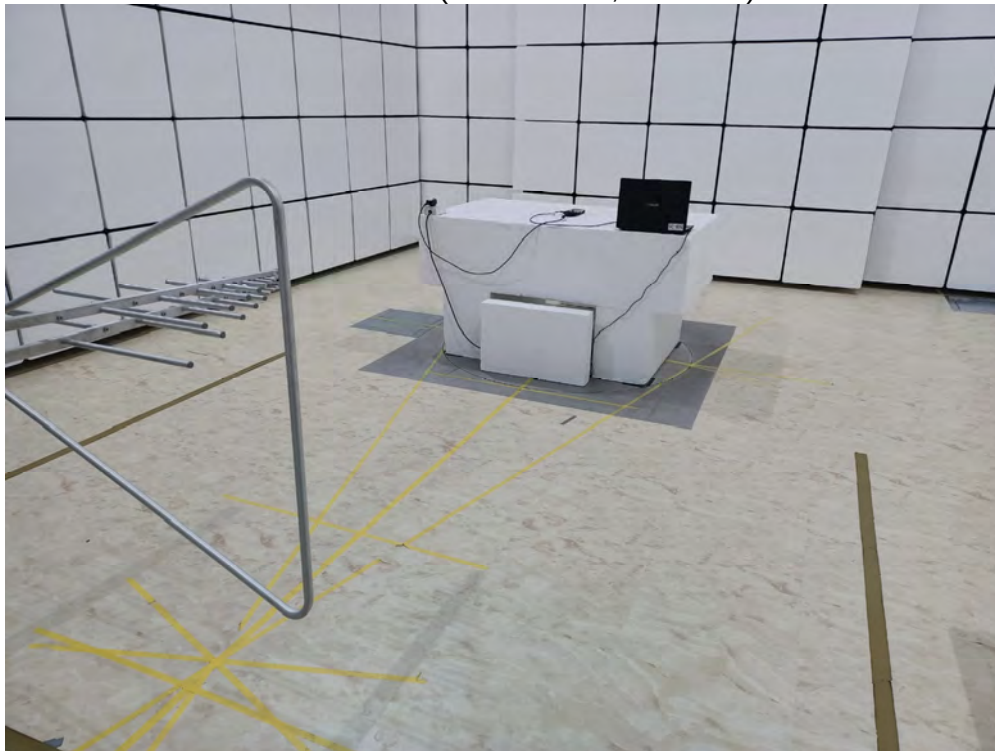
Radiated Test (Above 1GHz, For GSM)
