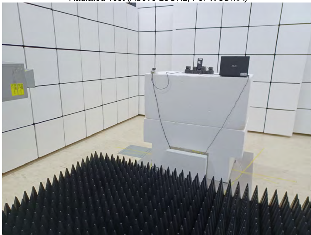
Radiated Test (Above 18GHz, For WCDMA)
