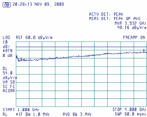
Plot 7.3.65 Radiated emission measurements from 1.0 to 4.0 GHz at the first mid carrier frequency
