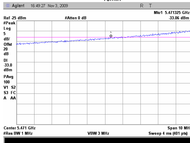
Plot 7.5.34 Band edge emissions at normal conditions 10th minute
