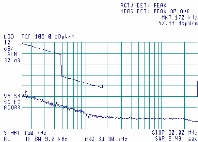
Plot 7.3.59 Radiated emission measurements from 0.15 MHz to 30 MHz at the high carrier frequency
