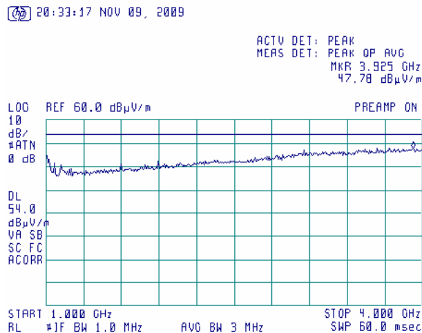
Plot 7.3.67 Radiated emission measurements from 1.0 to 4.0 GHz at the high carrier frequency
