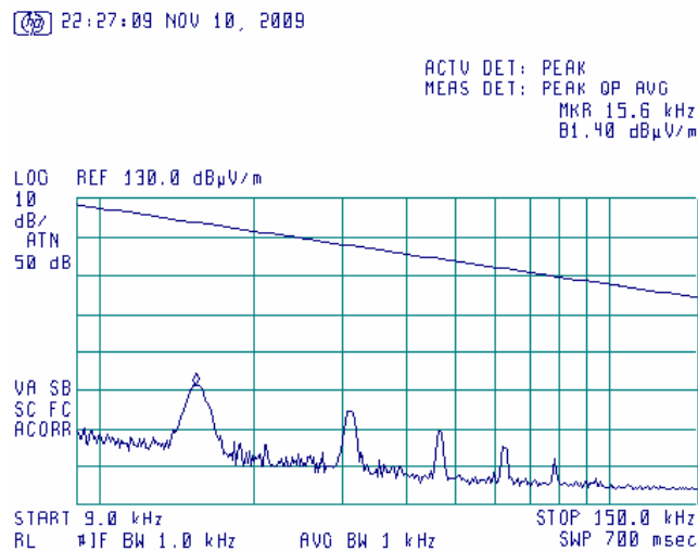
Plot 7.3.55 Radiated emission measurements from 9 to 150 kHz at the high carrier frequency
