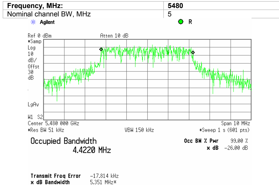
Plot 8.1.2 The 99%power bandwidth test result at low frequency, 64QAM modulation
