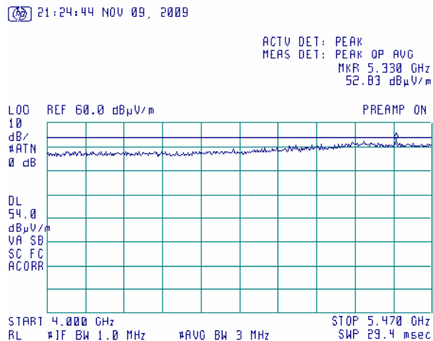
Plot 7.3.71 Radiated emission measurements from 4.0 to 5.47 GHz at the first mid carrier frequency
