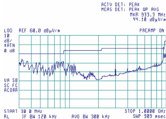
Plot 7.3.63 Radiated emission measurements from 30 MHz to 1000 MHz at the high carrier frequency
