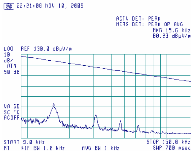
Plot 7.3.53 Radiated emission measurements from 9 to 150 kHz at the first mid carrier frequency
