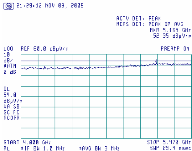
Plot 7.3.75 Radiated emission measurements from 4.0 to 5.47 GHz at the high carrier frequency
