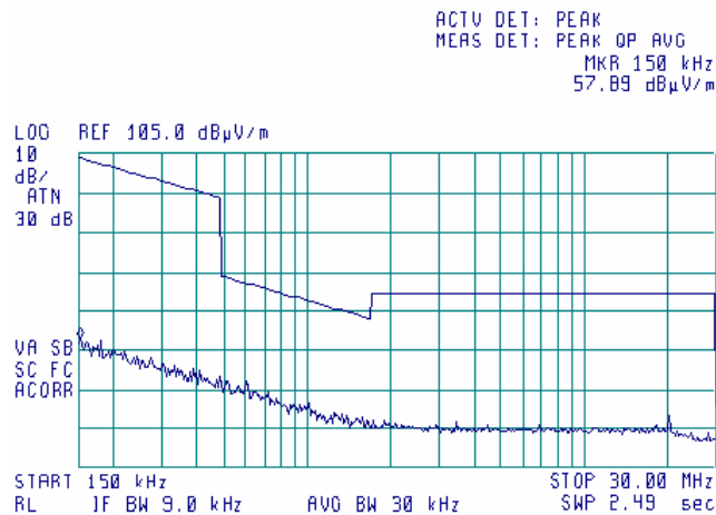
Plot 7.3.57 Radiated emission measurements from 0.15 MHz to 30 MHz at the first mid carrier frequency
