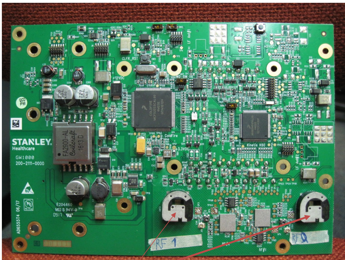
Internal Wireless PIFA Antennas
