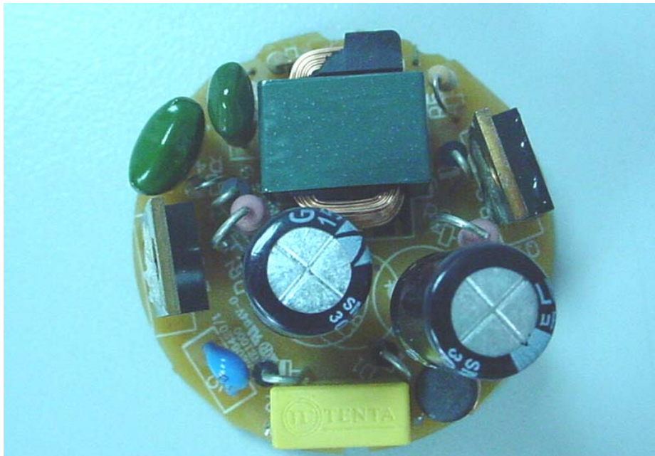
Figure 7 M/N: CL-20WL/25WL Main Board, Component Side
