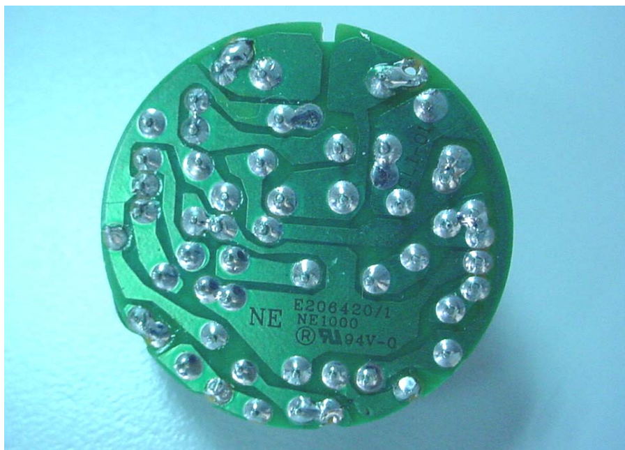
Figure 6 M/N: CL-10WL/15WL Main Board, Cu Foil Side
