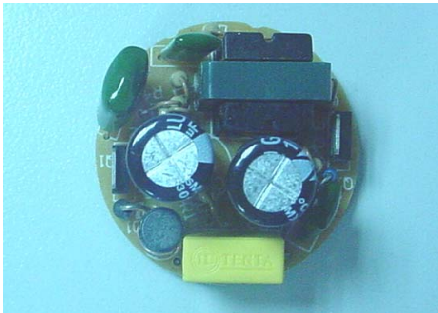
Figure 5 M/N: CL-10WL/15WL Main Board, Component Side
