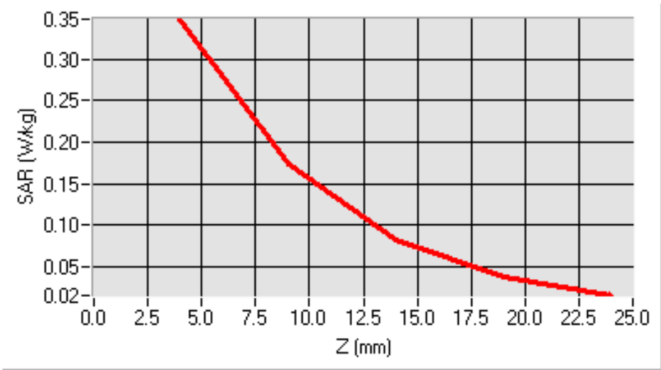
SAR, Z Axis Scan (X = -57, Y = -28)
