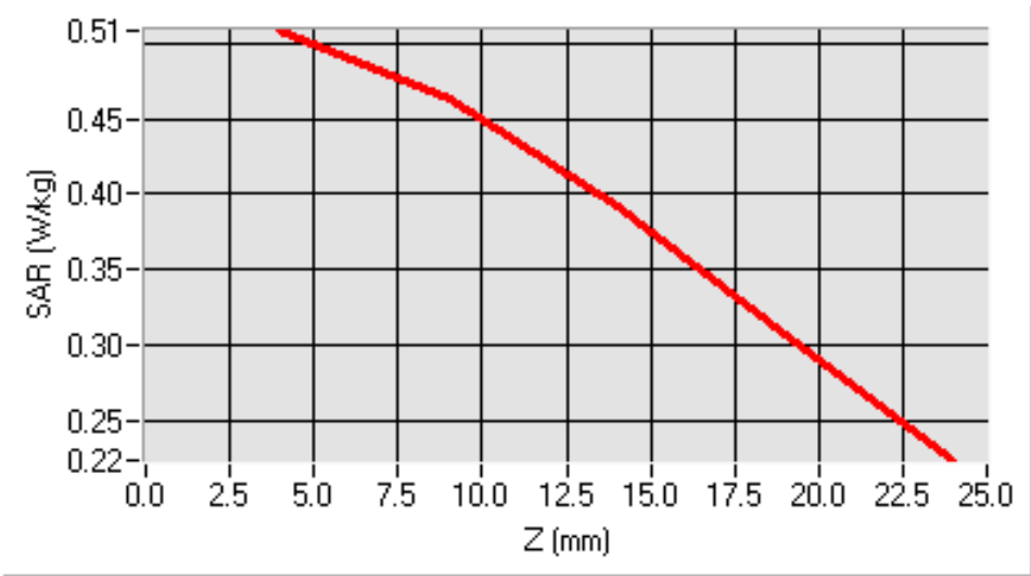
SAR, Z Axis Scan (X = -34, Y = -25)
