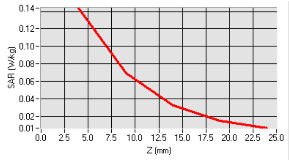
SAR, Z Axis Scan (X = -47, Y = -41)
