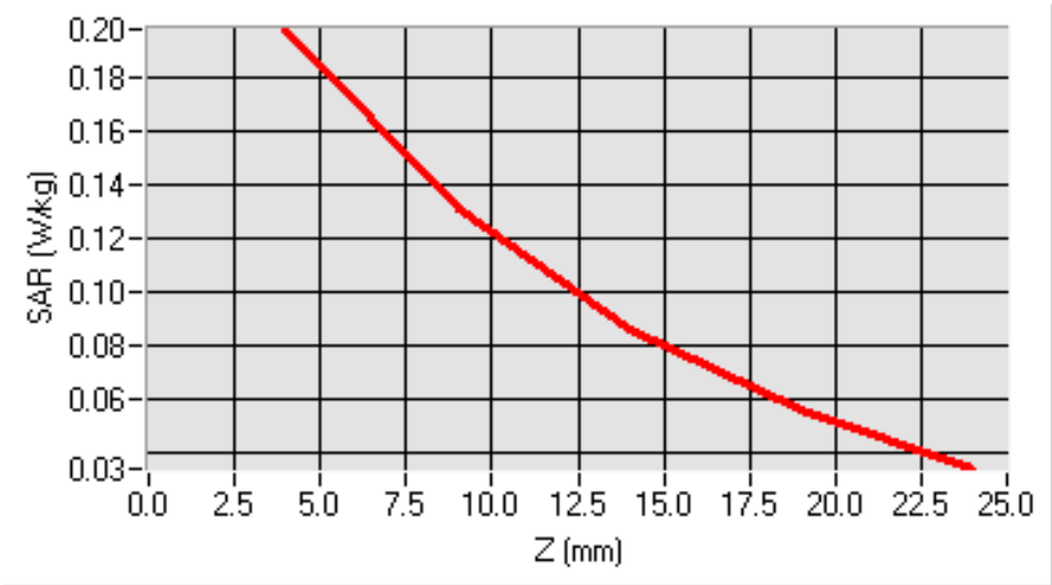
SAR, Z Axis Scan (X = -7, Y = -40)
