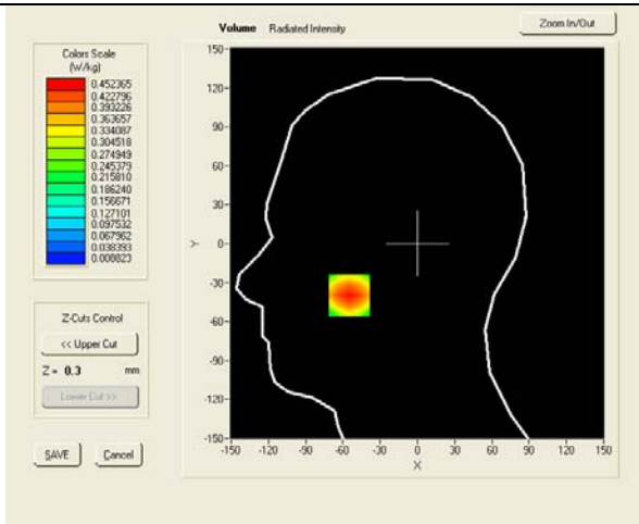
SAR, Z Axis Scan (X = -55, Y = -40)
