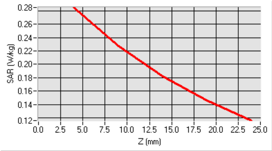
SAR, Z Axis Scan (X = -32, Y = -8)
