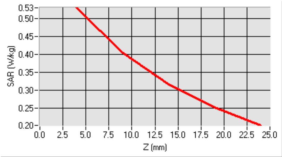
SAR, Z Axis Scan (X = -41, Y = -24)
