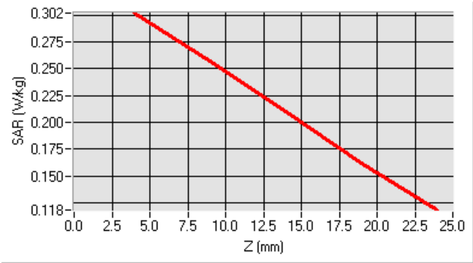
SAR, Z Axis Scan (X = -38, Y = -16)
