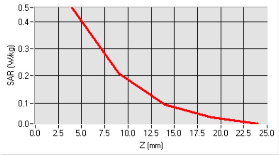
SAR, Z Axis Scan (X = -55, Y = -40)
