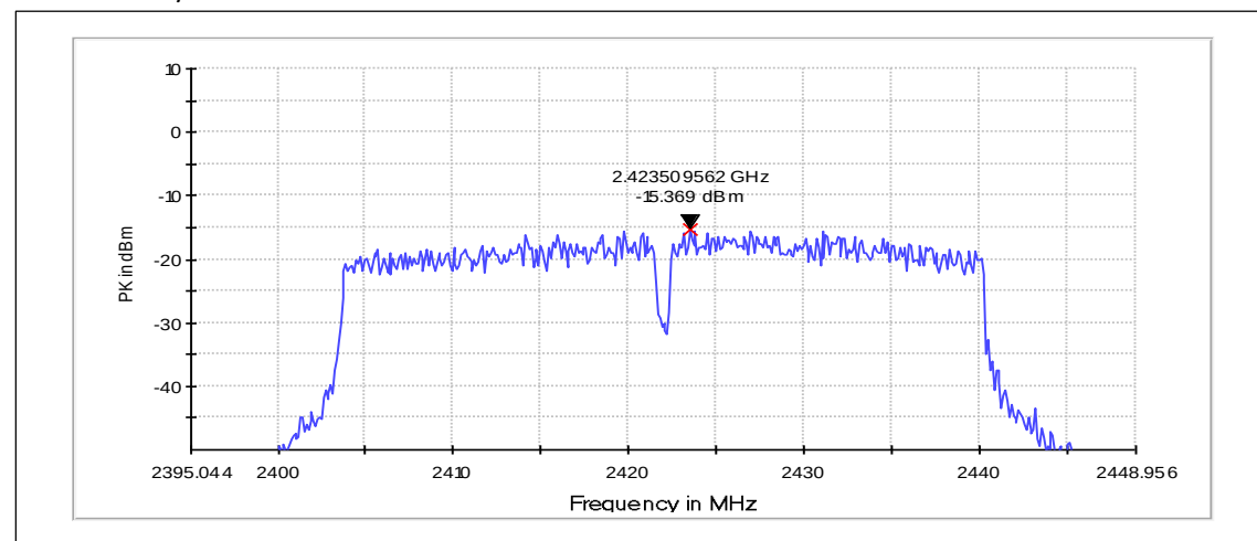
Channel 1-5 / 2422 MHz
