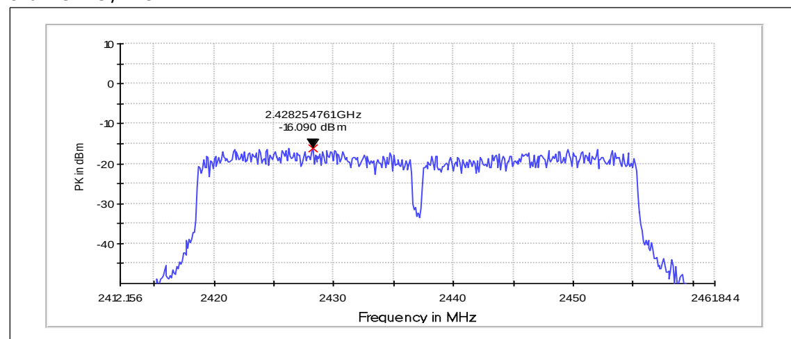
Channel 4-8 / 2437 MHz
