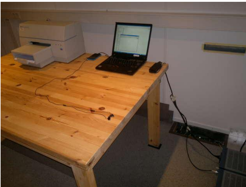
Picture 4. FCC Part 15B AC powerline conducted emissions
