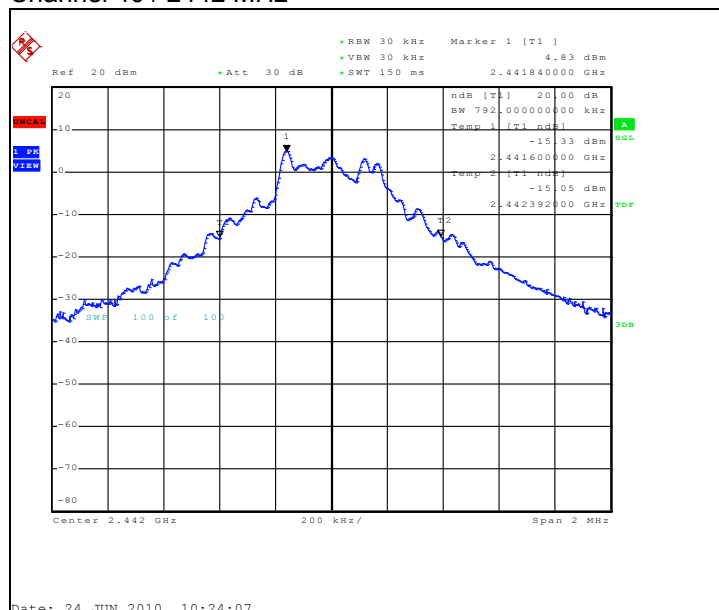
Channel 40 / 2442 MHz
