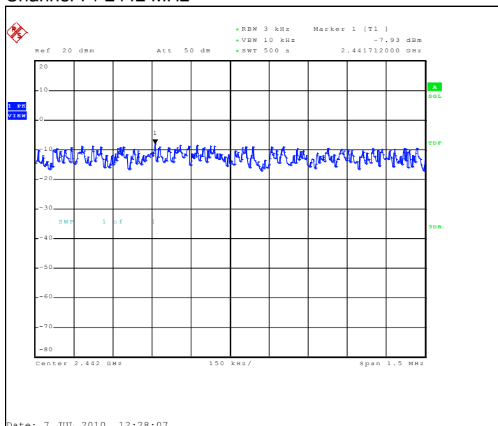
Channel 7 / 2442 MHz
