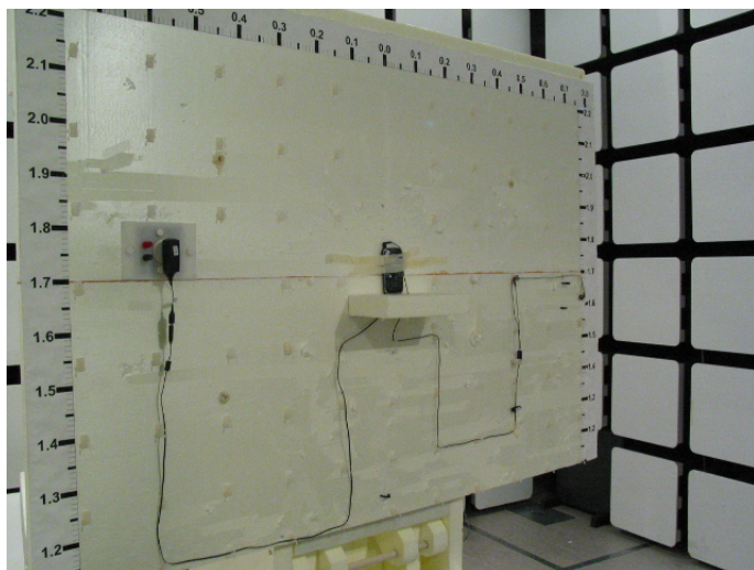
Picture 1 Radiated emission 15C
