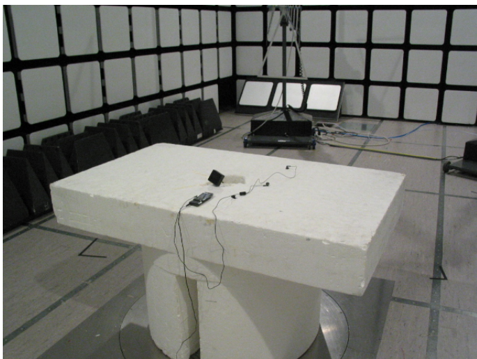
Picture 3 Radiated emission measurement GSM RX + GPS receiver on / FM radio on
