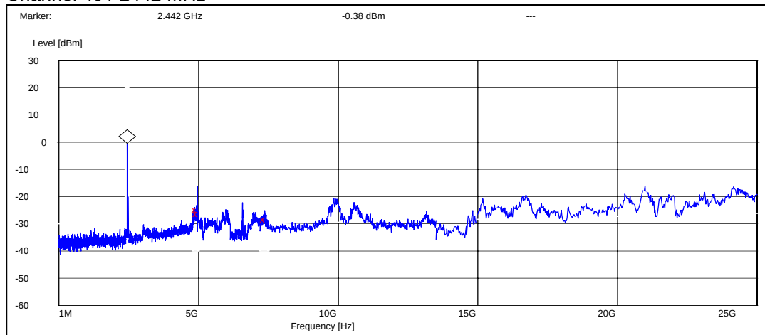
Channel 40 / 2442 MHz
