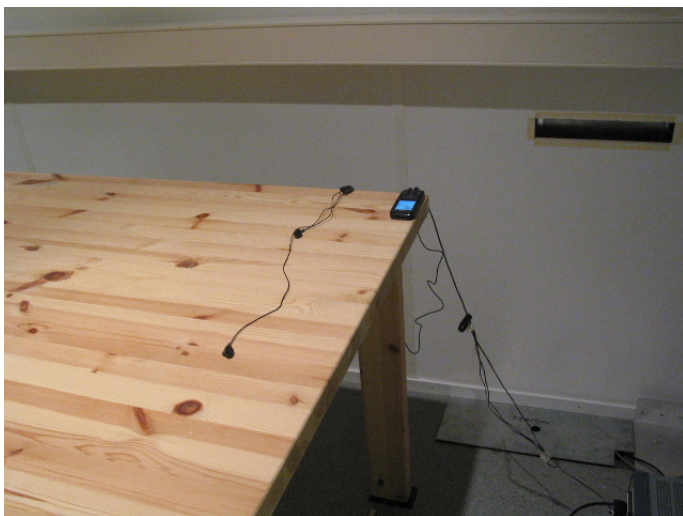
Picture 3 AC powerline conducted emission measurement Bluetooth TX / WLAN TX
