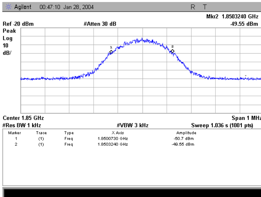
Picture 6: 99% occupied bandwidth, GSM EDGE 8PSK, channel 512
