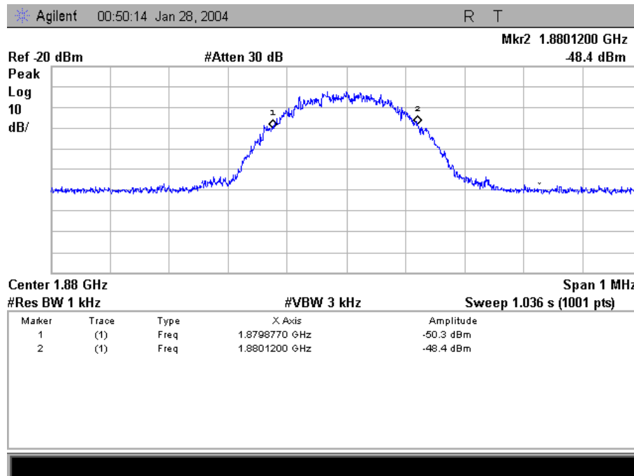
Picture 7: 99% occupied bandwidth, GSM EDGE 8PSK, channel 661
