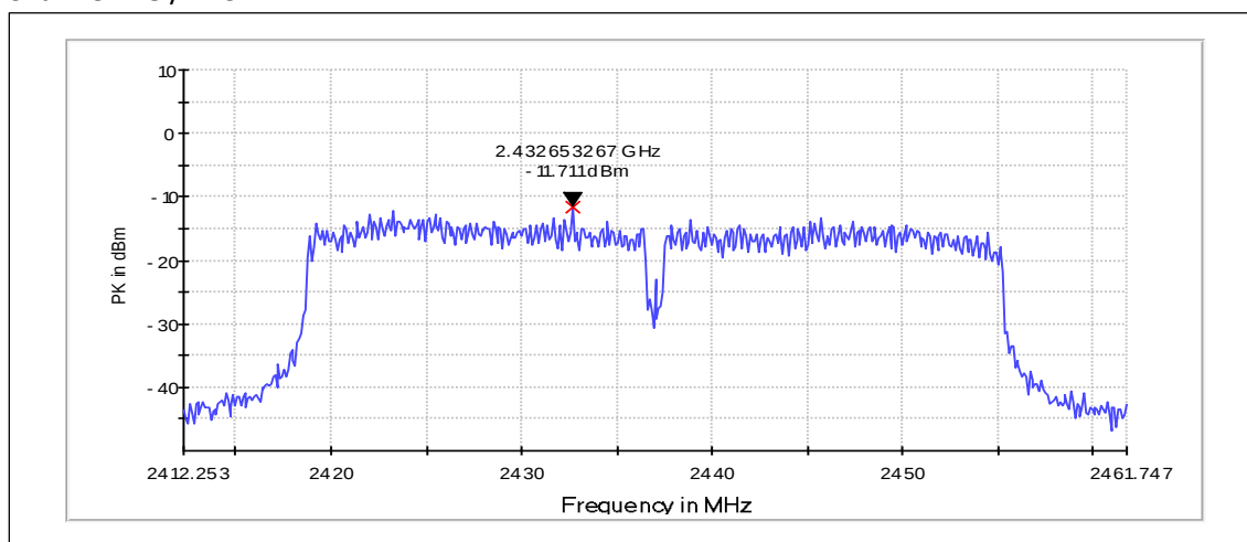
Channel 4-8 / 2437 MHz
