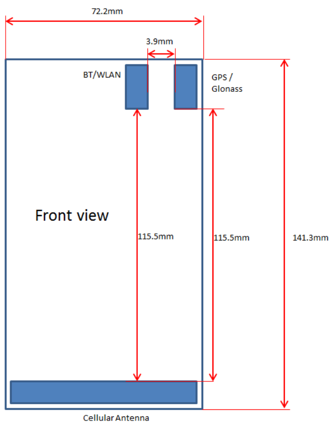
Photo 24: Antenna location
