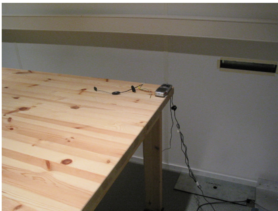
Picture 4 AC powerline conducted emission measurement (WLAN)
