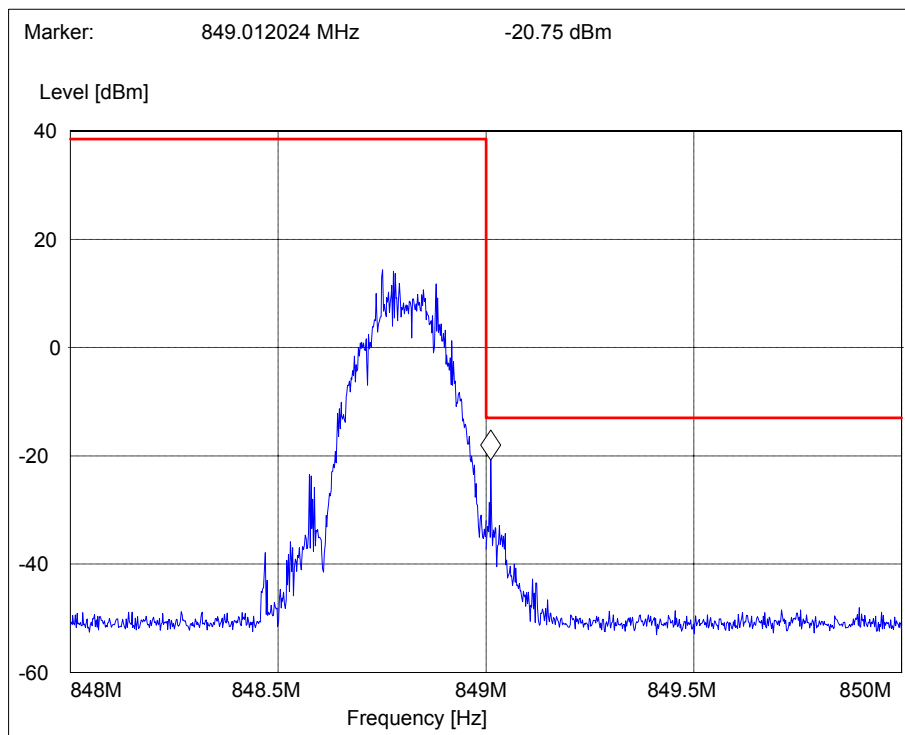
Picture 10 Upper bandedge, EGPRS 850 channel 251, flip open
