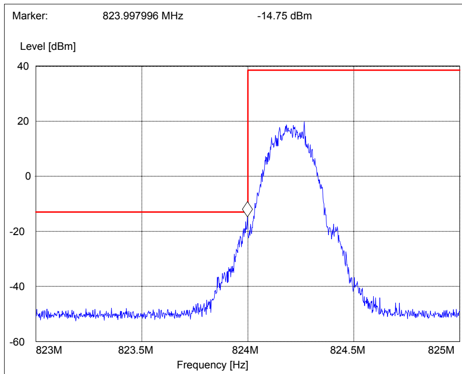
Picture 3 Lower bandedge, GSM 850 channel 128, flip closed
