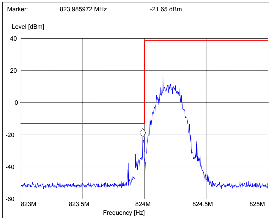
Picture 9 Lower bandedge, EGPRS 850 channel 128, flip open
