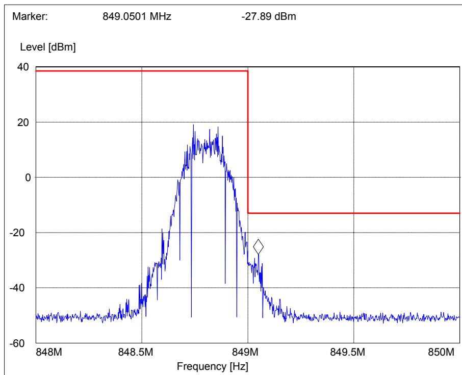
Picture 6 Upper bandedge, EGPRS 850 channel 251, flip closed
