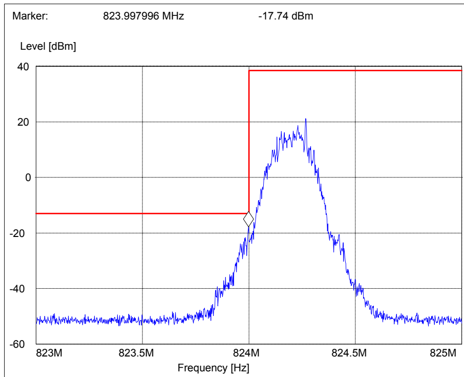
Picture 7 Lower bandedge, GSM 850 channel 128, flip open
