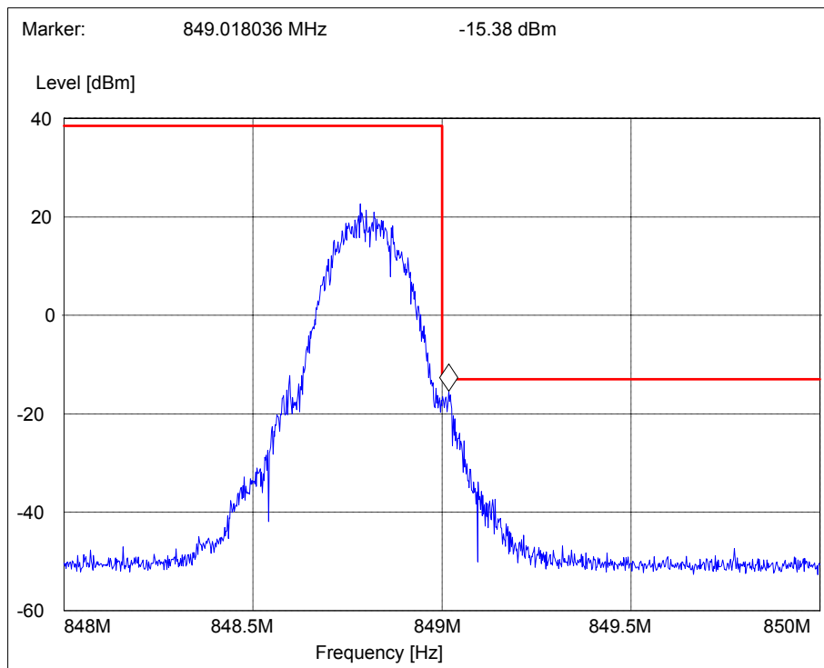
Picture 4 Upper bandedge, GSM 850 channel 251, flip closed
