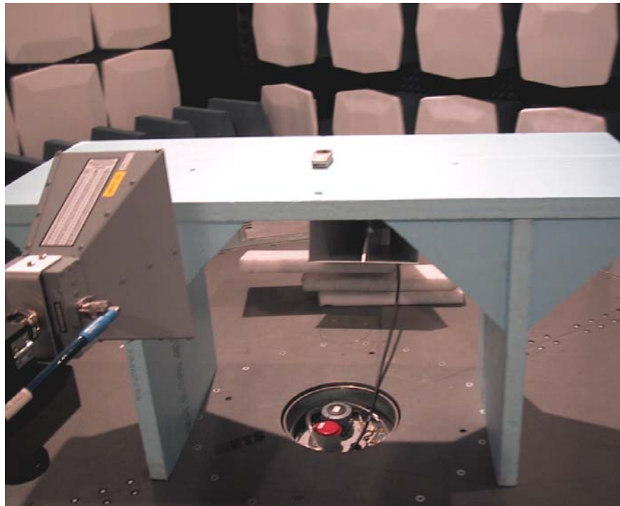
Picture 3: Radiated spurious emission measurement set-up for above 3 GHz measurements, EUT in horizontal orientation
