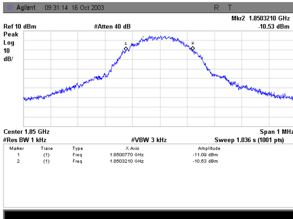
Picture 6: 99% occupied bandwidth, GSM EDGE 8PSK, channel 512
