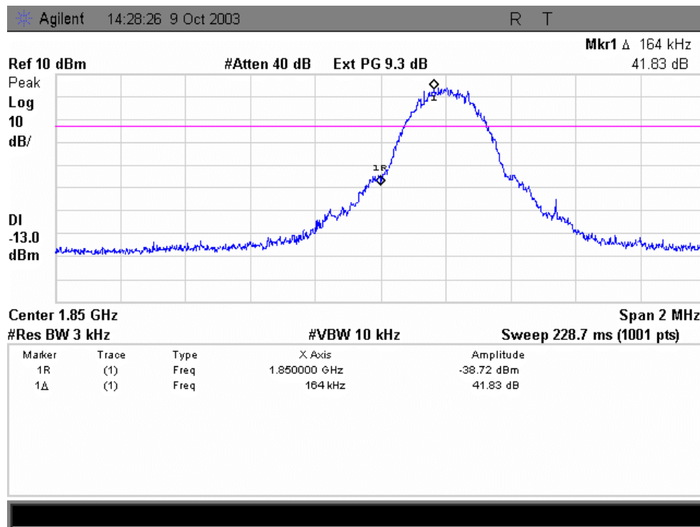
Picture 10: GSM GMSK, channel 512
