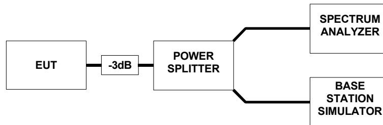
Picture 2: Test setup for 99% occupied bandwidth measurement
