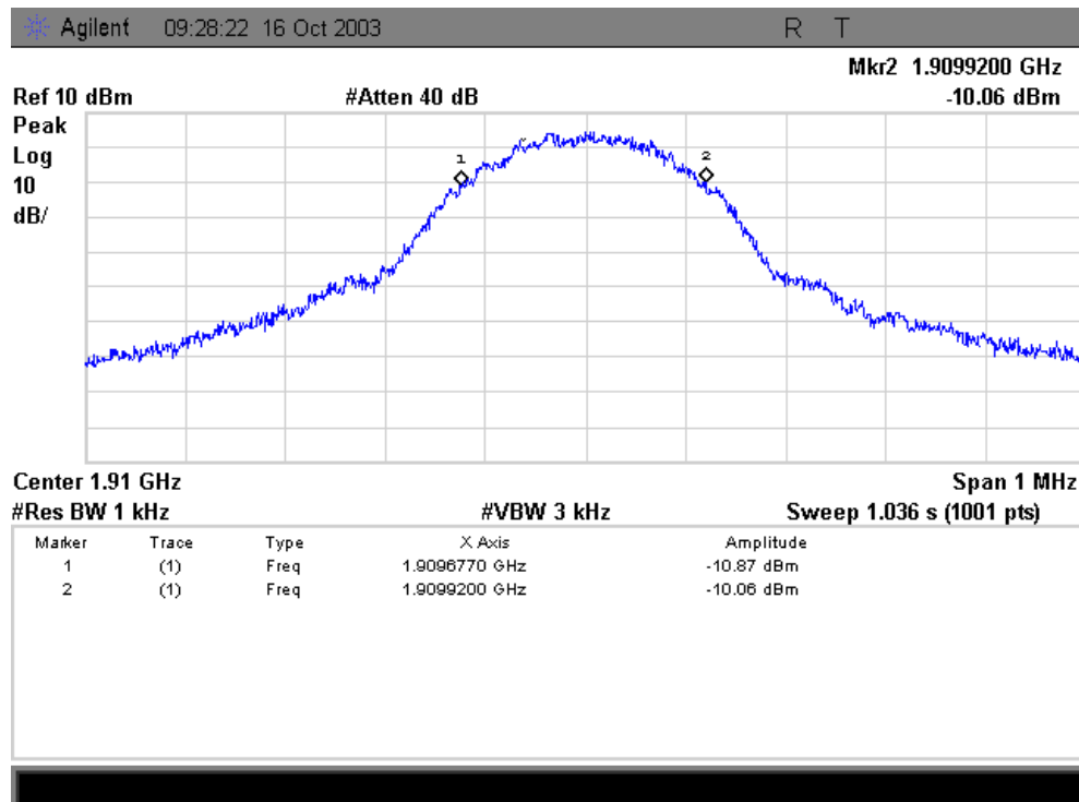
Picture 8: 99% occupied bandwidth, GSM EDGE 8PSK, channel 810
