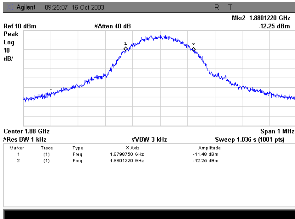
Picture 7: 99% occupied bandwidth, GSM EDGE 8PSK, channel 661
