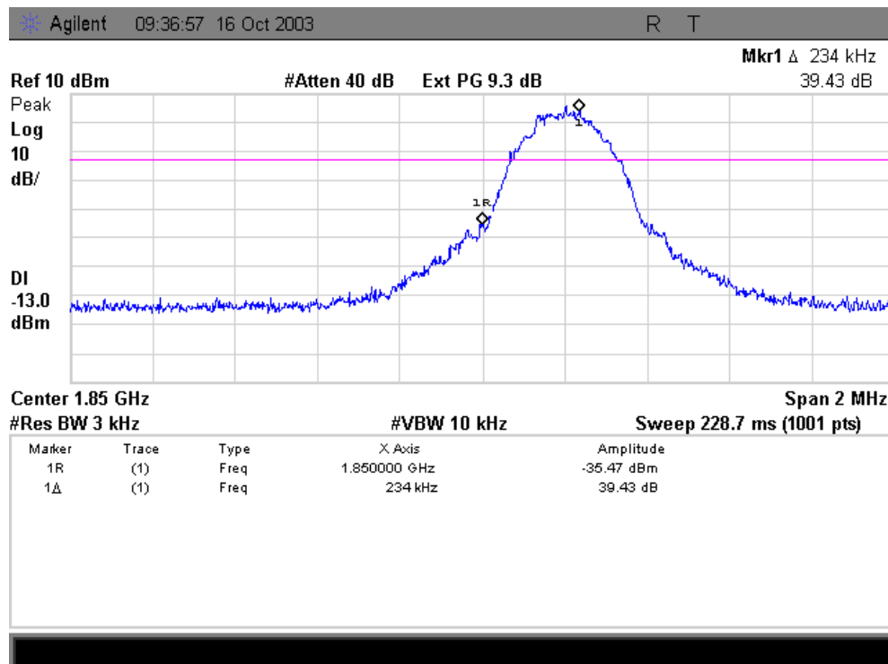
Picture 12: GSM EDGE 8PSK, channel 512
