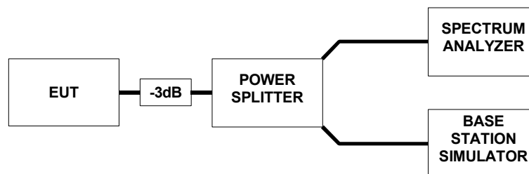
Picture 9: Test setup for block edge compliance measurement
