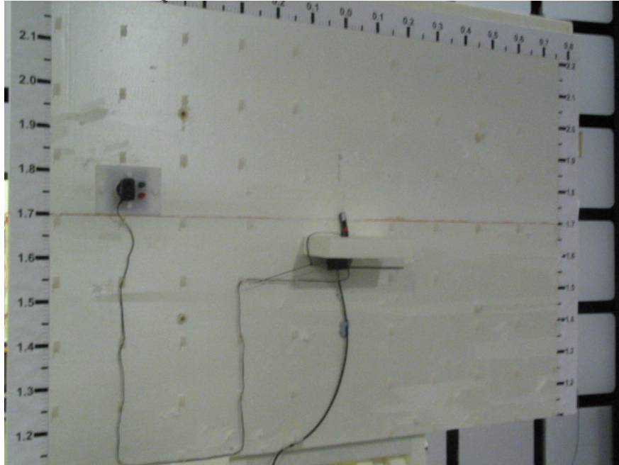
Picture 1 Spurious radiated emission measurement Bluetooth TX
