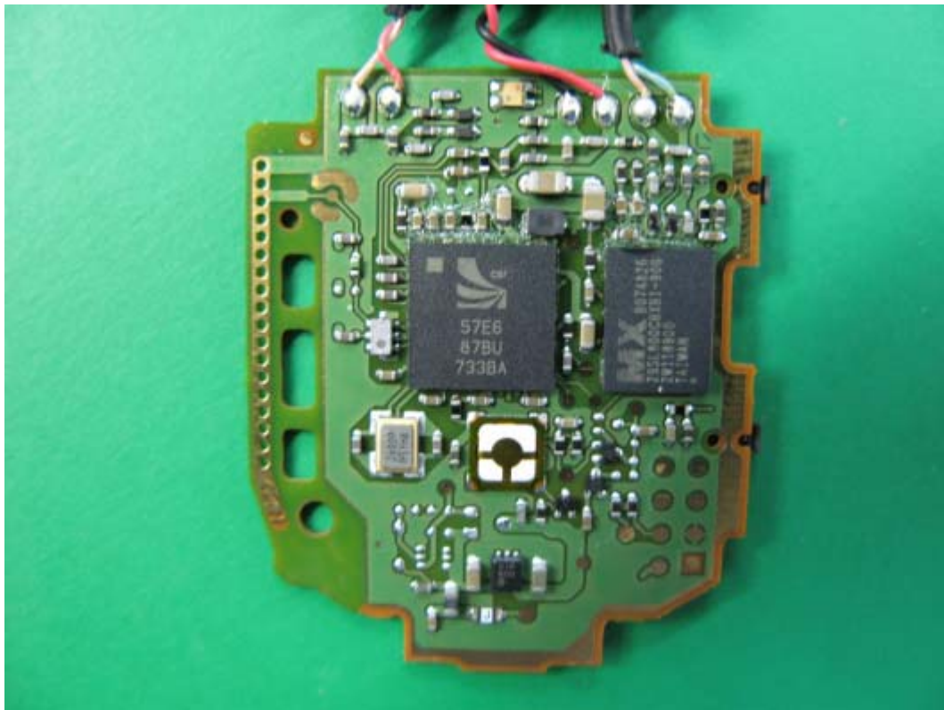
<Top side of PCB>
