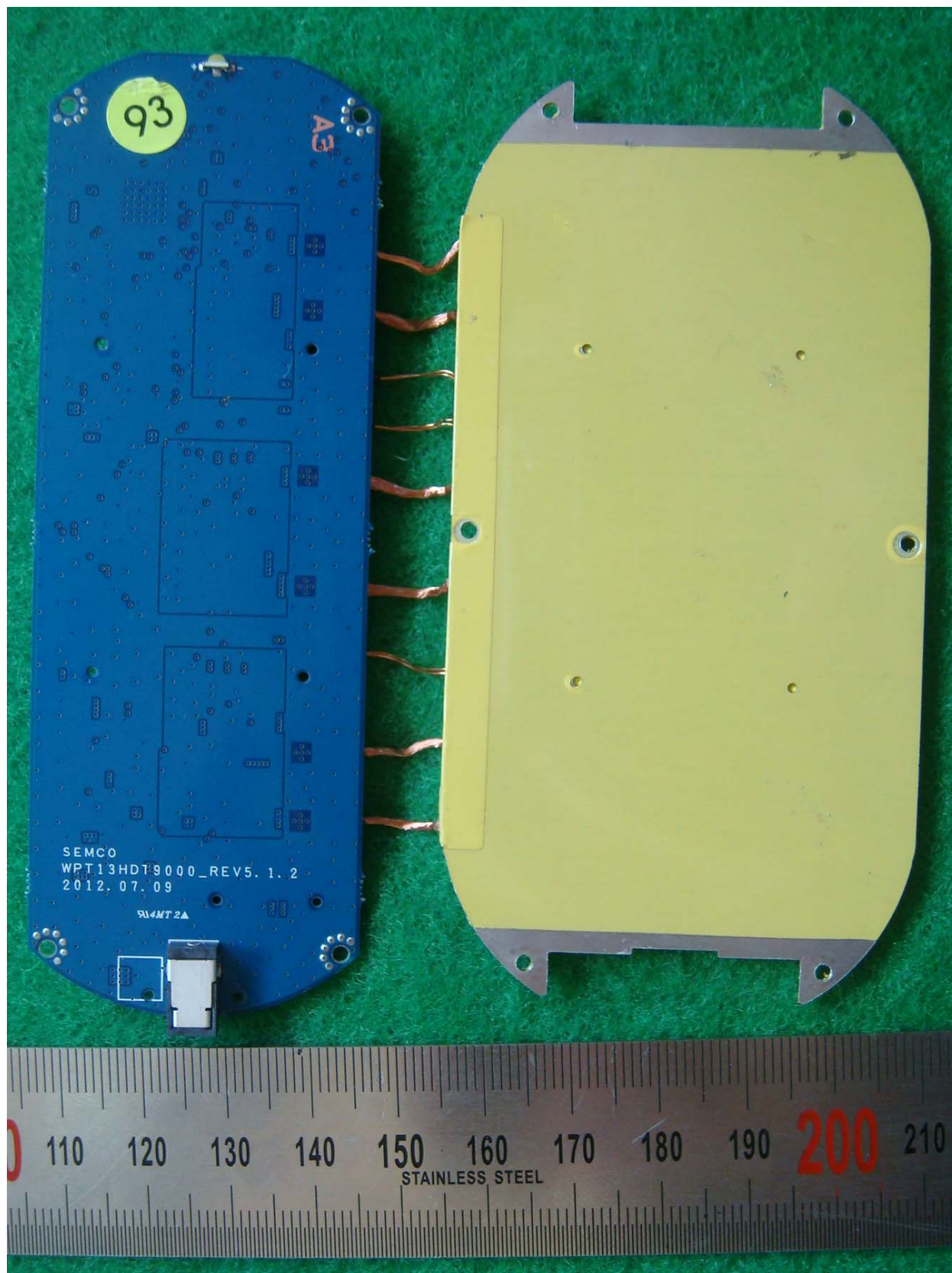
&lt;Photograph 3: Main board &amp; Antenna - Rear view&gt;
