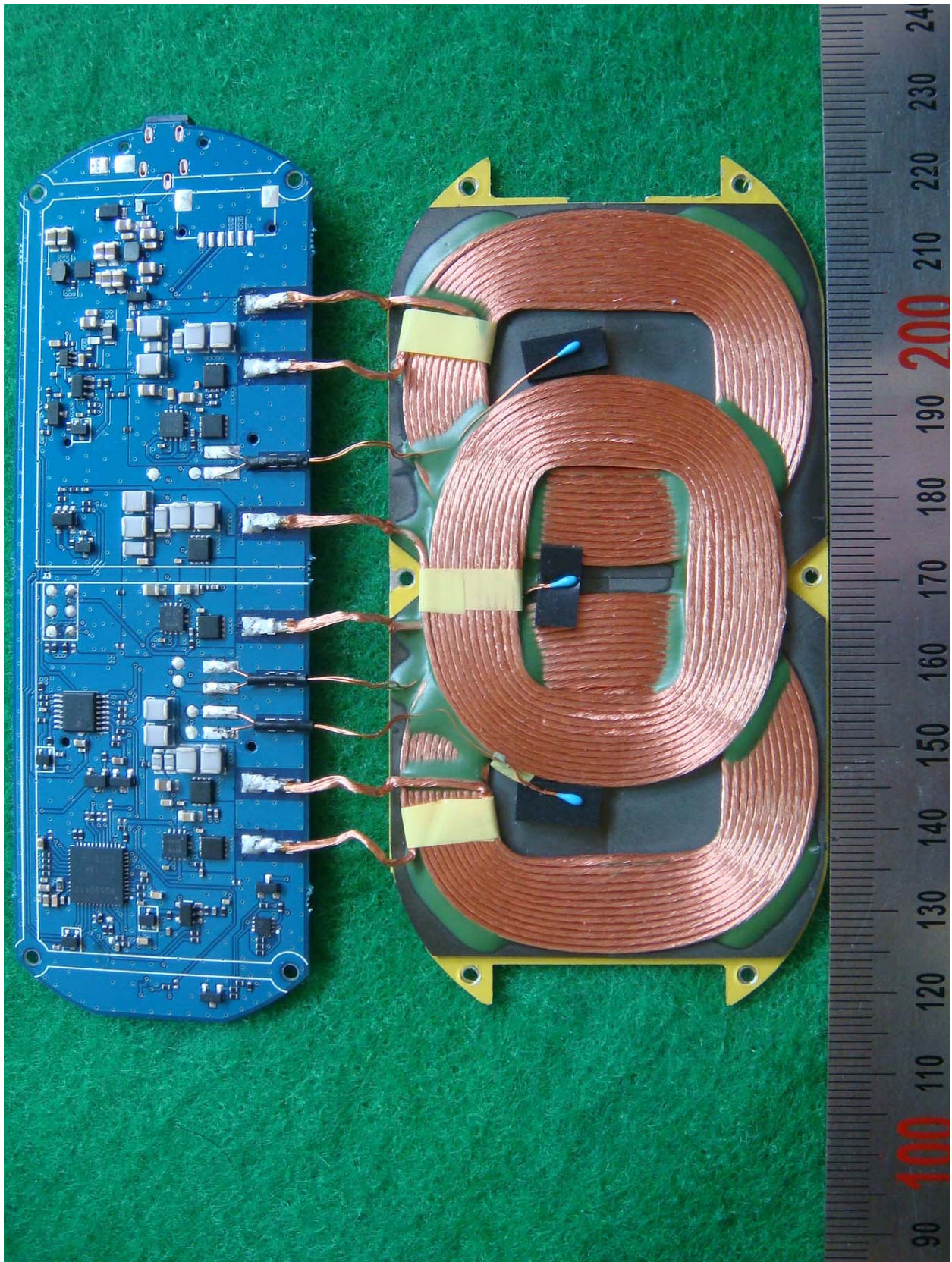
&lt;Photograph 2: Main board &amp; Antenna- Front view&gt;
