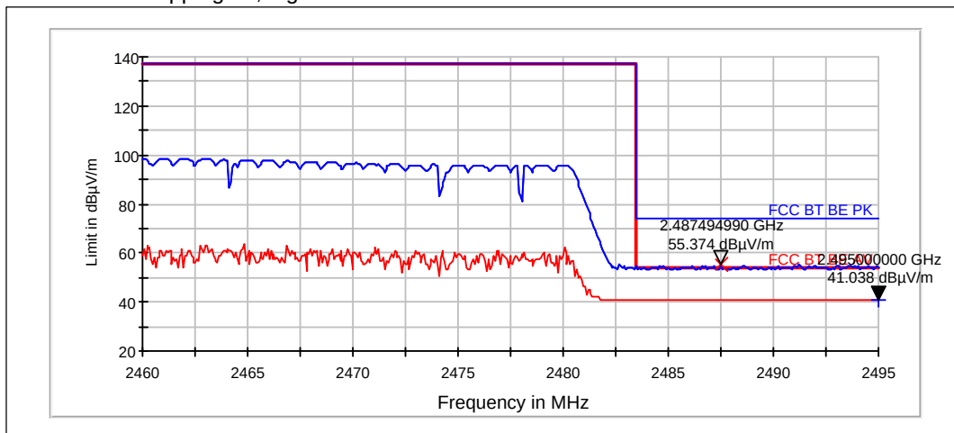
GFSK mode. Hopping on, high end
