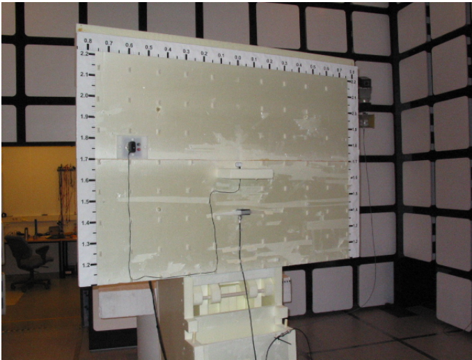
Picture 1 Spurious radiated emission measurement Bluetooth TX
