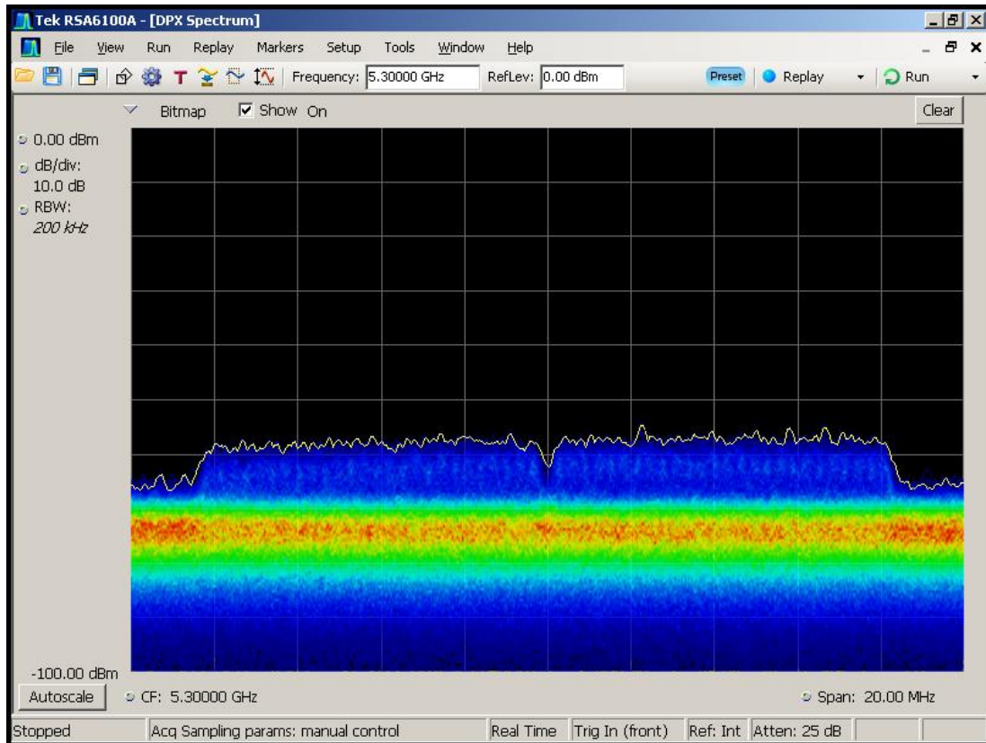
Figure 5-3. Real-Time Spectrum Display, WLAN Traffic (Streaming Video)
