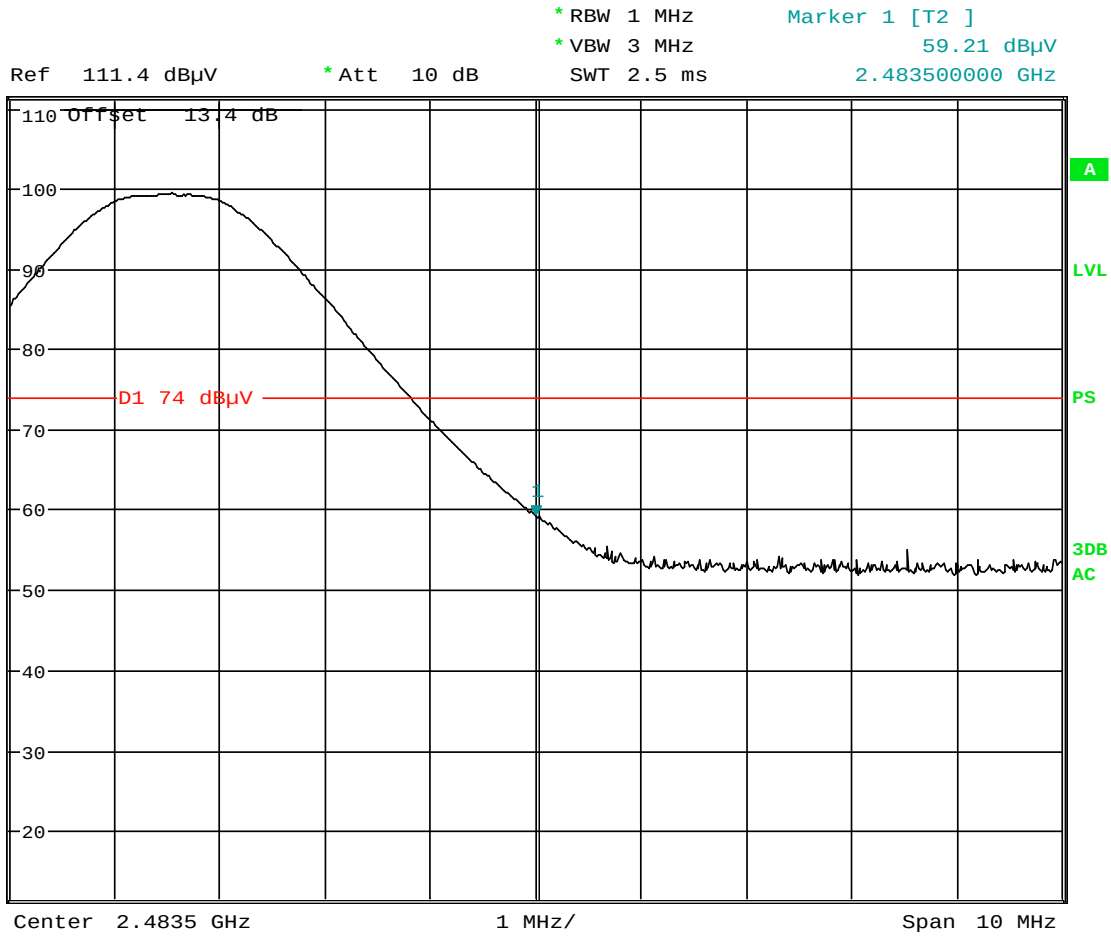
Plot 6-19. Radiated Restricted Band Edge Plot (Peak)
