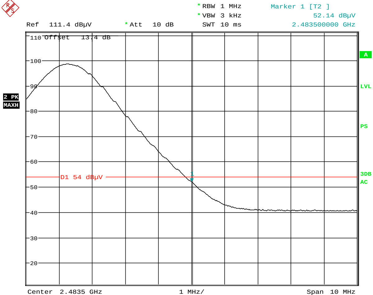
Plot 6-18.Radiated Restricted Band Edge Plot (Average)
