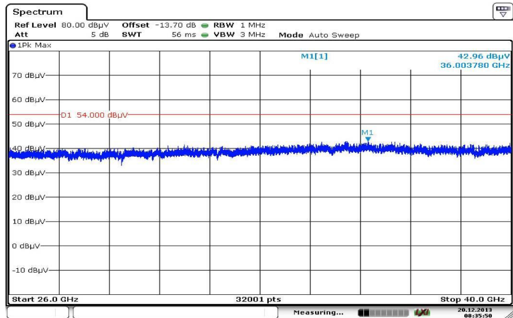
Plot 6: Receiver mode 26 GHz to 40 GHz
