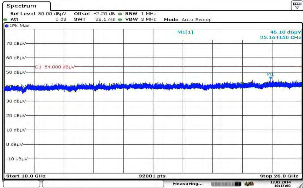
Plot 9: 18 GHz to 26 GHz, 5290 MHz, vertical & horizontal polarization
