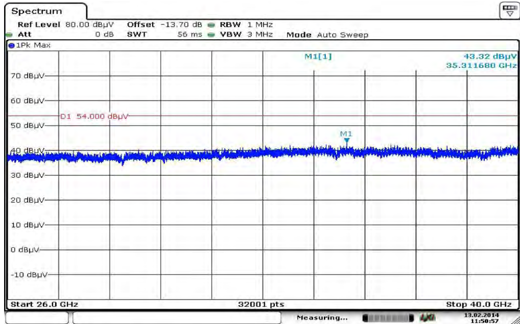
Plot 15: 26 GHz to 40 GHz, 5530 MHz, vertical & horizontal polarization
