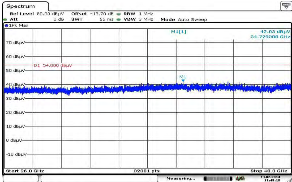
Plot 10: 26 GHz to 40 GHz, 5290 MHz, vertical & horizontal polarization
