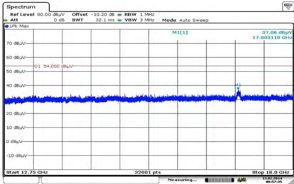
Plot 28: 12 GHz to 18 GHz, 5670 MHz, vertical & horizontal polarization
