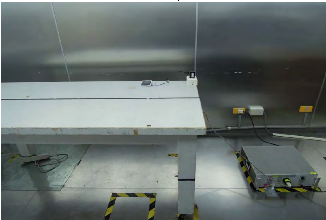
AC Power-line Conducted Emission Set up Photo (Adapter Model number: EP800)
