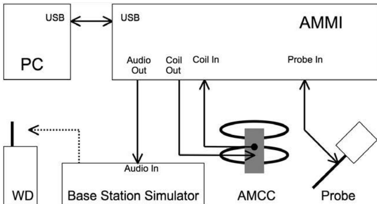
Fig. 5.5 T-Coil setup cabling
