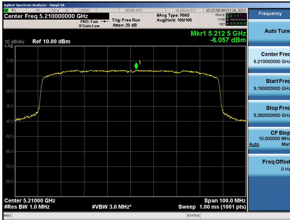
Plot 6-41. Peak Power Spectral Density Plot (80MHz BW 802.11ac (UNII Band 1) – Ch. 42)
