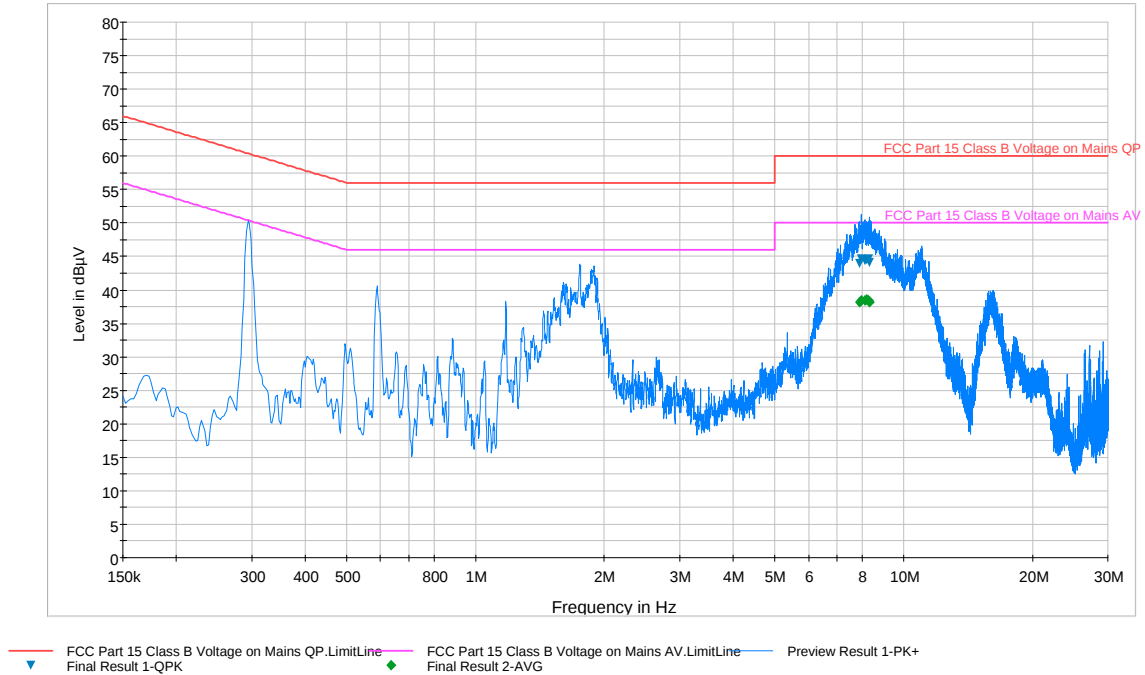
Plot 6-91. Line Conducted Plot with 802.11a UNII Band 3 (N)
