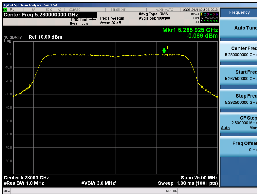
Plot 6-46. Peak Power Spectral Density Plot (20MHz BW 802.11n (UNII Band 2) – Ch. 56)
