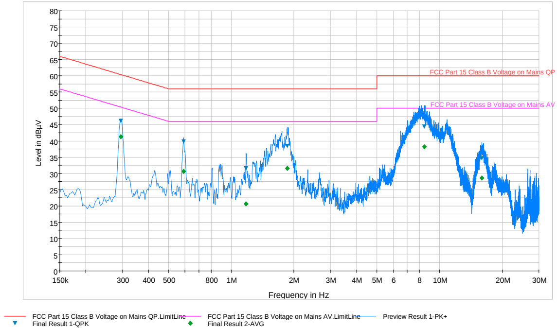
Plot 6-90. Line Conducted Plot with 802.11a UNII Band 3 (L1)
