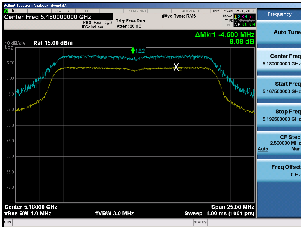
Plot 6-61. Peak Excursion Ratio Plot (802.11a)
