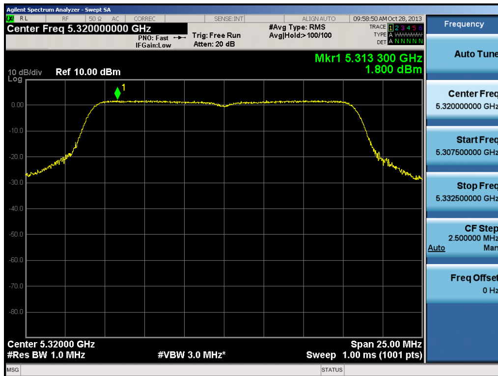
Plot 6-44. Peak Power Spectral Density Plot (802.11a (UNII Band 2) – Ch. 64)
