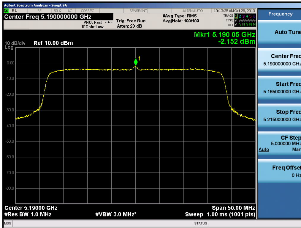
Plot 6-39. Peak Power Spectral Density Plot (40MHz BW 802.11n (UNII Band 1) – Ch. 38)
