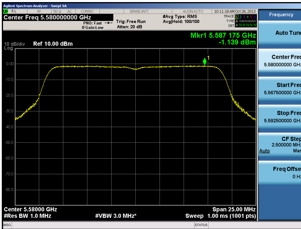
Plot 6-55. Peak Power Spectral Density Plot (20MHz BW 802.11n (UNII Band 3) – Ch. 116)
