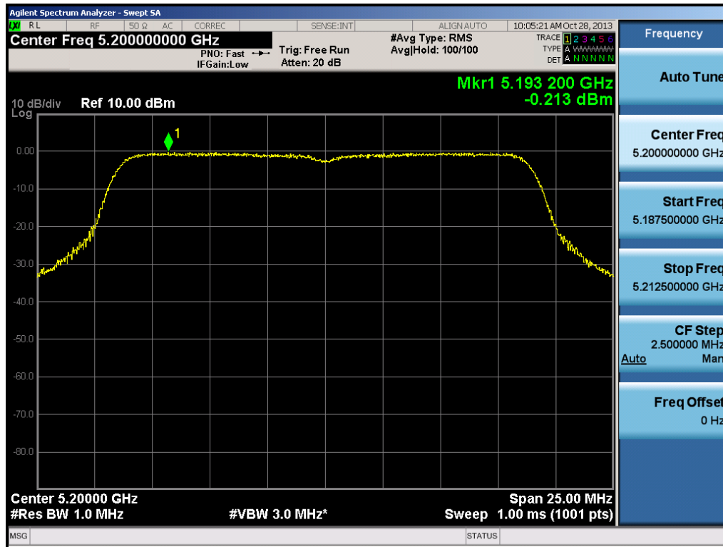
Plot 6-37. Peak Power Spectral Density Plot (20MHz BW 802.11n (UNII Band 1) – Ch. 40)
