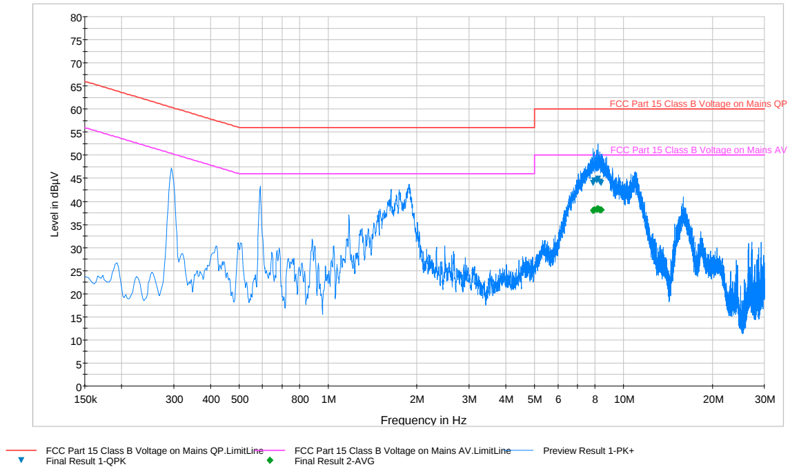
Plot 6-89. Line Conducted Plot with 802.11a UNII Band 2 (N)
