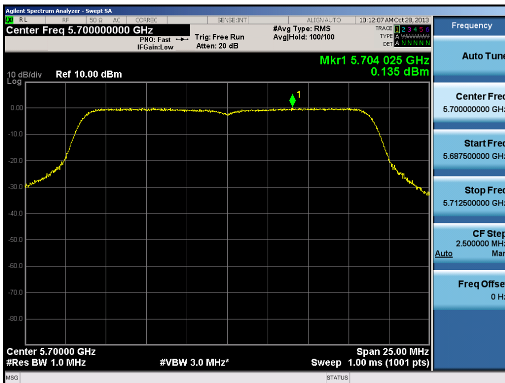
Plot 6-56. Peak Power Spectral Density Plot (20MHz BW 802.11n (UNII Band 3) – Ch. 140)
