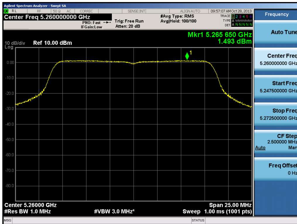
Plot 6-42. Peak Power Spectral Density Plot (802.11a (UNII Band 2) – Ch. 52)
