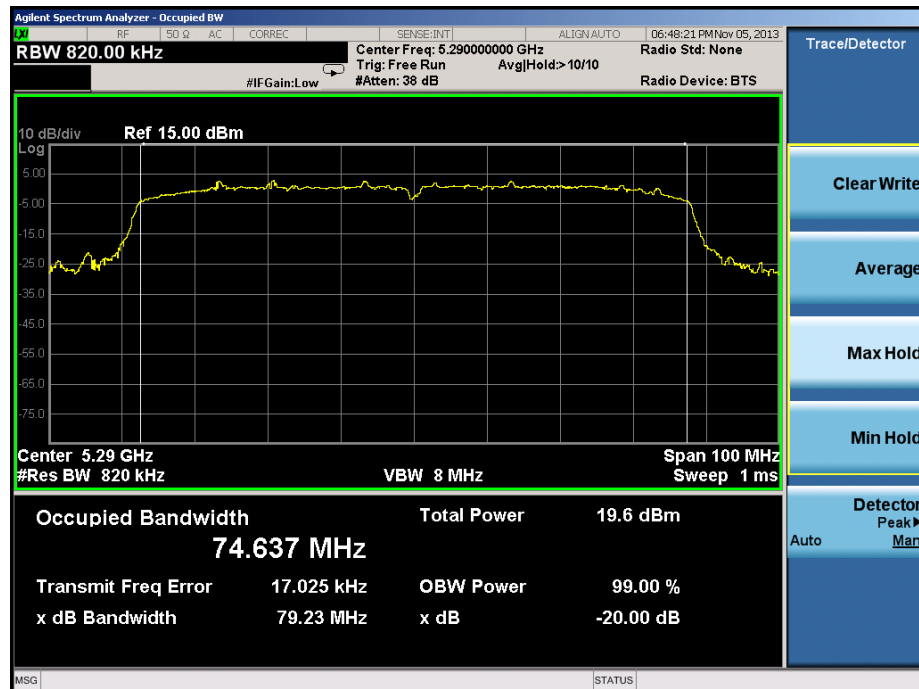
Plot 6-32. 20dB Bandwidth Plot (80MHz BW 802.11n (UNII Band 2) – Ch. 58)
