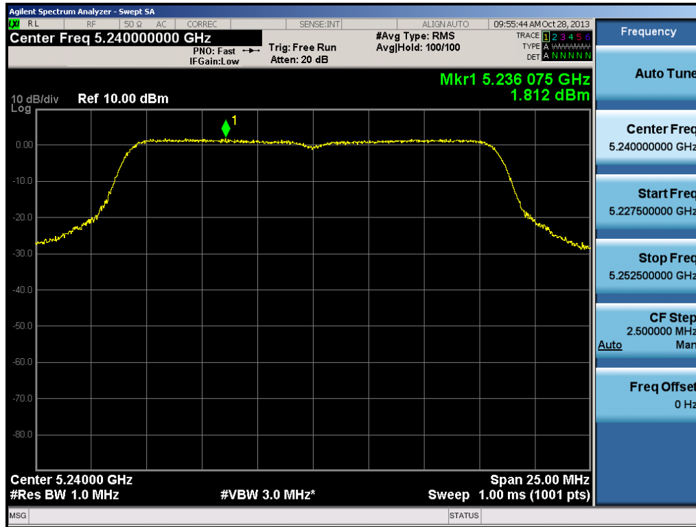
Plot 6-35. Peak Power Spectral Density Plot (802.11a (UNII Band 1) – Ch. 48)
