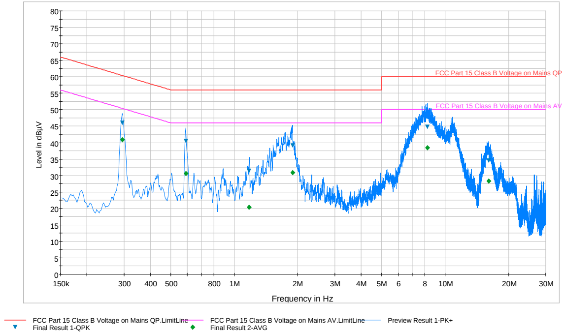
Plot 6-88. Line Conducted Plot with 802.11a UNII Band 2 (L1)
