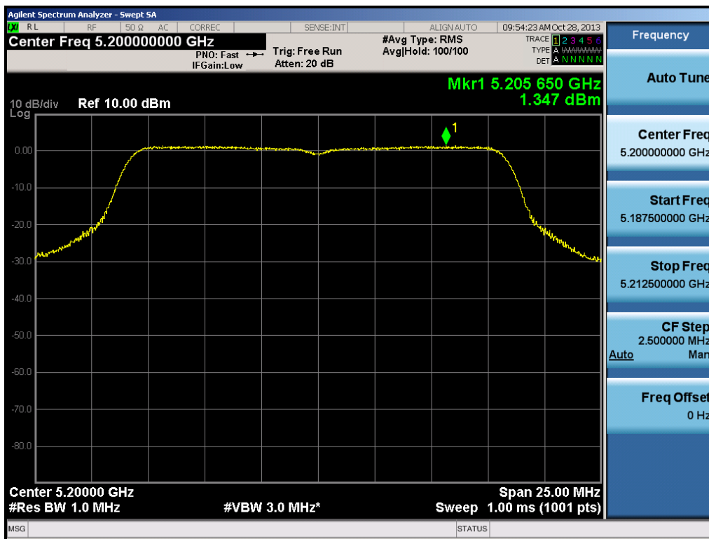
Plot 6-34. Peak Power Spectral Density Plot (802.11a (UNII Band 1) – Ch. 40)
