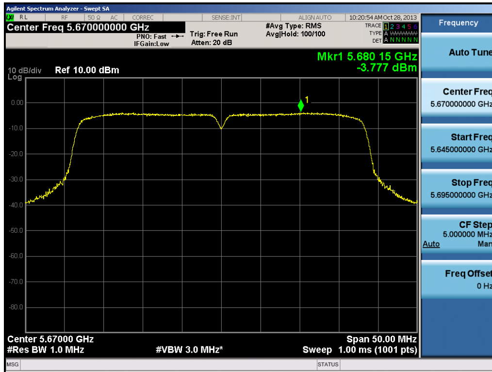
Plot 6-59. Peak Power Spectral Density Plot (40MHz BW 802.11n (UNII Band 3) – Ch. 134)
