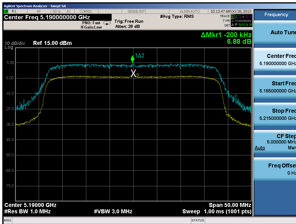
Plot 6-63. Peak Excursion Ratio Plot (40MHz BW 802.11n)
