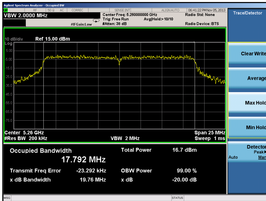
Plot 6-30. 20dB Bandwidth Plot (20MHz BW 802.11n (UNII Band 2) – Ch. 52)
