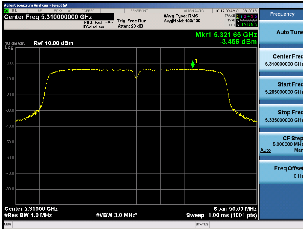
Plot 6-49. Peak Power Spectral Density Plot (40MHz BW 802.11n (UNII Band 2) – Ch. 62)
