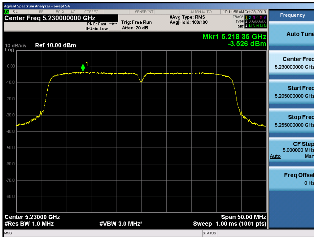
Plot 6-40. Peak Power Spectral Density Plot (40MHz BW 802.11n (UNII Band 1) – Ch. 46)
