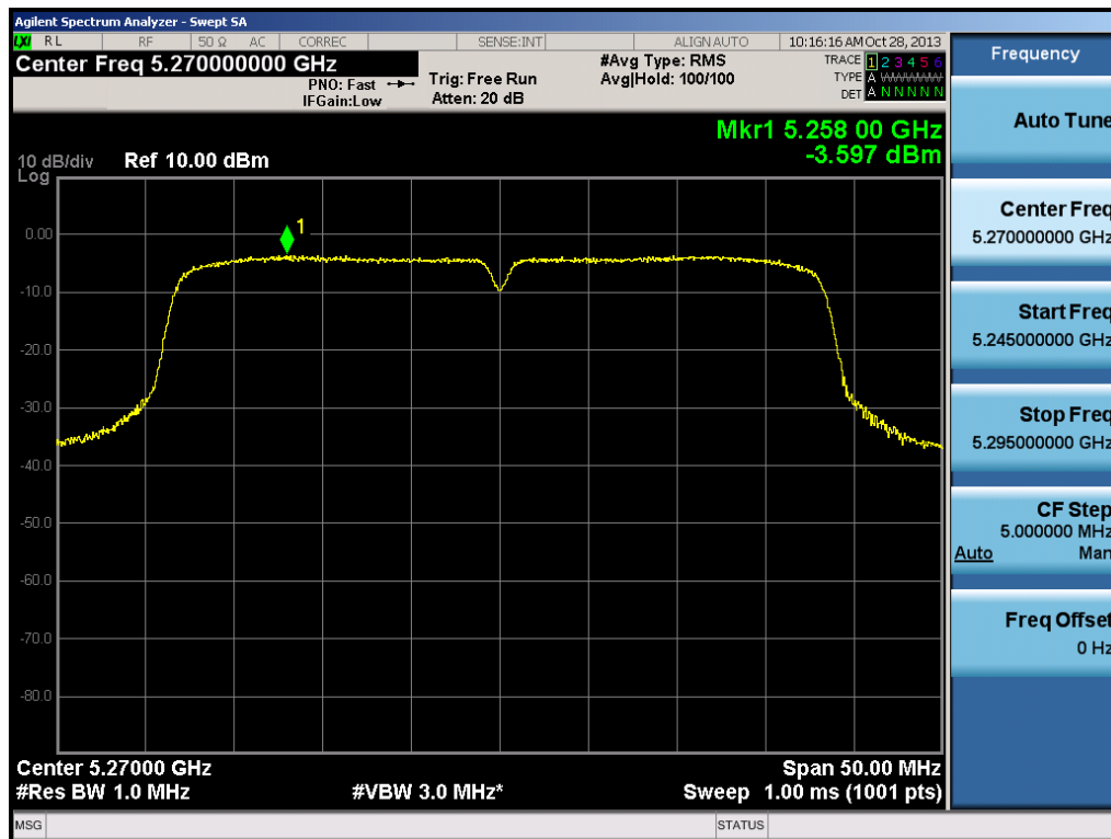
Plot 6-48. Peak Power Spectral Density Plot (40MHz BW 802.11n (UNII Band 2) – Ch. 54)
