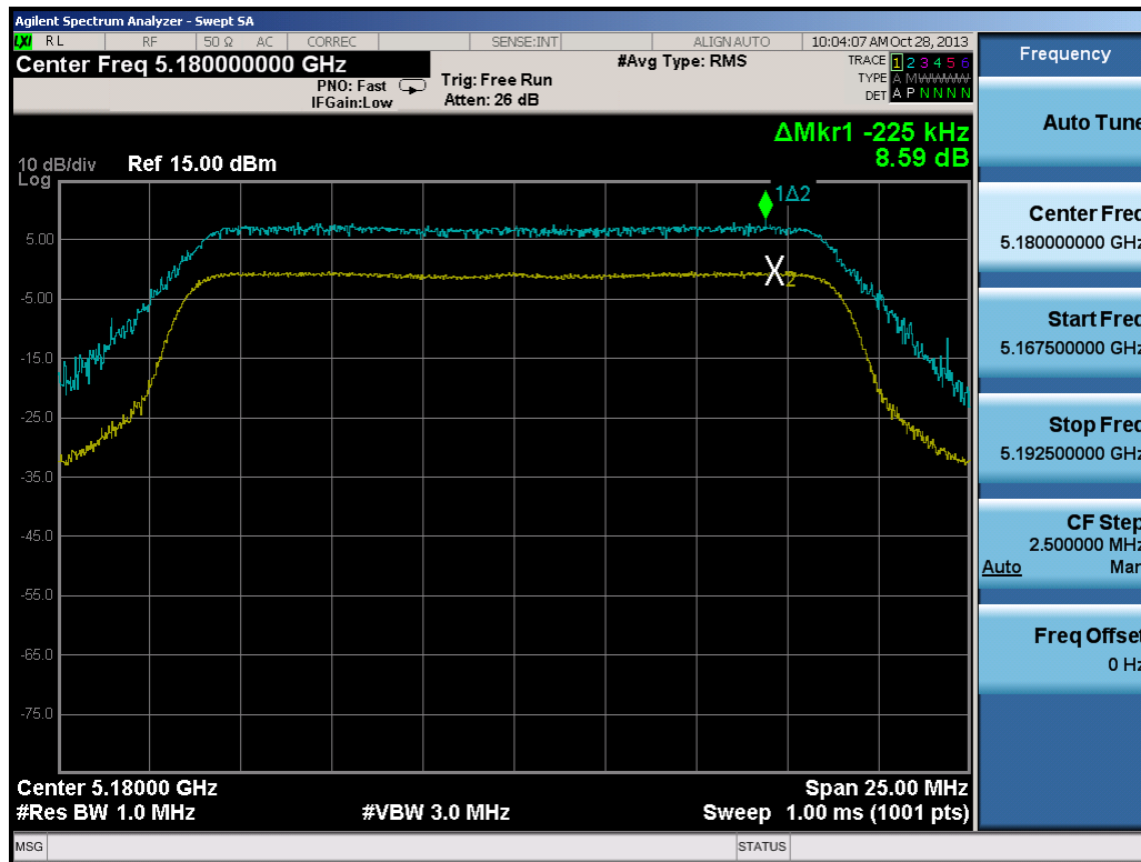
Plot 6-62. Peak Excursion Ratio Plot (20MHz BW 802.11n)
