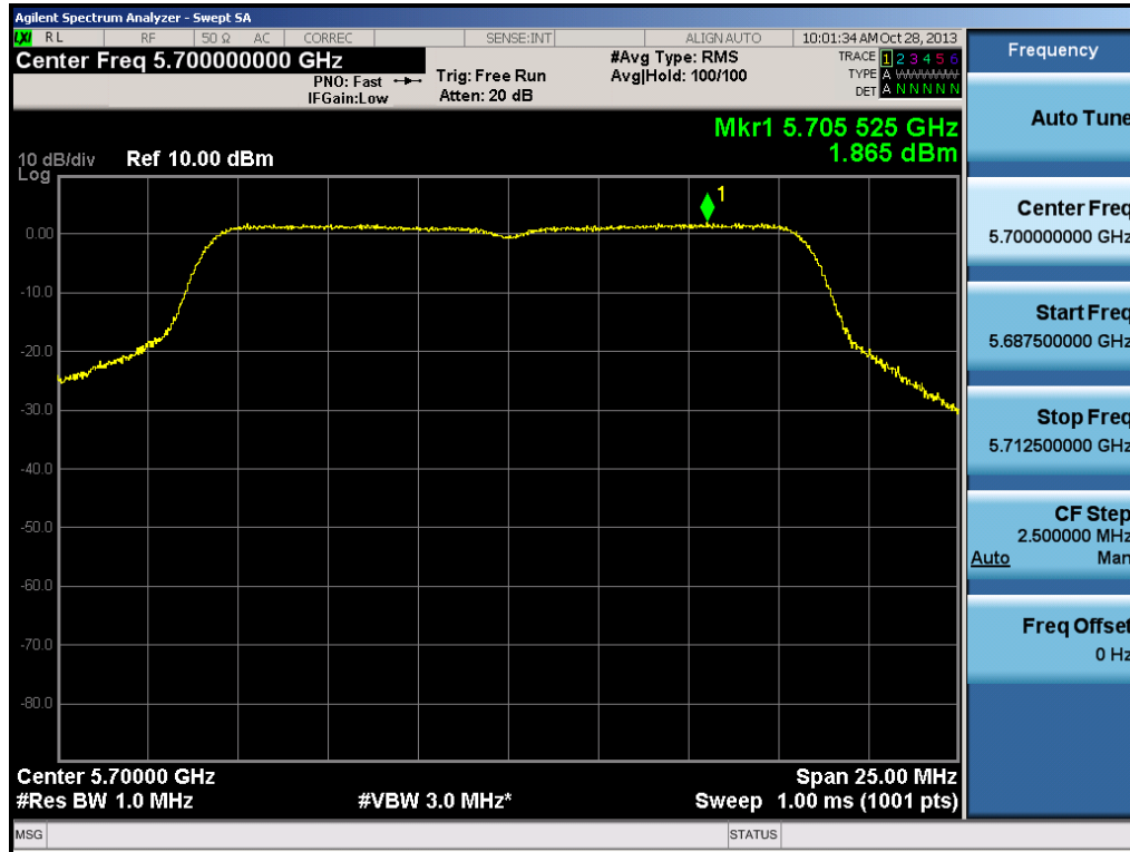
Plot 6-53. Peak Power Spectral Density Plot (802.11a (UNII Band 3) – Ch. 140)
