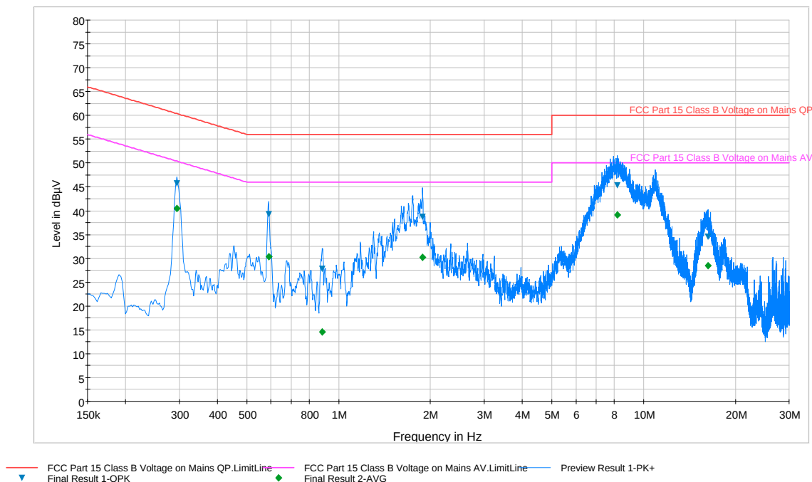
Plot 6-86. Line Conducted Plot with 802.11a UNII Band 1 (L1)
