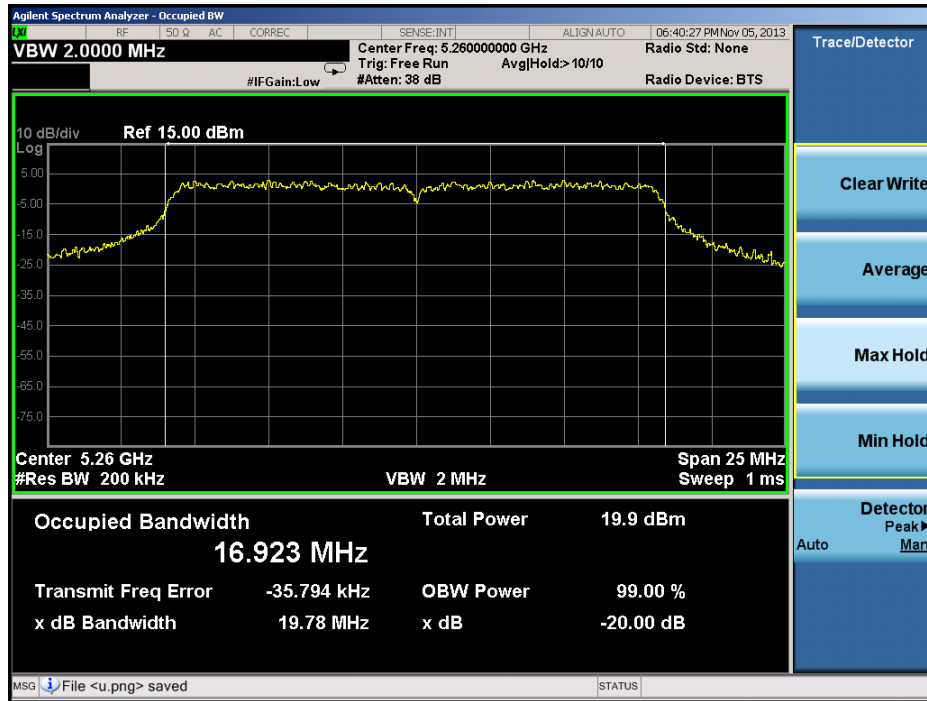
Plot 6-29. 20dB Bandwidth Plot (20MHz BW 802.11a (UNII Band 2) – Ch. 52)
