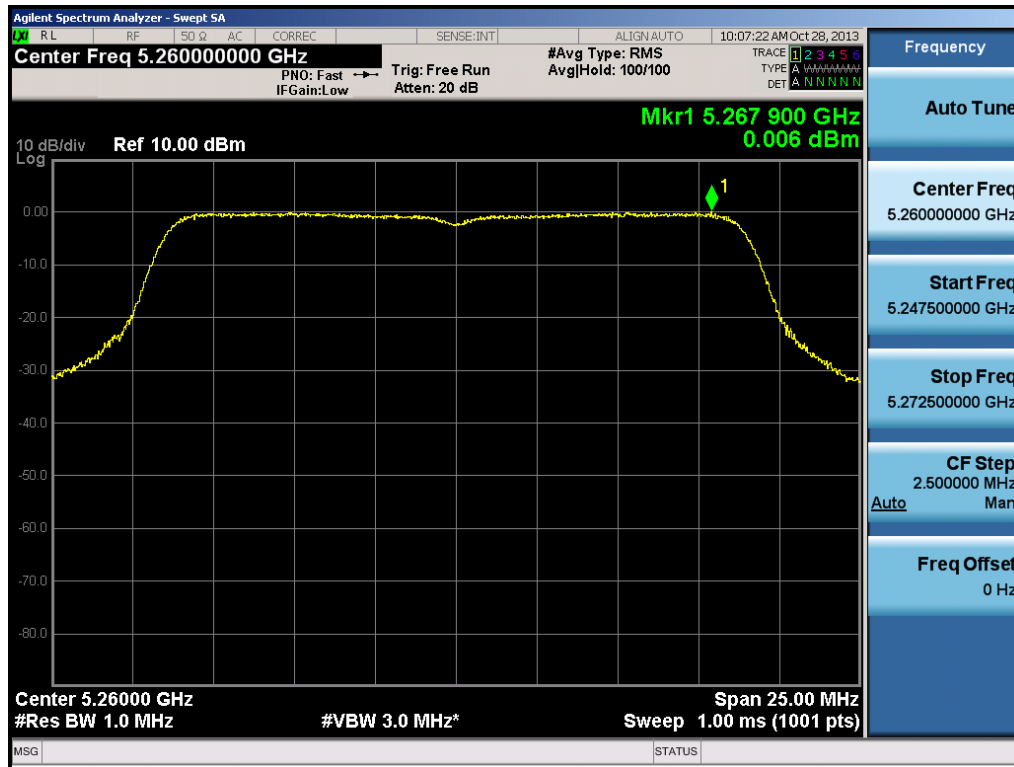
Plot 6-45. Peak Power Spectral Density Plot (20MHz BW 802.11n (UNII Band 2) – Ch. 52)
