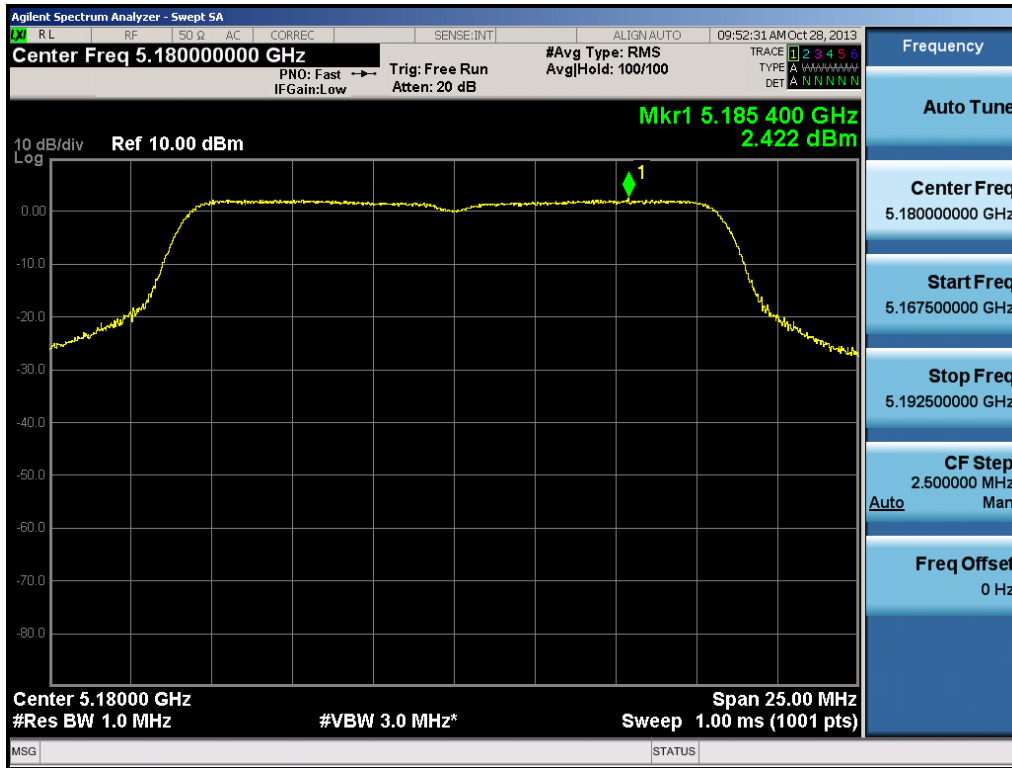
Plot 6-33. Peak Power Spectral Density Plot (802.11a (UNII Band 1) – Ch. 36)
