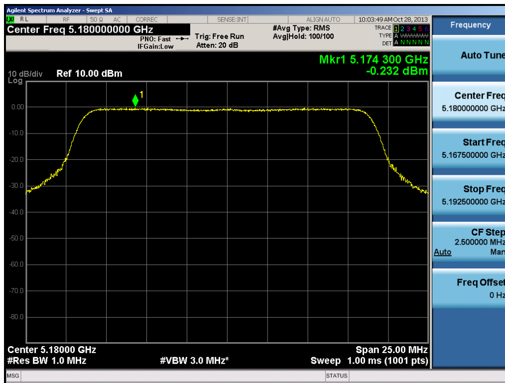
Plot 6-36. Peak Power Spectral Density Plot (20MHz BW 802.11n (UNII Band 1) – Ch. 36)
