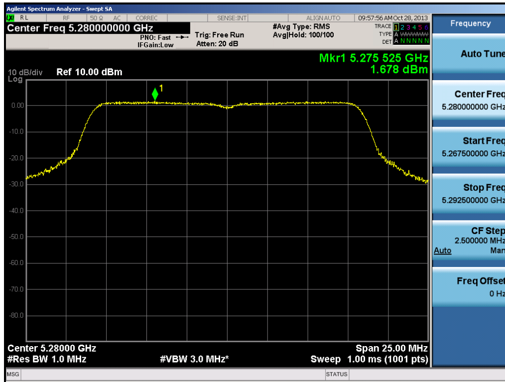
Plot 6-43. Peak Power Spectral Density Plot (802.11a (UNII Band 2) – Ch. 56)
