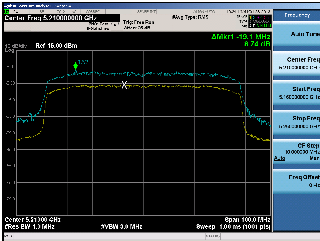
Plot 6-64. Peak Excursion Ratio Plot (80MHz BW 802.11ac)
