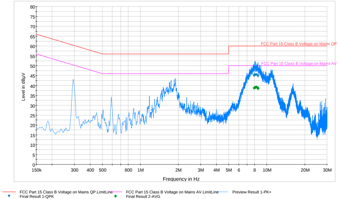
Plot 6-87. Line Conducted Plot with 802.11a UNII Band 1 (N)
