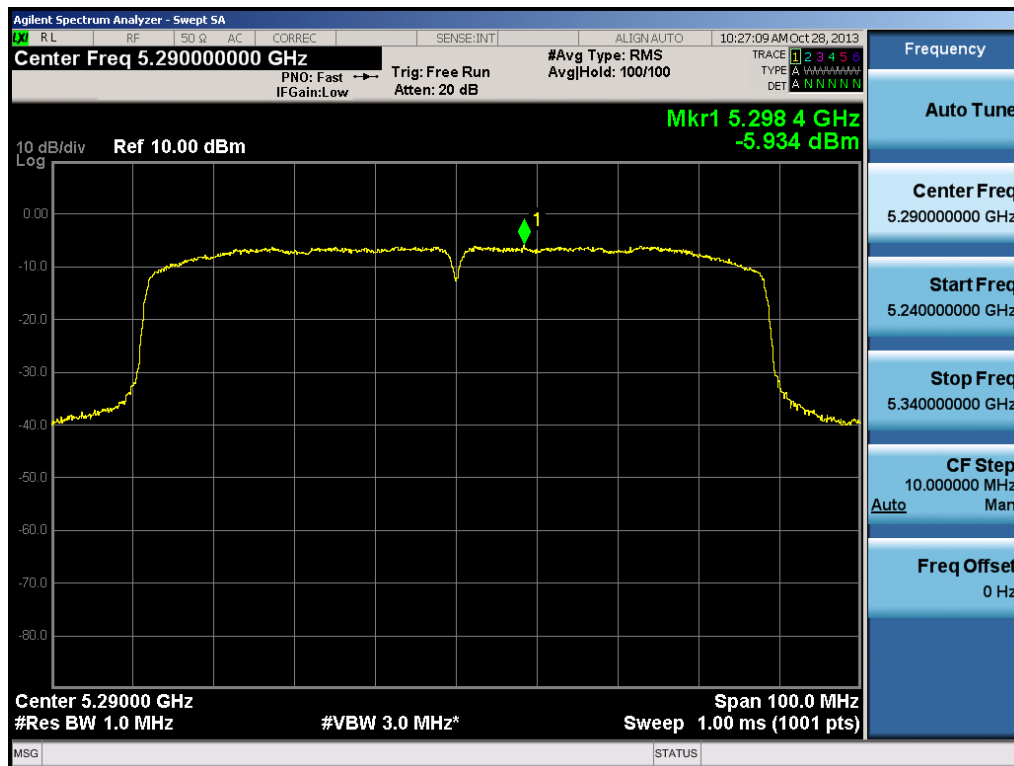
Plot 6-50. Peak Power Spectral Density Plot (80MHz BW 802.11ac (UNII Band 2) – Ch. 58)
