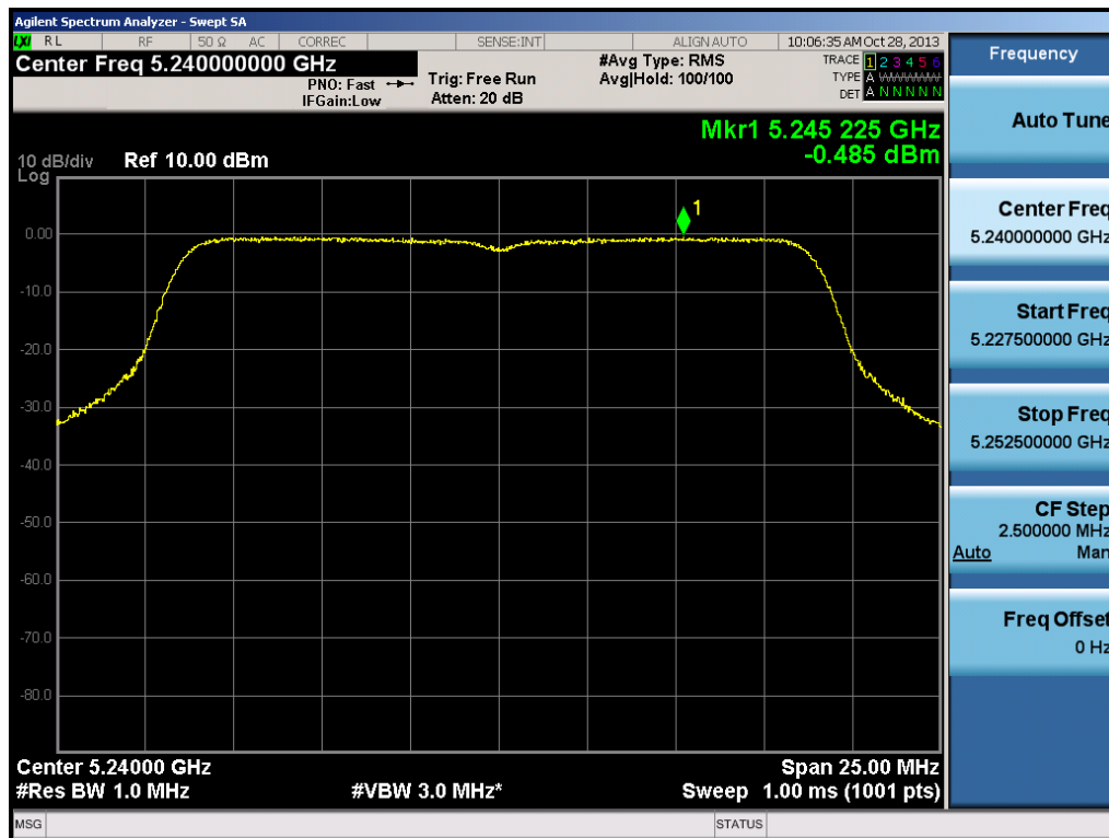
Plot 6-38. Peak Power Spectral Density Plot (20MHz BW 802.11n (UNII Band 1) – Ch. 48)
