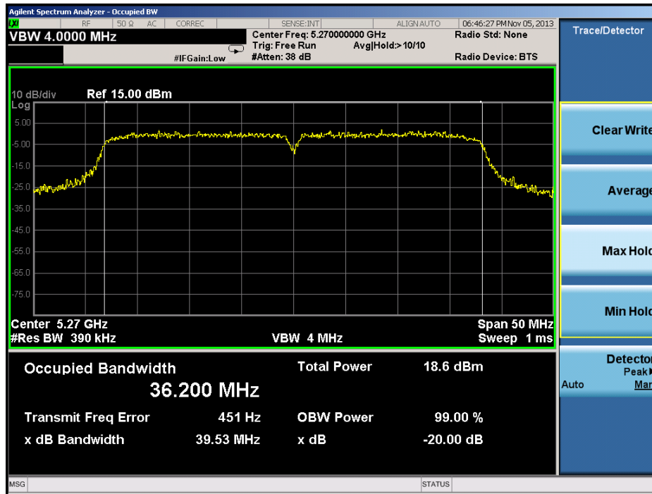
Plot 6-31. 20dB Bandwidth Plot (40MHz BW 802.11n (UNII Band 2) – Ch. 54)
