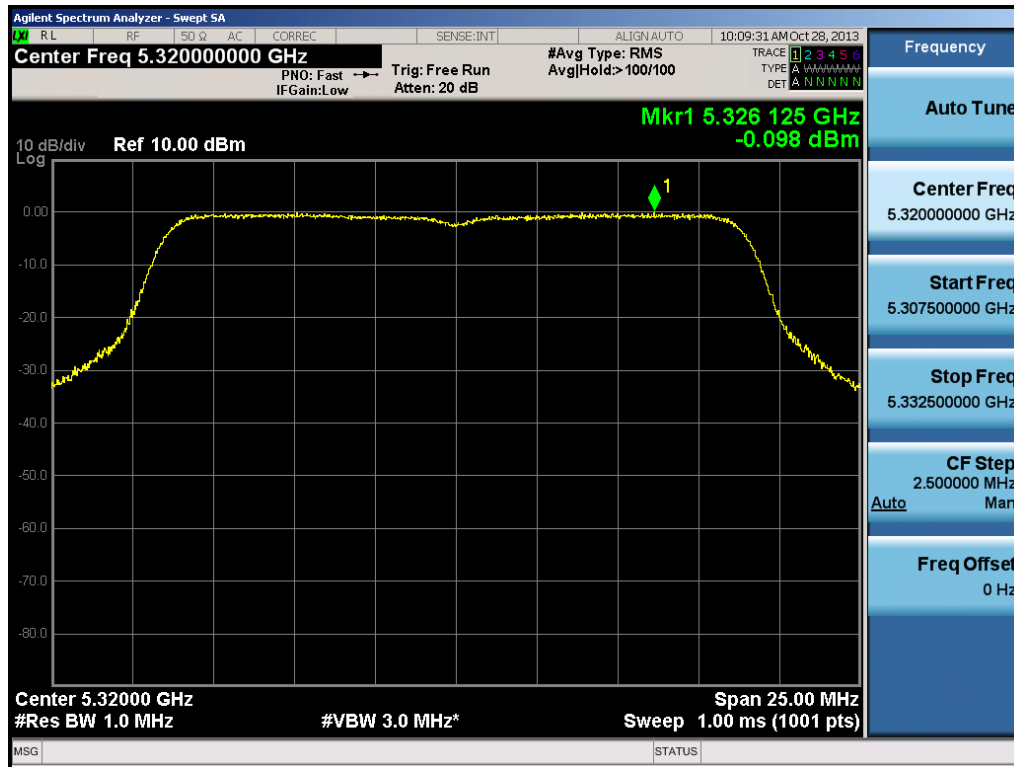
Plot 6-47. Peak Power Spectral Density Plot (20MHz BW 802.11n (UNII Band 2) – Ch. 64)
