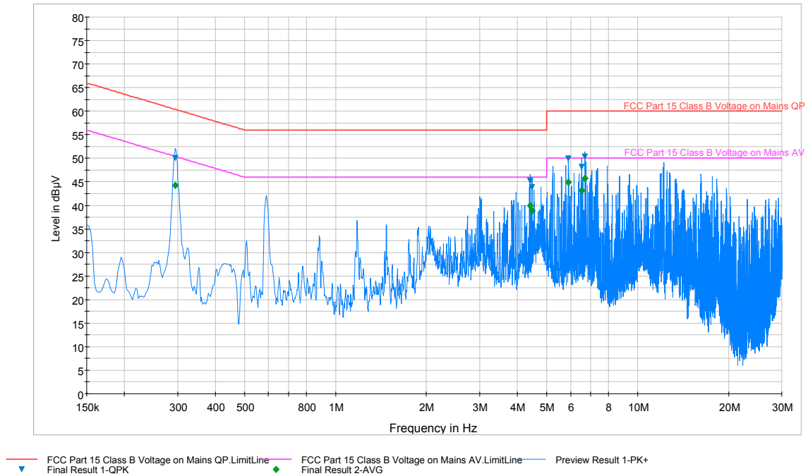
Plot 6-73. Line Conducted Plot with 802.11a (L1)
