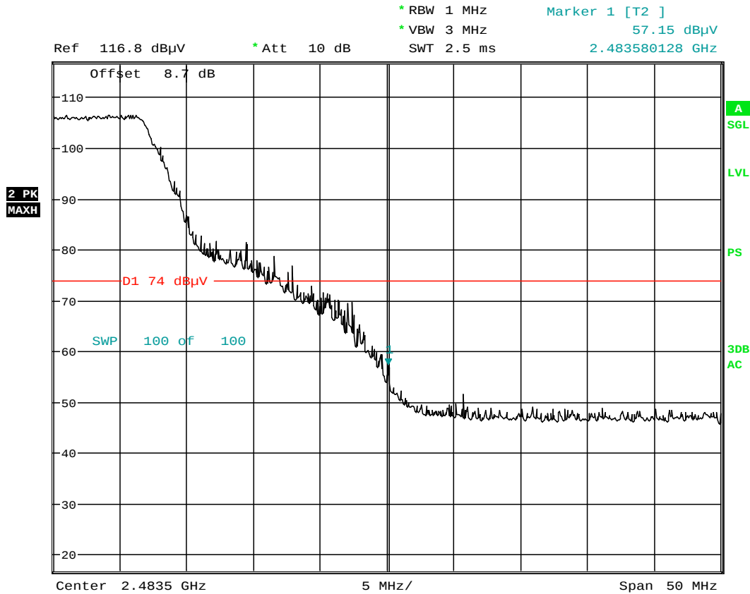
Plot 6-68. Radiated Restricted Upper Band Edge Measurement (Peak)
