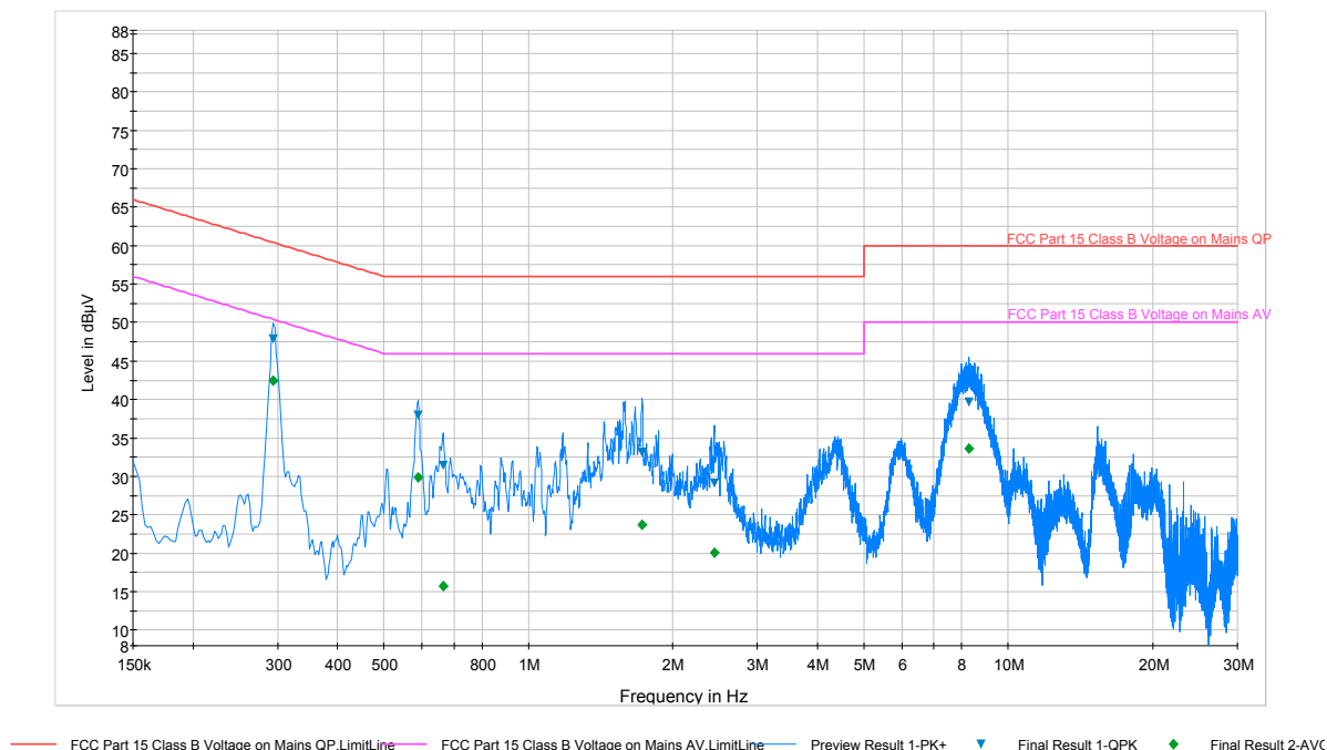
Plot 6-71. Line Conducted Plot with 802.11b (L1)
