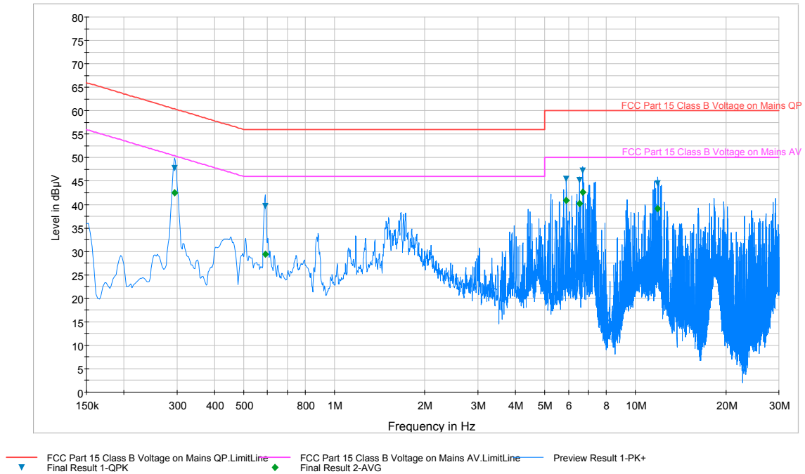
Plot 6-74. Line Conducted Plot with 802.11a (N)
