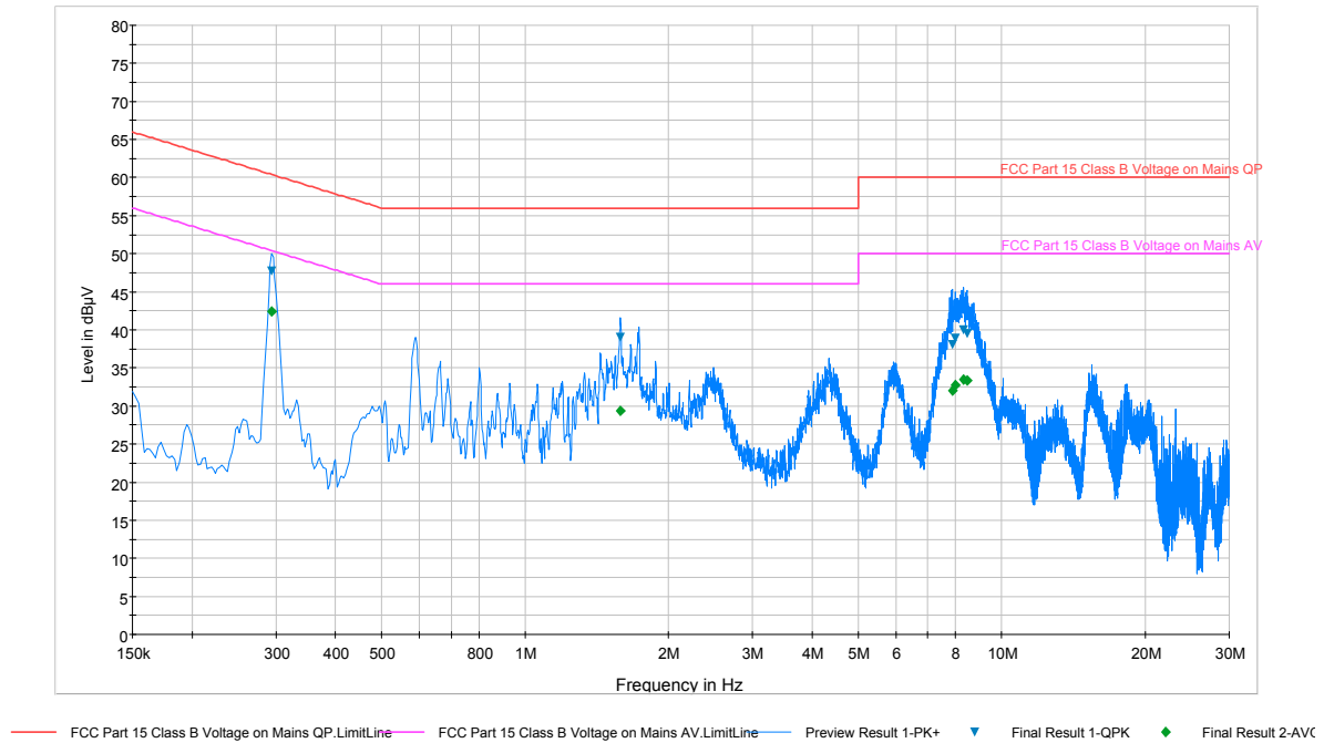
Plot 6-72. Line Conducted Plot with 802.11b (N)
