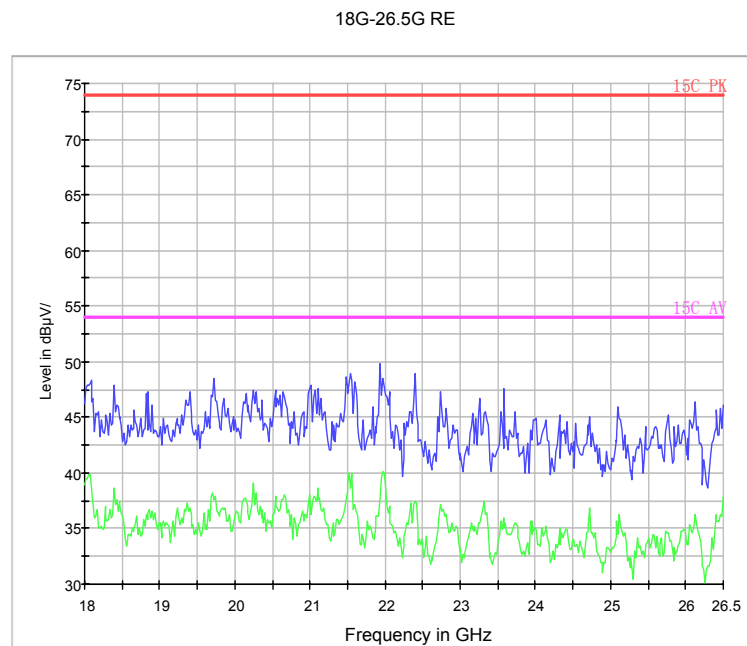
Fig.69. Radiated emission: GFSK, 18 GHz – 26.5 GHz
