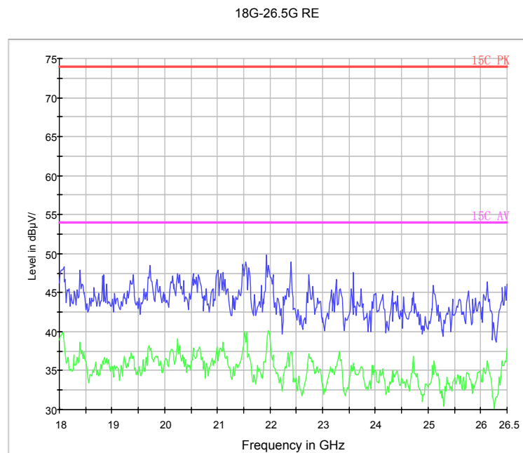
Fig.93. Radiated emission: 8DPSK, 18 GHz – 26.5 GHz
