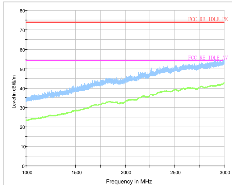
RE - 1GHz-3GHz
