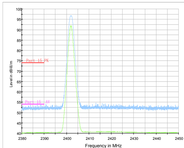
RE - Power-2.38GHz-2.45GHz
