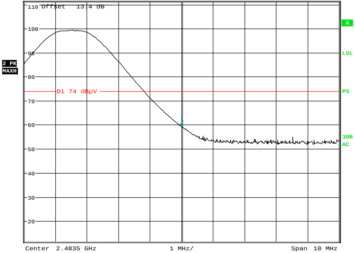
Plot 6-19. Radiated Restricted Band Edge Plot (Peak)
