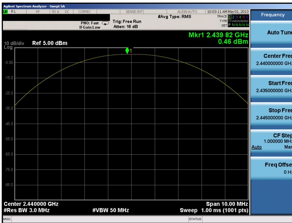
Plot 6-5. Peak Powery Plot (Bluetooth (LE) – Ch. 19)
