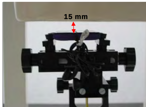
Fig.7 EUT front side with headset (MH410C) to flat phantom
