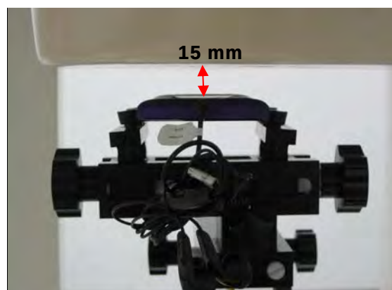
Fig.8 EUT back side with headset (MH410C) to flat phantom
