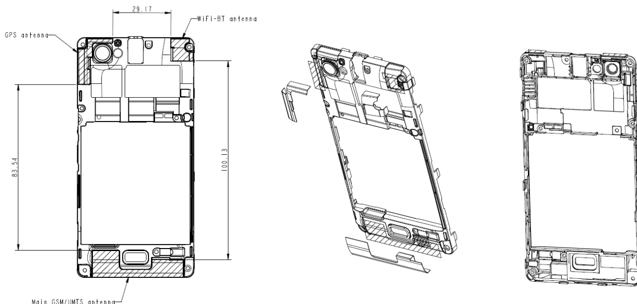
Fig.21 Antenna position of EUT
