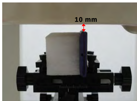
Fig.14 EUT right to flat phantom
