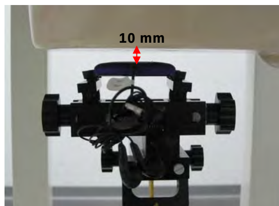
Fig.11 EUT back with headset (MH410C) to flat phantom
