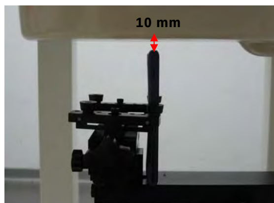
Fig.13 EUT top to flat phantom
