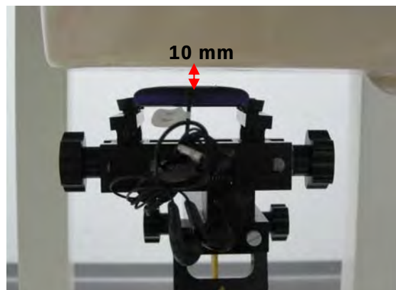
Fig.12 EUT back with headset (MH410C) to flat phantom
