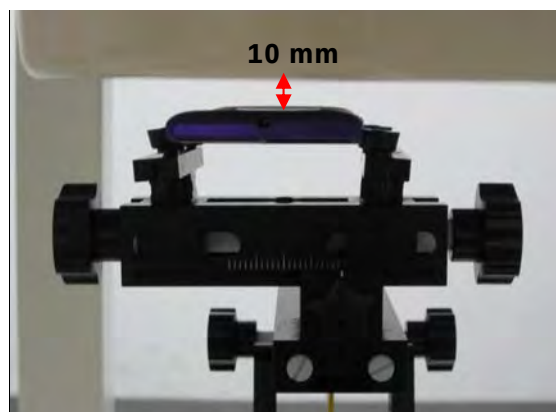
Fig.11 EUT back to flat phantom
