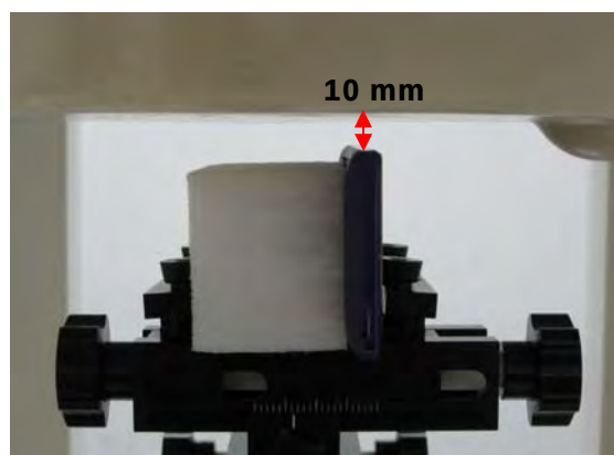
Fig.16 EUT left to flat phantom
