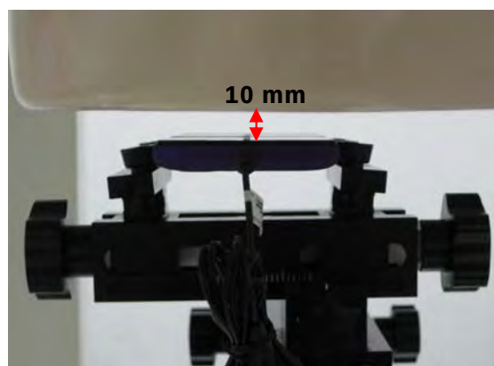
Fig.10 EUT front with headset (MH410C) to flat phantom
