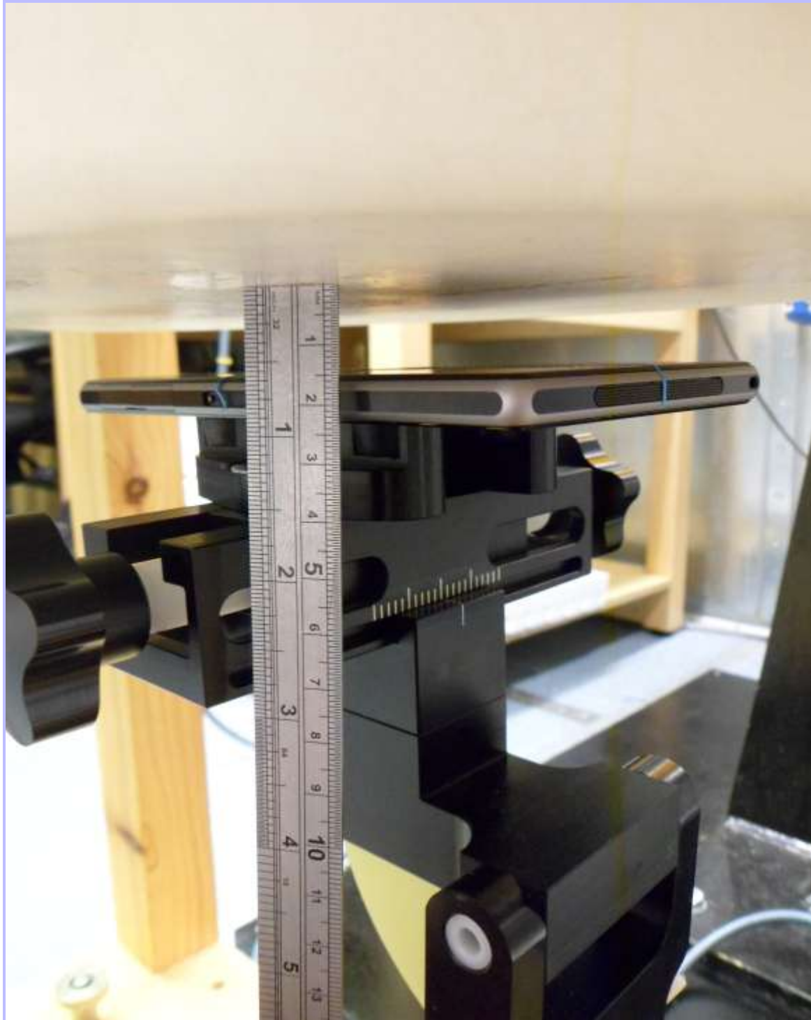
PHT/10014945JD13/007: Front of EUT Facing Phantom at 15mm Separation
