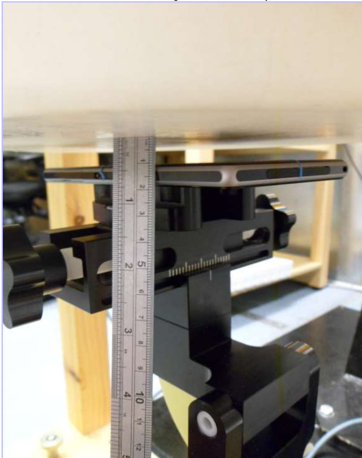
PHT/10014945JD13/006: Front of EUT Facing Phantom at 10mm Separation
