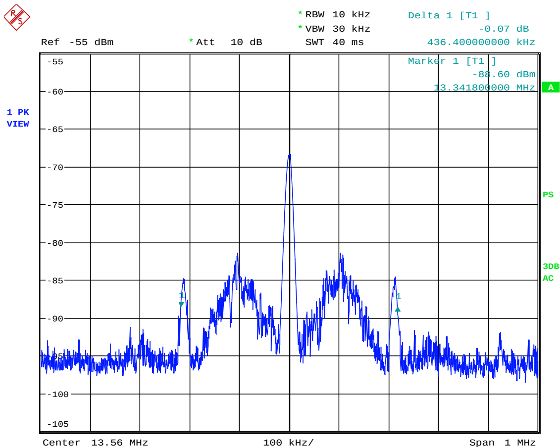
Figure 8-2. 20dB Bandwidth Plot
