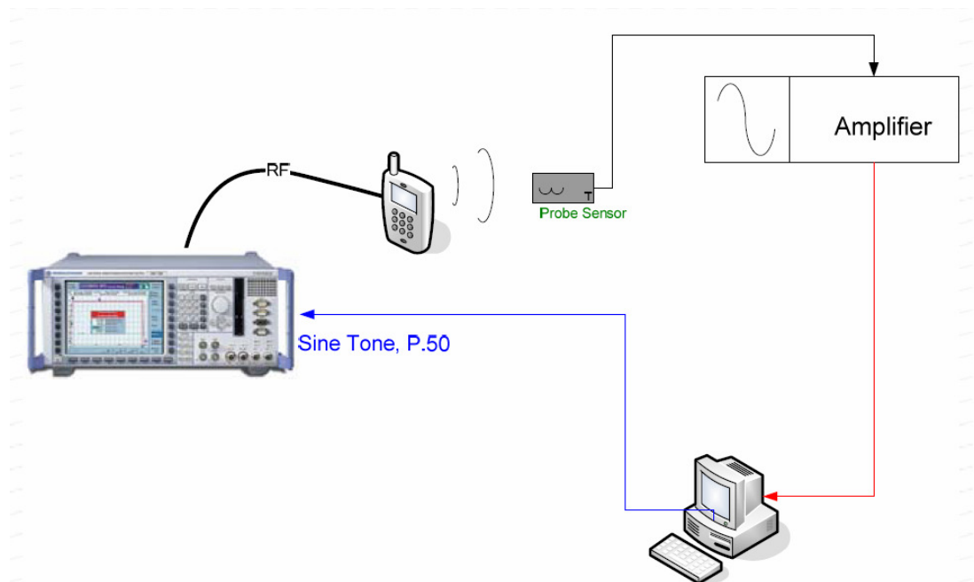
Figure 5-2 T-Coil Test Setup
