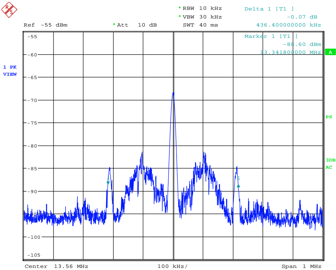
Figure 8-2. 20dB Bandwidth Plot
