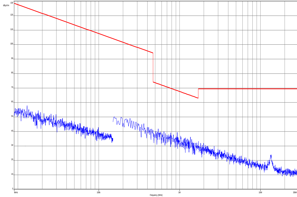
Plot 4: Channel 23790 (Traffic mode up to 30 MHz)
