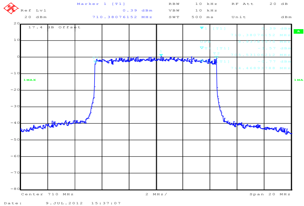
Plot 3: 10 MHz (99% - OBW)
