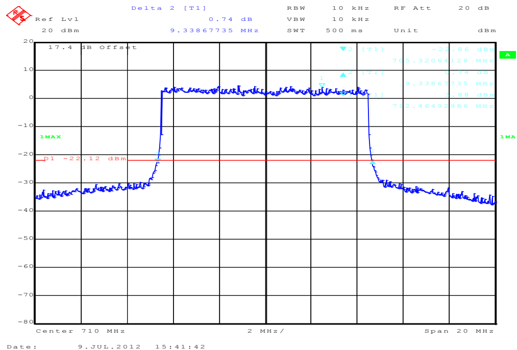
Plot 4: 10 MHz (-26 dBc BW)
