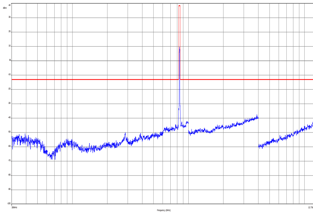
Plot 4: Channel 20525 (30 MHz – 12.75 GHz)
