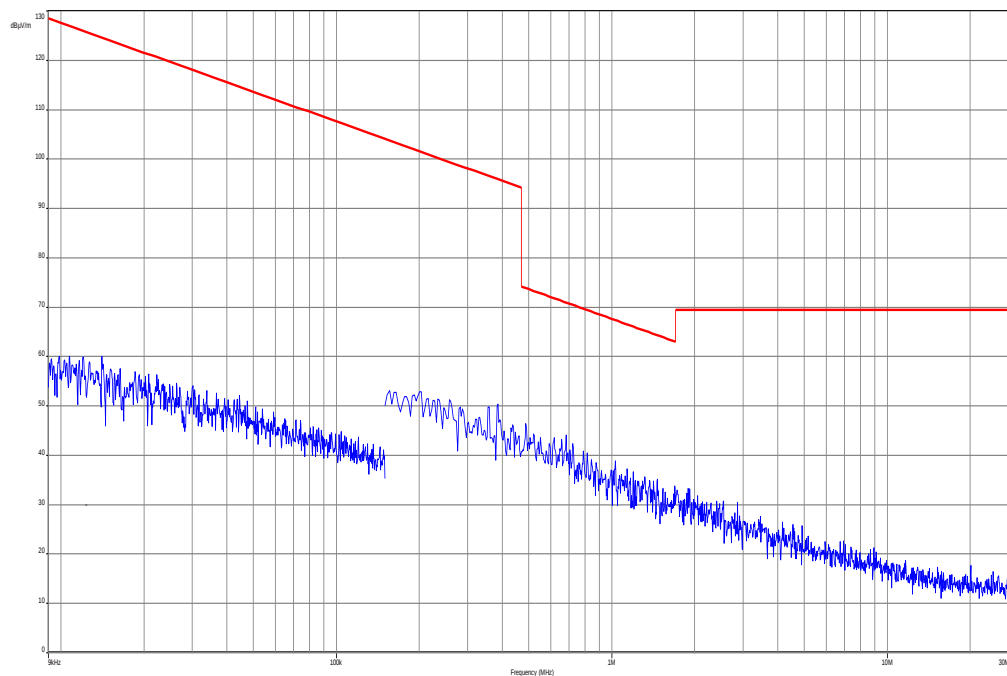
Plot 3: Channel 20525 (Traffic mode up to 30 MHz)
